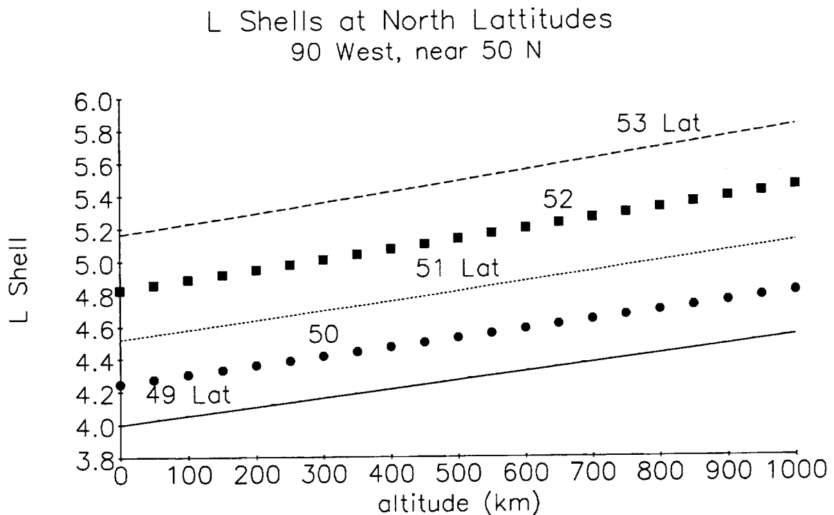
Figure 4. Relationship of L shell with altitude for several Latitudes at 90^\circ\text{W} longitude, from IGRF91.
