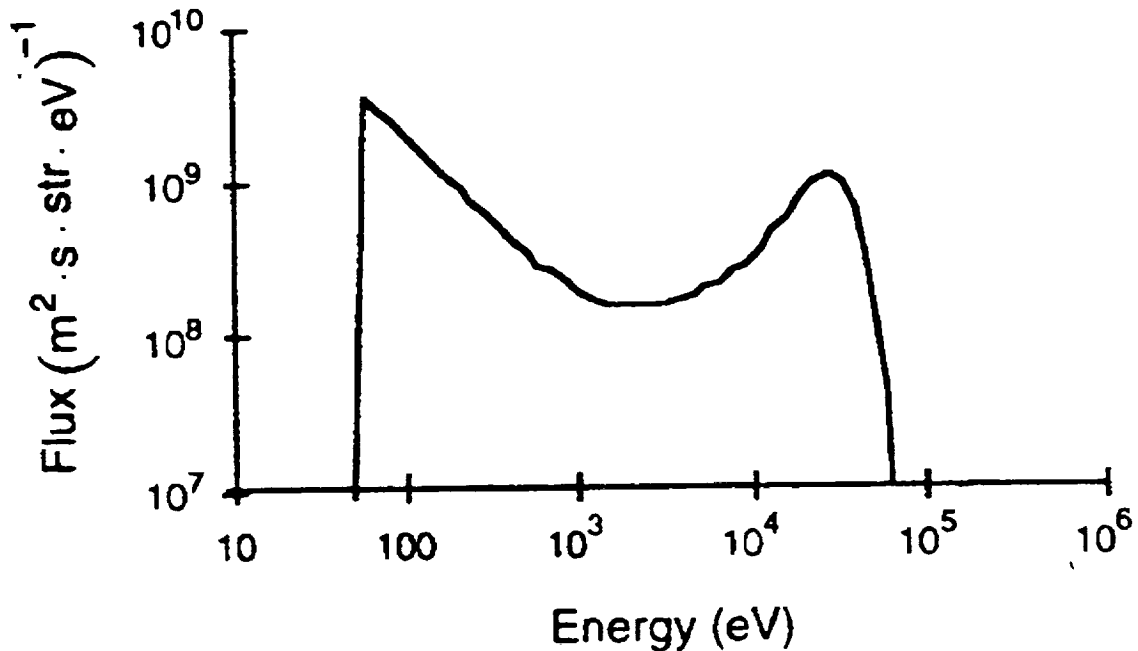
Figure 6. A severe charging environment. Fontheim distribution for A_p [Power law coefficient] = 3 \times 10^{11} \text{ m}^{-3} , \alpha = 1.1 , E_{PL} = 50 \text{ eV} , E_{PH} = 1.6 \times 10^6 \text{ eV} , n = 6 \times 10^5 \text{ m}^{-3} , \Theta = 8 \text{ KeV} , A_G = 4 \times 10^4 \text{ m}^{-3} , E_0 = 24 \text{ KeV} , \delta = 16 \text{ KeV} , from ref. 8.
