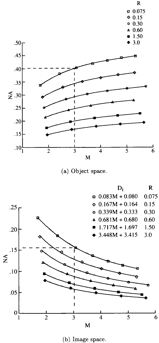
Figure 3. Dependence of NA on ball lens M of laser diode with defocus to balance SA and provide 0.25\lambda -OPD wave front. Coupling efficiency = 0.56; \lambda = 0.85\ \mu\text{m} ; n = 1.76 .
