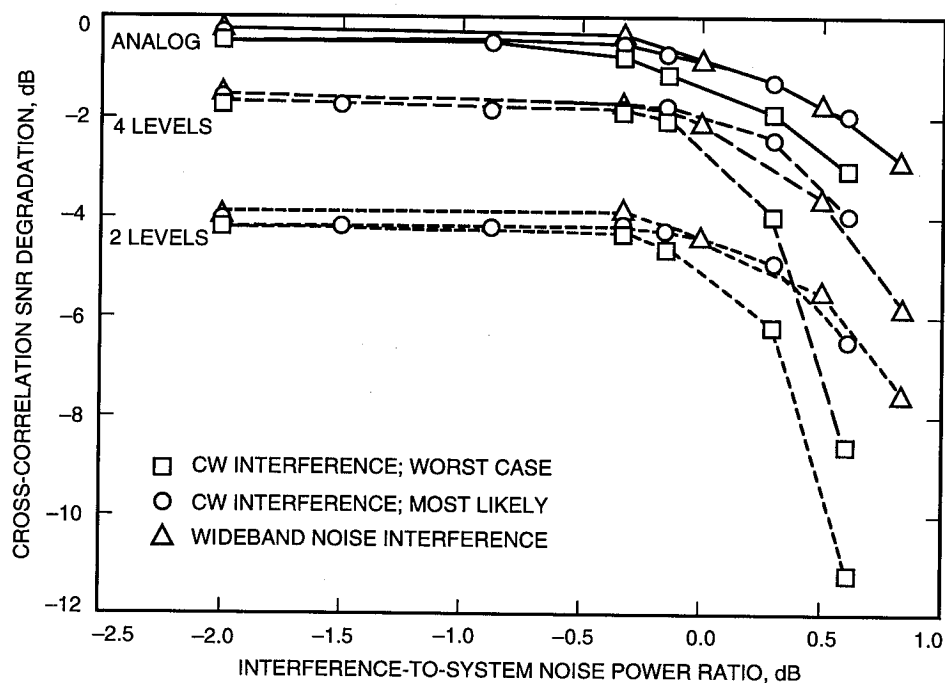
Fig. 3. Cross-correlation SNR degradation as a function of interference-to-system noise power ratio.
