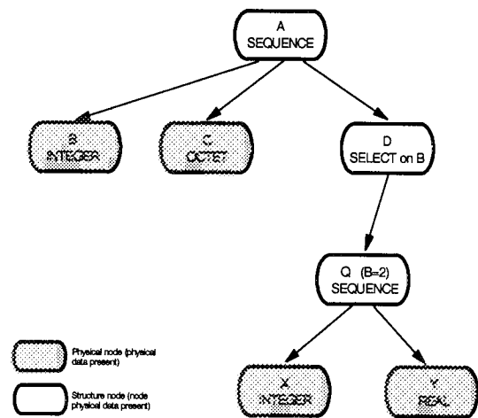
Figure 4: Schematic of the Value Tree Generated
