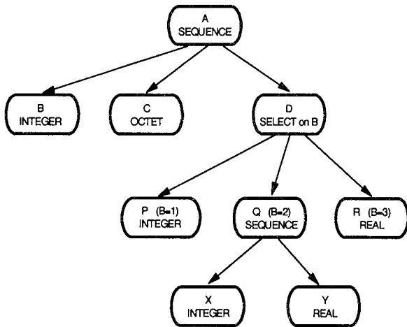
Figure 3: Schematic of the Syntax Tree Generated
