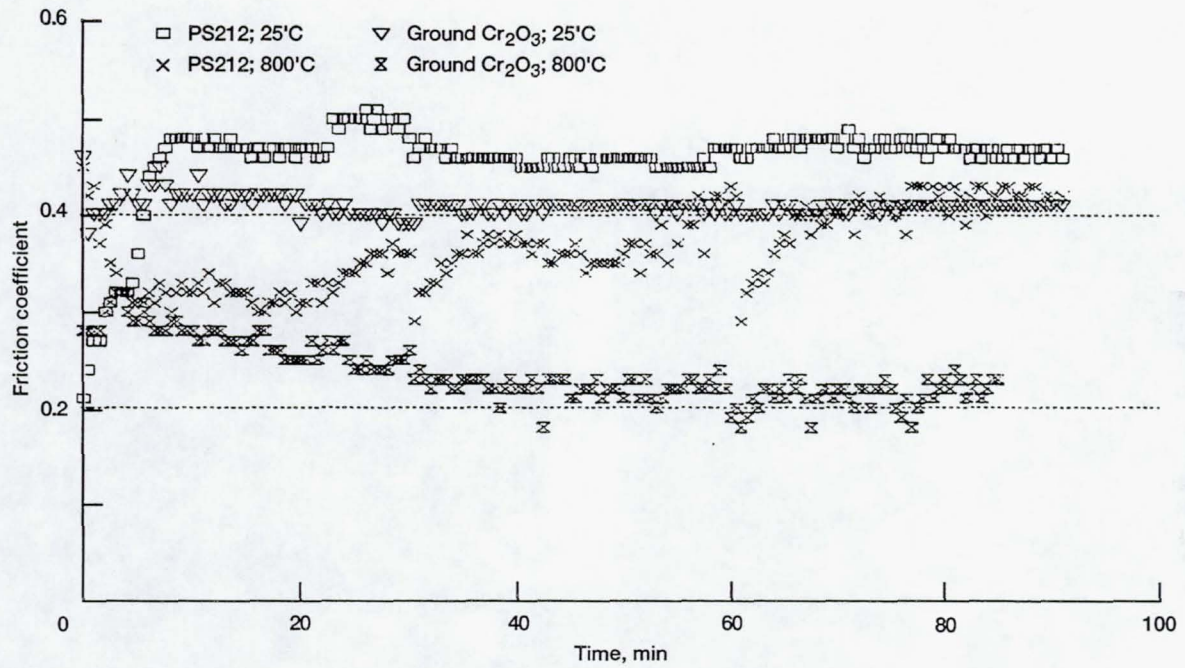
Figure 7.—Friction-time trends.
