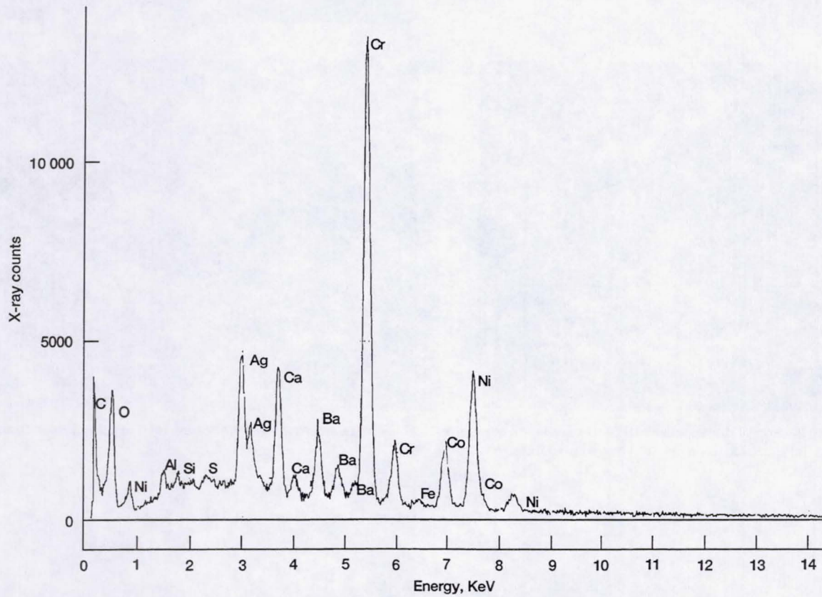
Figure 4.—SEM photomicrograph and EDS spectrum of Cr 2 O 3 seal coating/PS212 interfacial region.
