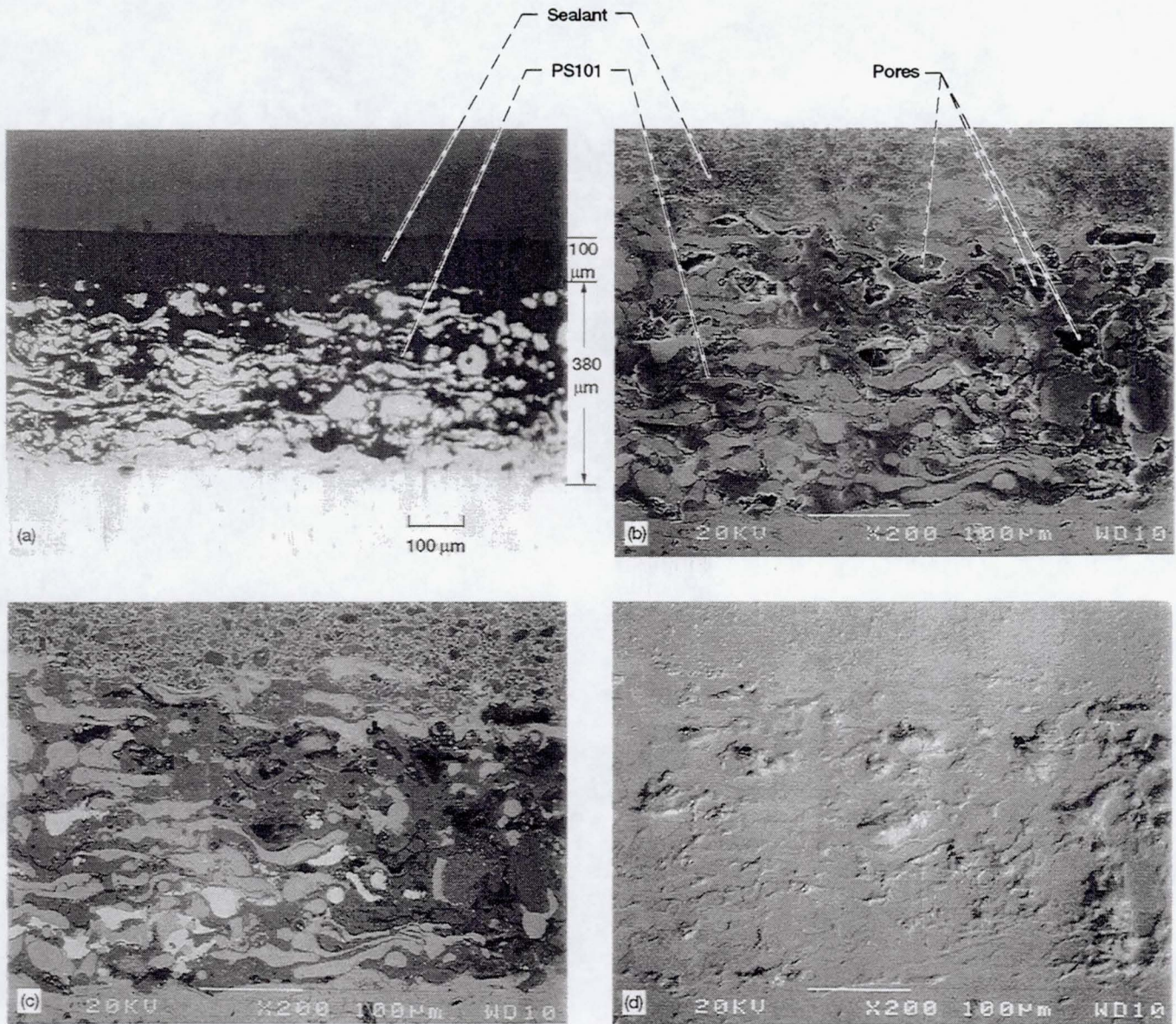
Figure 5.—Cross section of duplex sealant/PS101 coating on Inconel X-750 by various microscopy techniques. (a) Optical. (b) Secondary electron SEM. (c) Back scatter SEM. (d) Topographic SEM.
