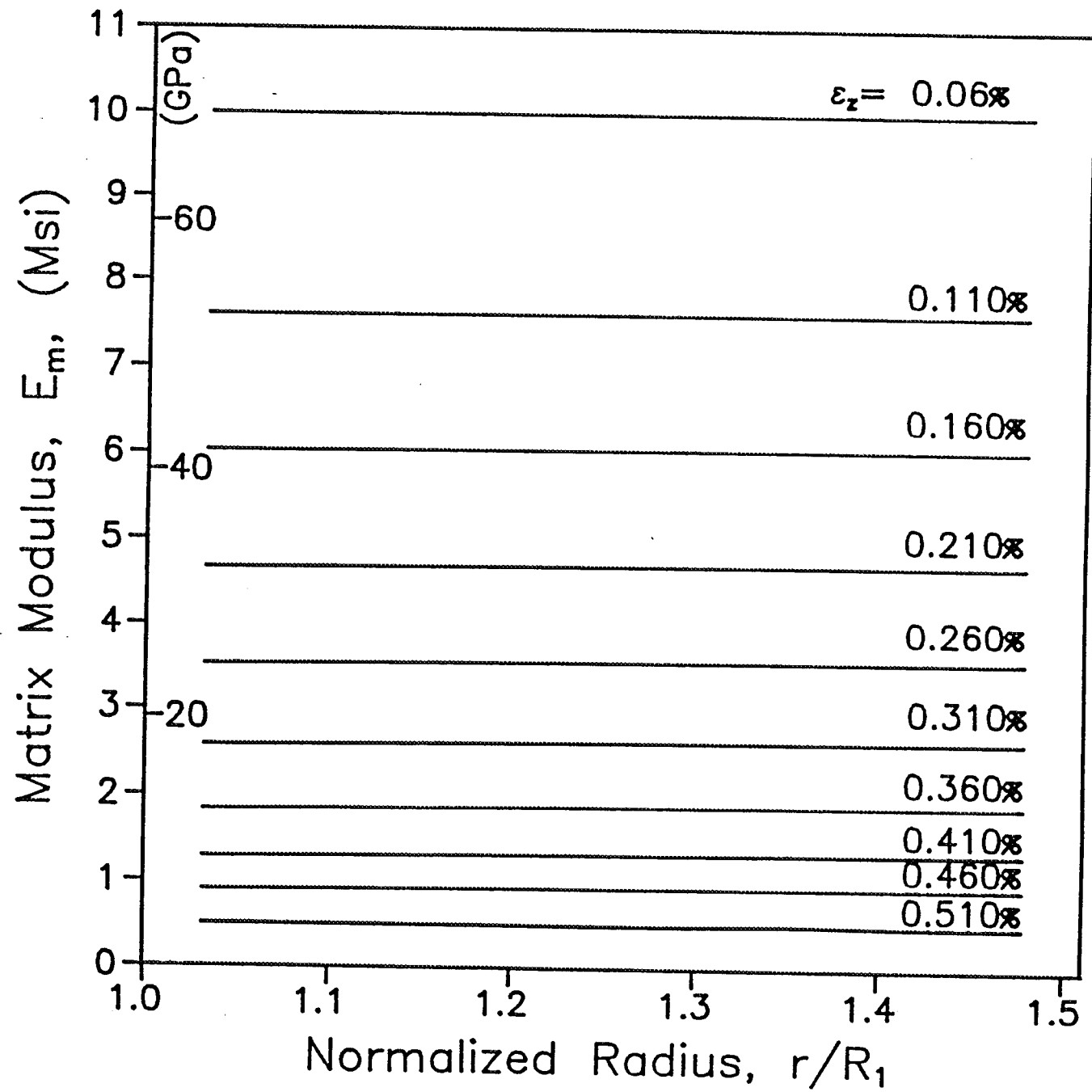
Fig. 5 Variation of Tangent Modulus Along the Thickness of the Aluminum Matrix Shell in the CCM for Different Values of the Applied Strain \epsilon_z at T = 2000^\circ\text{C} (3550 ^\circ\text{F} )
