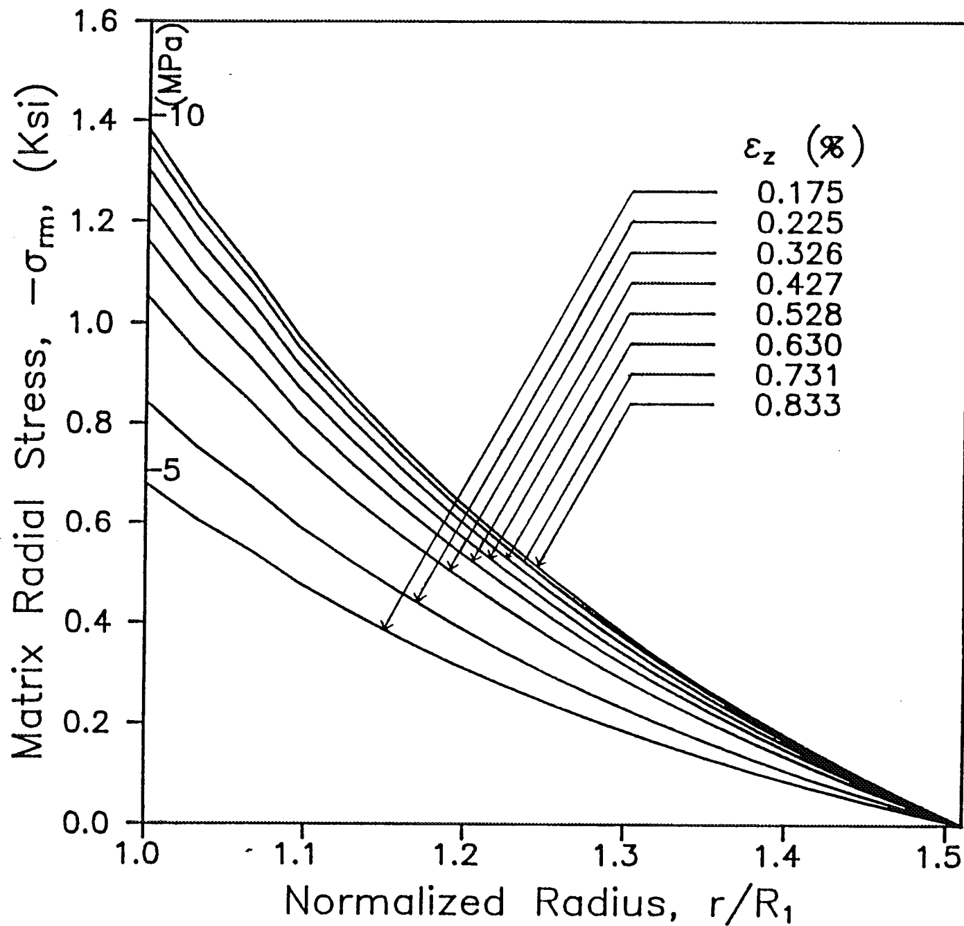
Fig. 9. Variation of the Radial Stress \sigma_m Along the Thickness of Aluminum Matrix Shell in the CCM for Different Values of the Applied Strain \epsilon_z at T = 24^\circ\text{C} ( 75^\circ\text{F} ).
