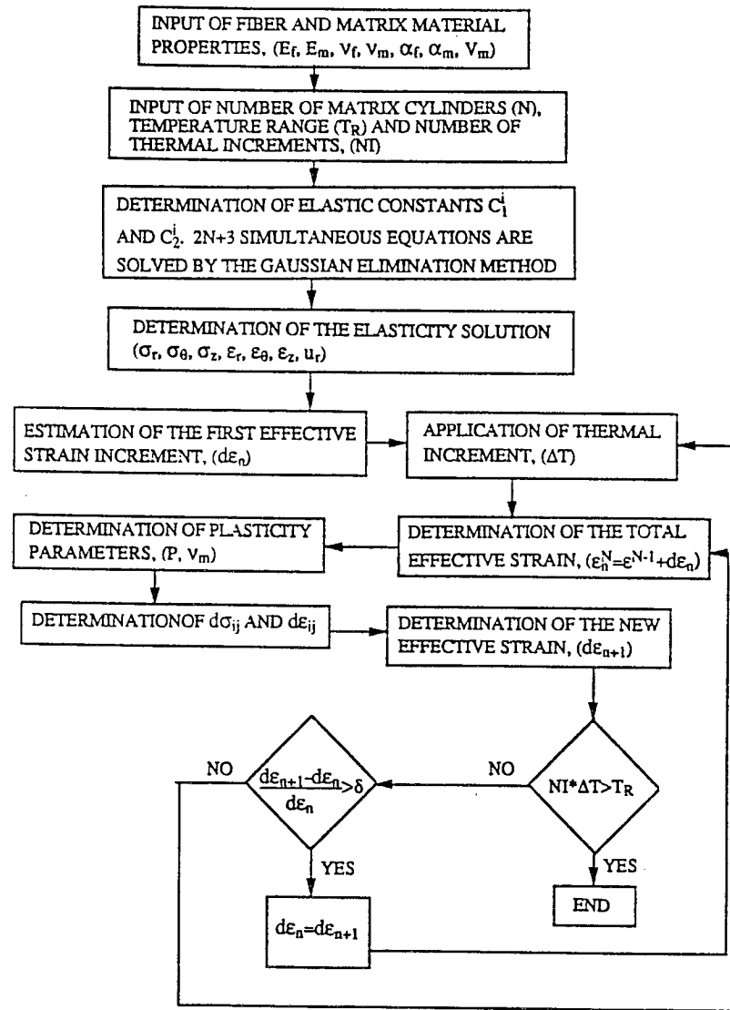
Fig. 7.2 Flow Chart of the Composite Cylinder Thermal Loading Program.
