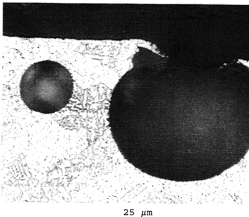
Figure 4. - Internal and external blistering in a 2195 alloy weld bead caused by air contamination.
