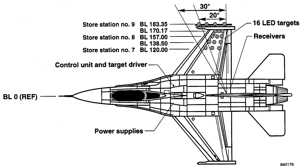
Fig. 3 FDMS installation.
