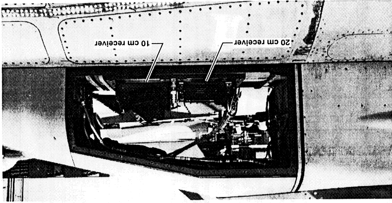
Fig. 5 Receiver bay.
