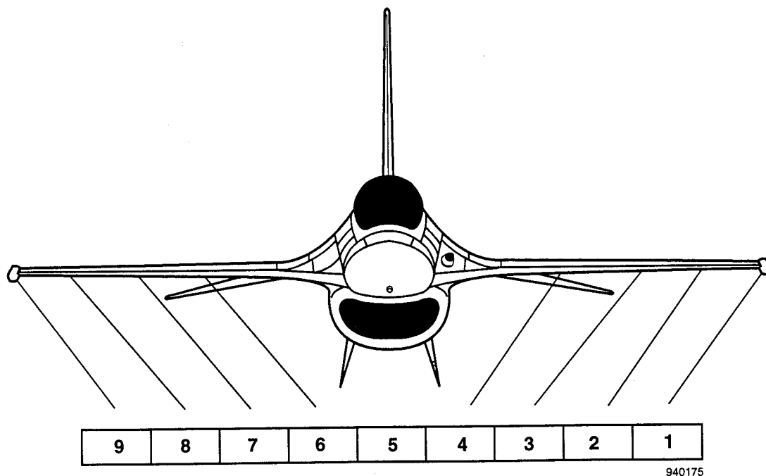
Fig. 1 F-16 external store stations.
