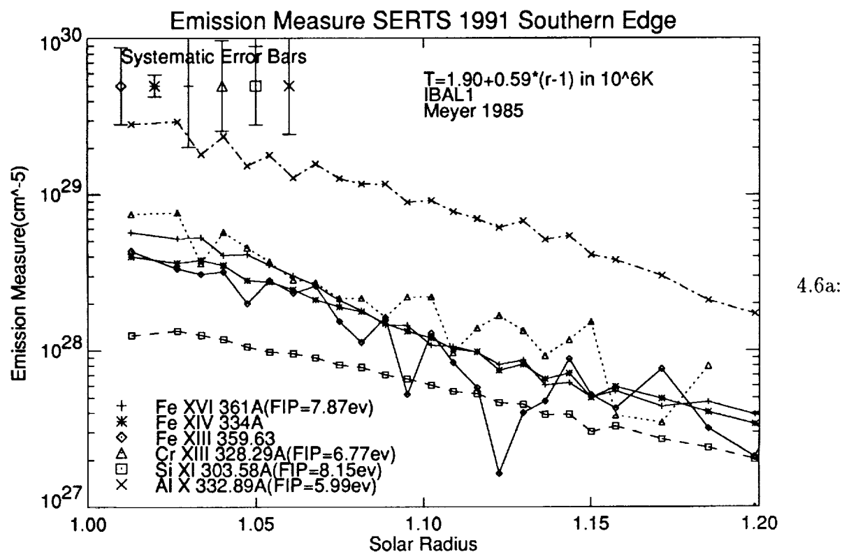
Figure 4.6. The emission measures plotted as a function of radius are shown for SERTS 1991 southern edge (4.6a), SERTS 1989 southern edge (4.6b), and SERTS 1991 northern edge (4.6c). This plot uses the line-ratio temperature determined from Figure 4.4 using IBAL1. The systematic error bars for each emission measure are shown in the upper left hand corner with a symbol in the center corresponding to the appropriate emission line. In Figure 4.6, the emission measure for Fe XVI is larger than for the other iron lines due to the hot loop. The dips in the Fe XIII emission measure near 1.09 and 1.12R_{\odot} are probably due to the uncertainties in the background subtraction.
