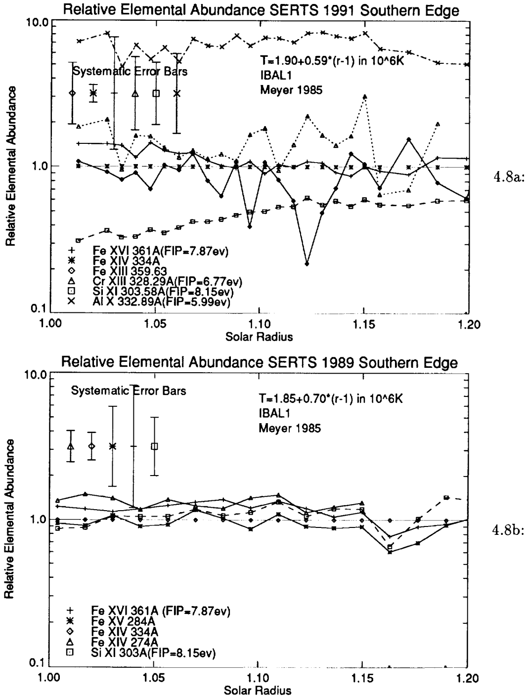
Figure 4.8. Plots of the relative elemental abundance for SERTS 1991 southern edge (4.8a), and SERTS 1989 southern edge (4.8b) using IBAL1. These plots used the emission measures determined earlier divided by the emission measure of the Fe XIV line for Figure 4.8a and the Fe XV for Figure 4.8b. The systematic error bars are shown in the upper left hand corner.
