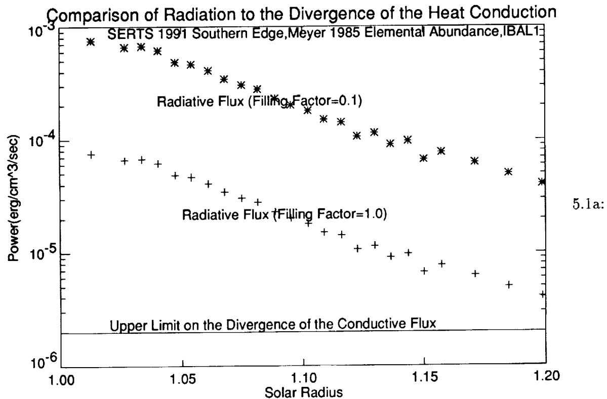
Figure 5.1. Heating Constraints
