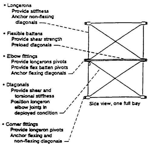
Figure 2 - FASTMast Structure
