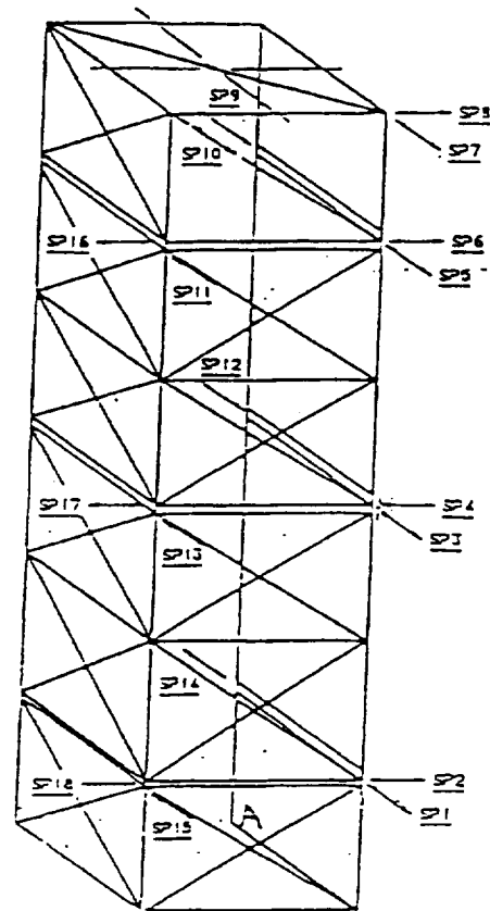
Figure 15 - Displacement Transducer Locations for Tip Shear Test
