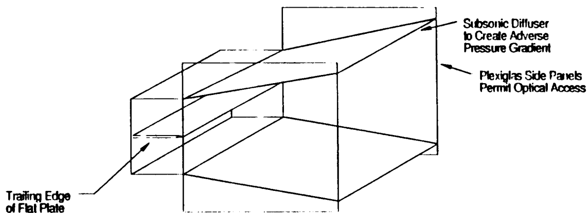
Figure 2. Diffuser Used to Create Adverse Pressure Gradient.
