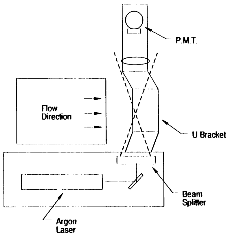
Figure 4. Top View of Forward Scatter L. D. V. System.
