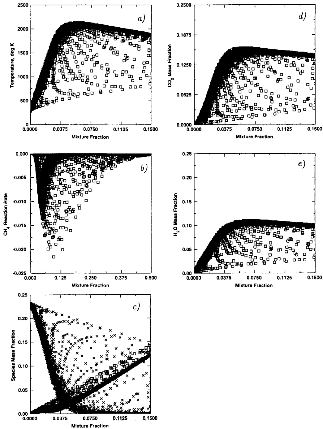
FIGURE 5. Scatter plots at 1.0 eddy turn time for one-step mechanism: a) temperature, b) \text{CH}_4 reaction rate, c) \text{CH}_4 and \text{O}_2 mass fraction ( \square \text{CH}_4 , \times \text{O}_2 ), d) \text{CO}_2 mass fraction, and e) \text{H}_2\text{O} mass fraction.
