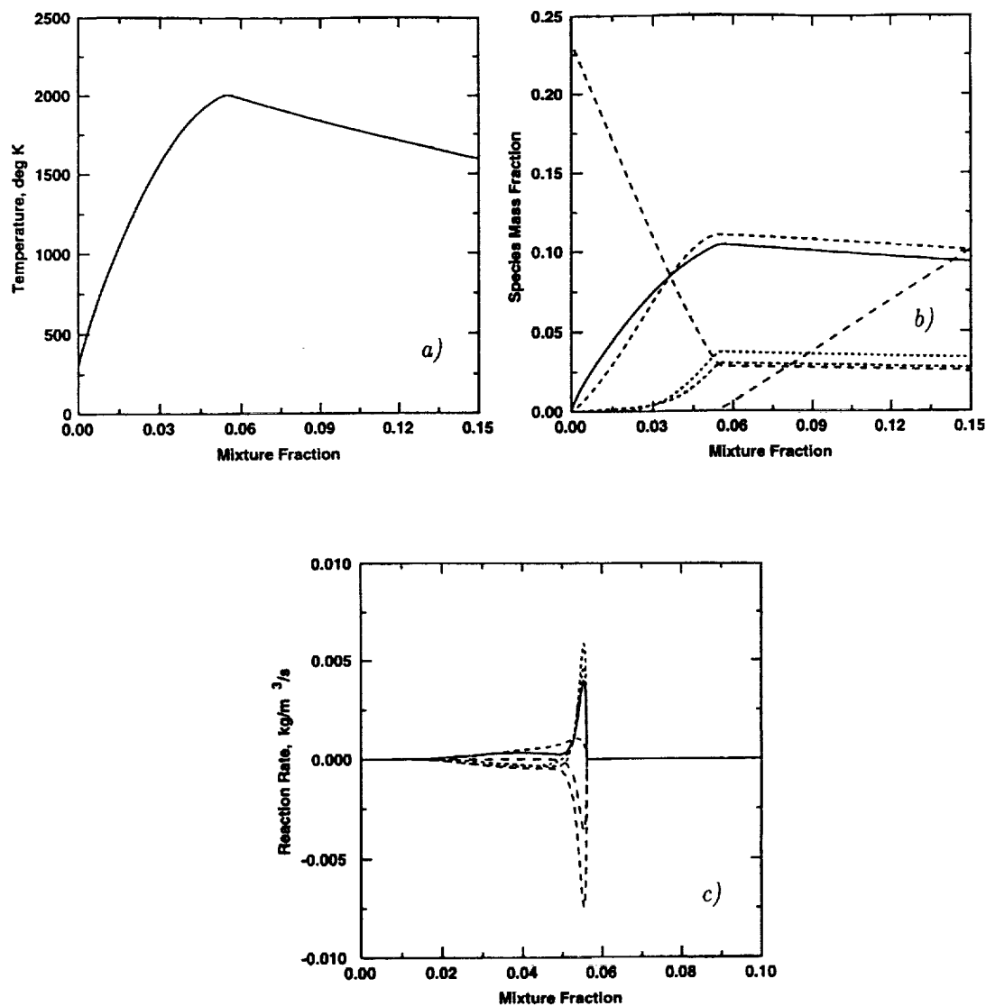
FIGURE 2. One-dimensional strained laminar flame for methane-air three-step mechanism: a) temperature, b) species mass fractions, c) species reaction rates. (— H_2O , ..... H_2 \times 40 , ..... CO , ---- CO_2 , ---- O_2 , ---- CH_4 ).
