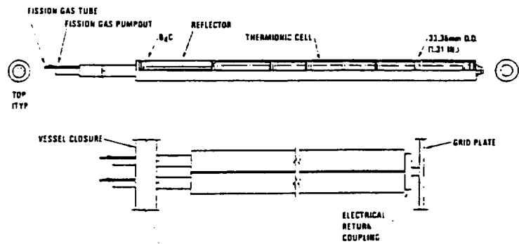
Figure F-1. Driver Fuel In-Core TFE system concept.
