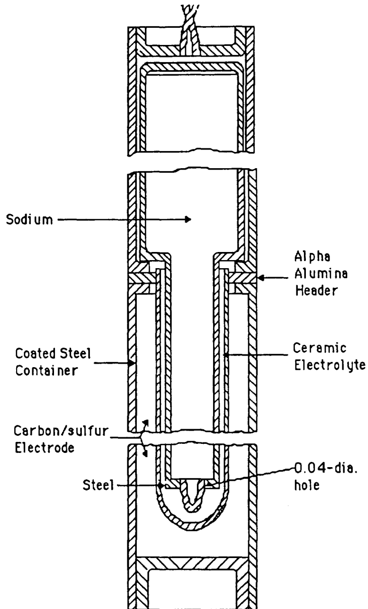
Figure C-3. Typical tubular NaS battery cell design.
