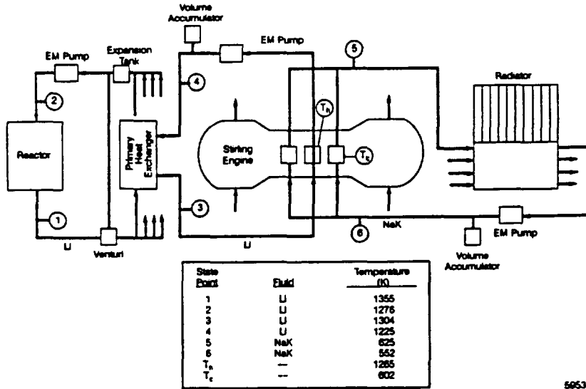
Figure H-1. 550 kW Brayton cycle power system schematic.
