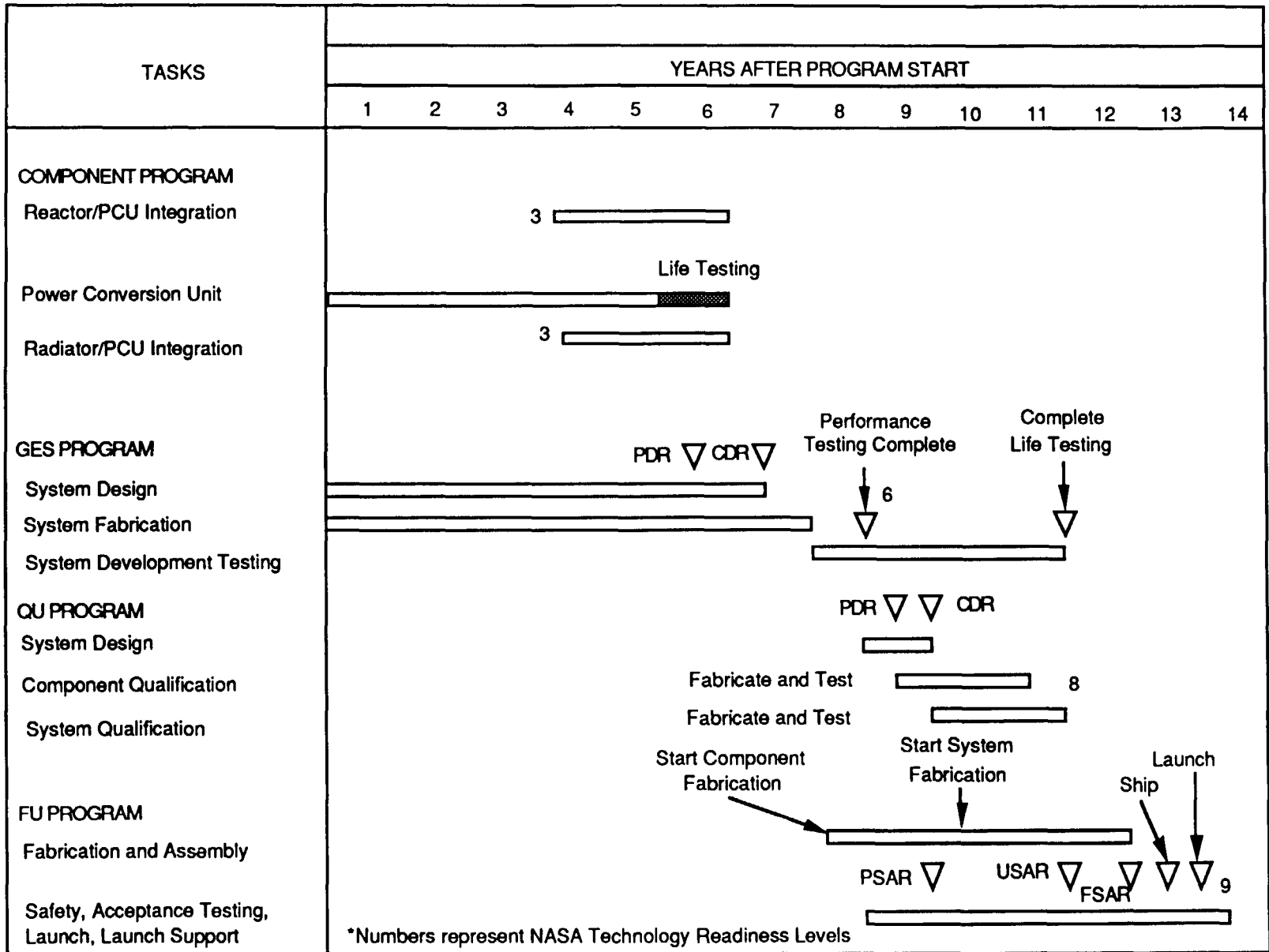
Figure H-9. PRC dynamic SP-100 development schedule.
