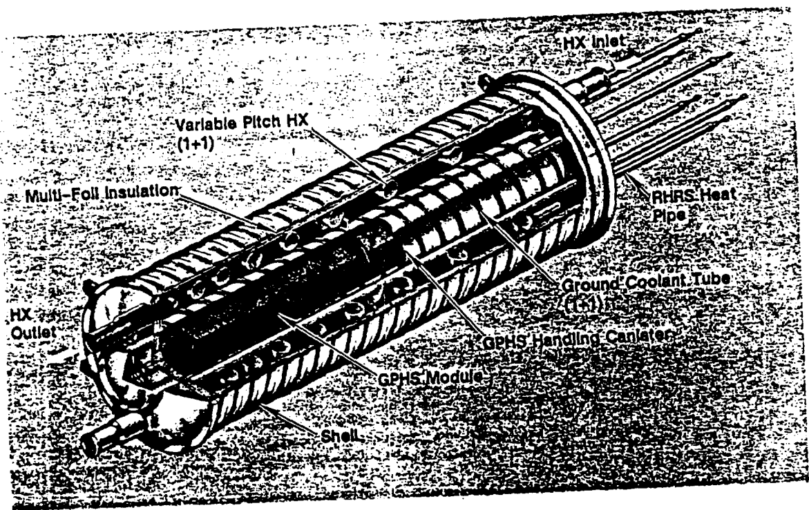
Figure A-3. 2.5 kWe DIPS HSU.
