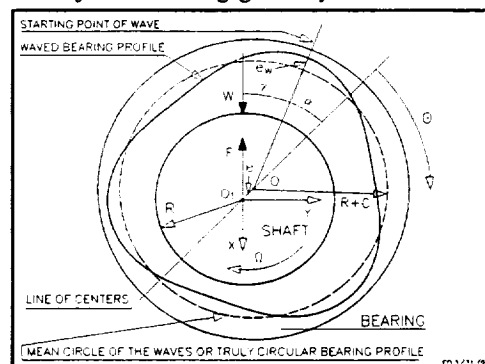
FIGURE 1. WAVE AND PLAIN JOURNAL BEARING GEOMETRY
