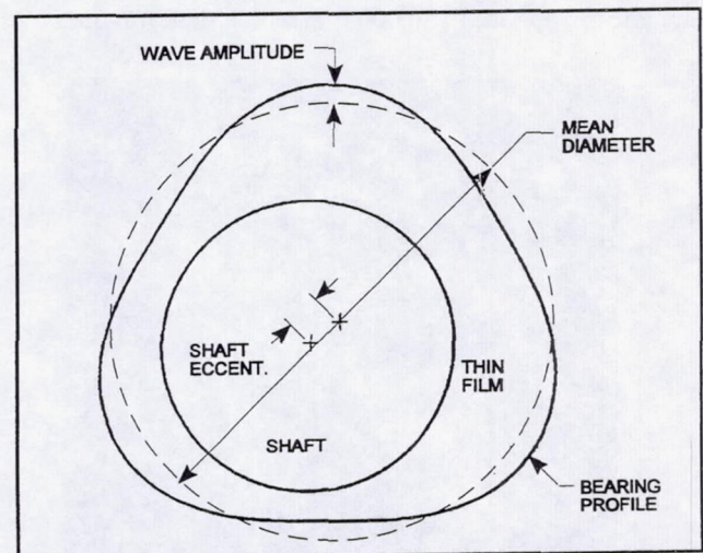
FIGURE 1. THREE-WAVE JOURNAL BEARING (WAVE AMPLITUDE AND CLEARANCE GREATLY EXAGGERATED)
