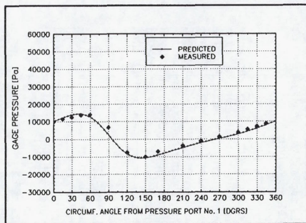
b. 10,160 RPM, RADIAL LOAD = 33 N, RADIAL CLEARANCE = 38 MICRONS
