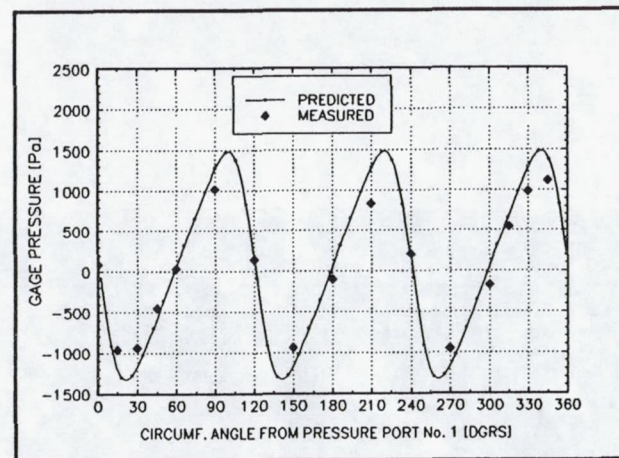
d. 2,500 RPM, RADIAL CLEARANCE = 39 MICRONS AND WAVE AMPLITUDE RATIO = .33 AT BEARING TEMPERATURE = 28 C
