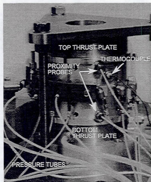
FIGURE 3. BEARING ASSEMBLY
