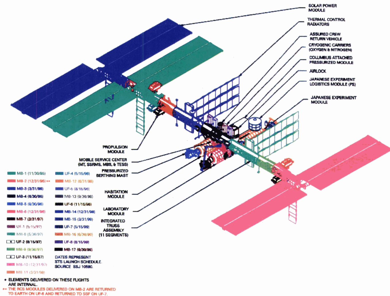
Figure 4.—Assembly sequence overview of the Space Station (figure courtesy of Boeing).
