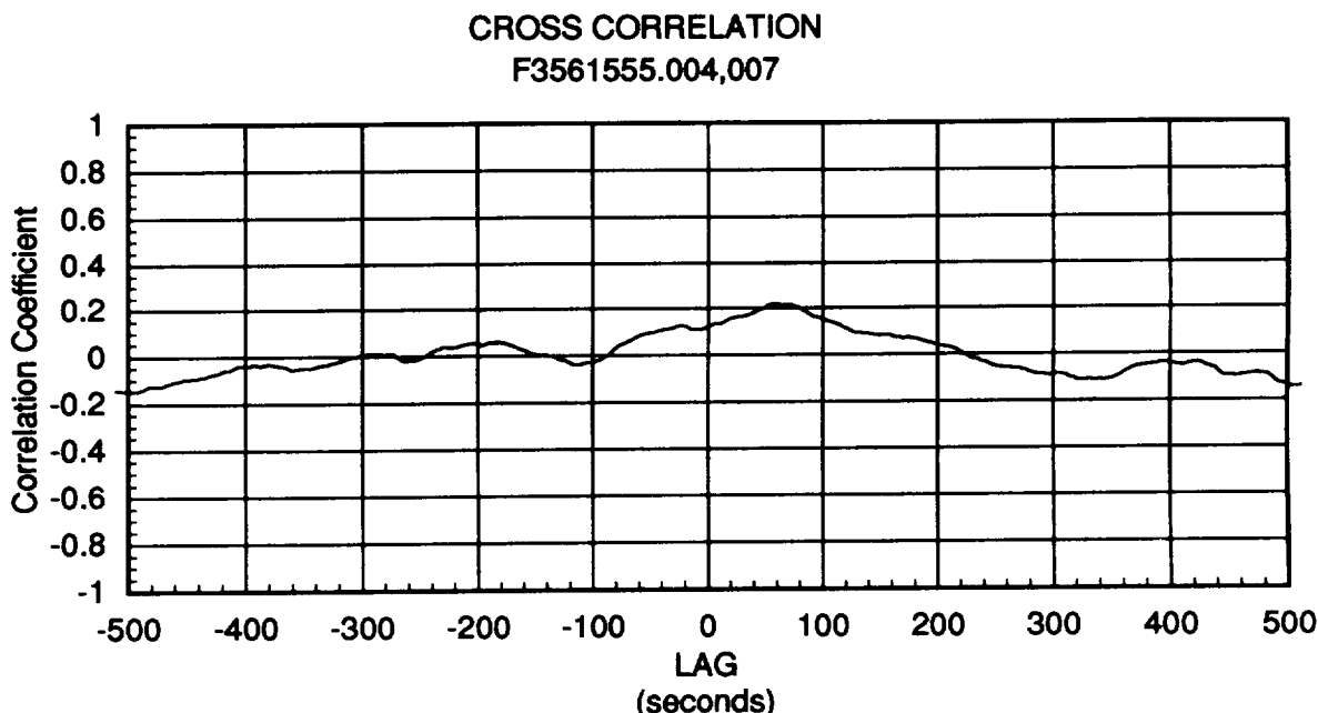
Figure 16. One Second Lagged WS Correlation, Files F3561555.004, 7
