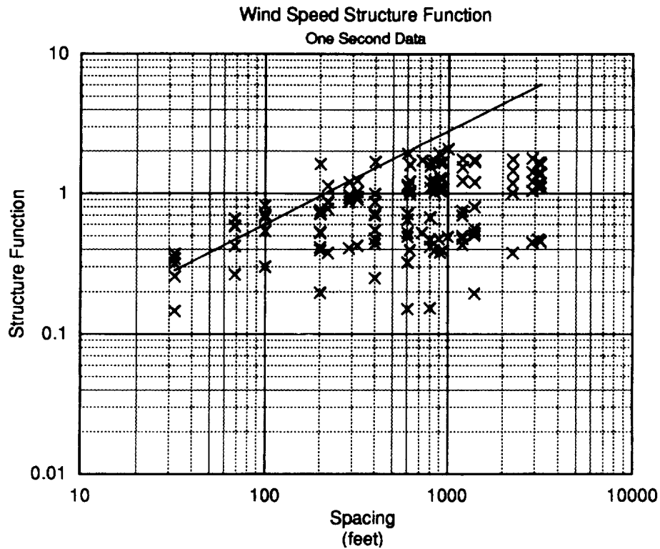
Figure 18. One Second WS Structure Function
