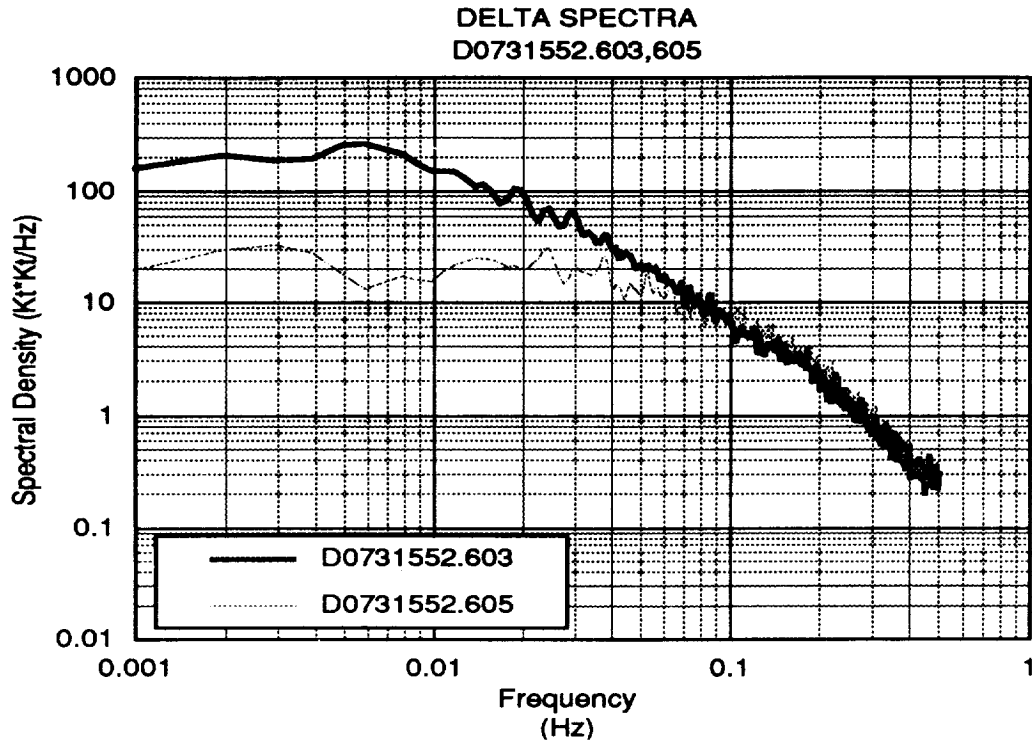
Figure 28. Speed Difference Spectrum
