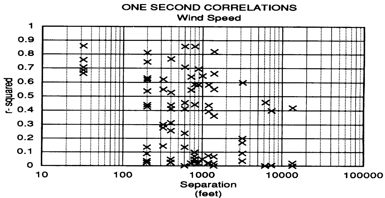
Figure 12. One Second Wind Speed Correlation at Zero Lag
