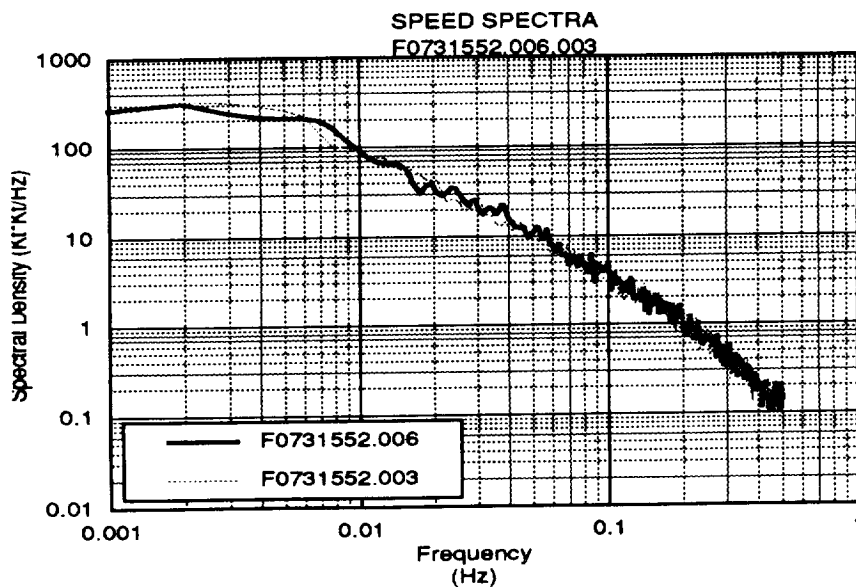
Figure 23. Typical Wind Speed Spectrum
