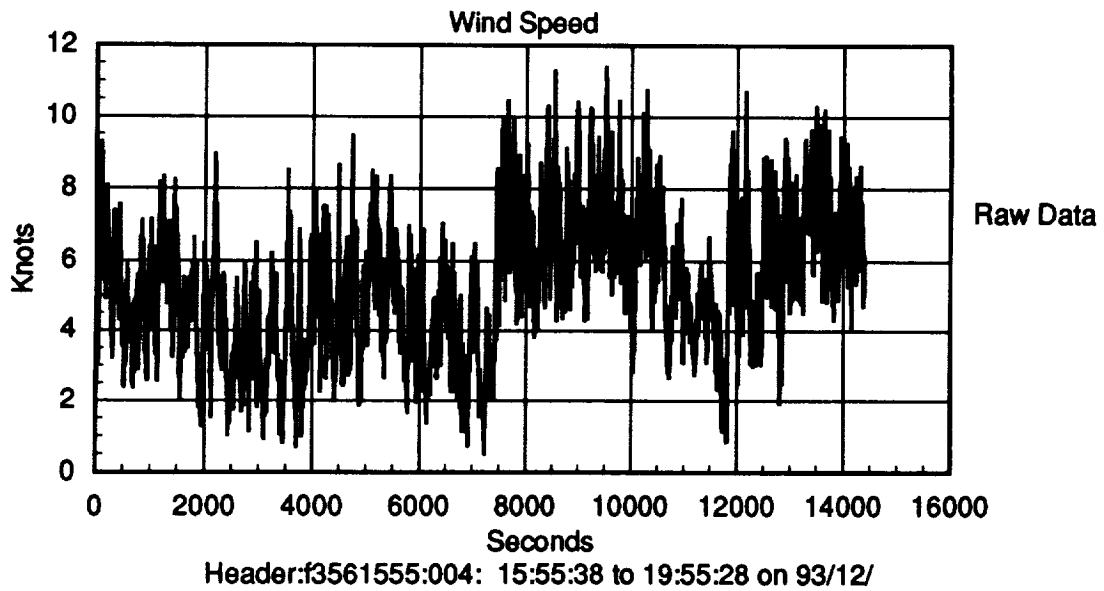
Figure 17b. Time Series, File F3561555.004
