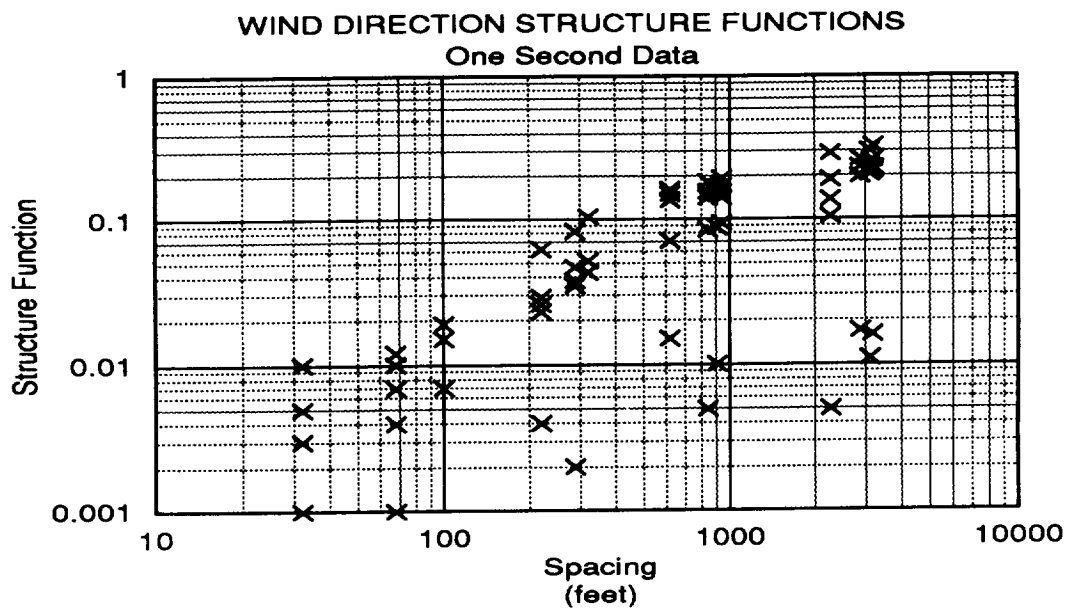
Figure 22. Five Minute WD Structure Function
