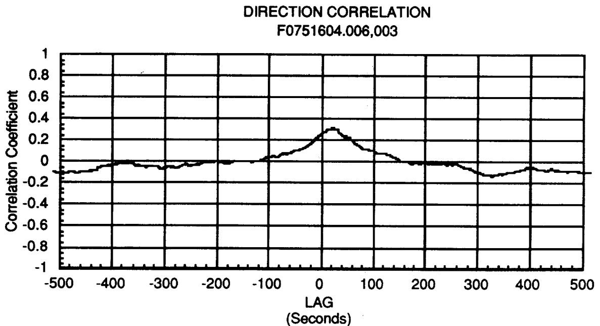
Figure 6. Wind Direction Correlation
