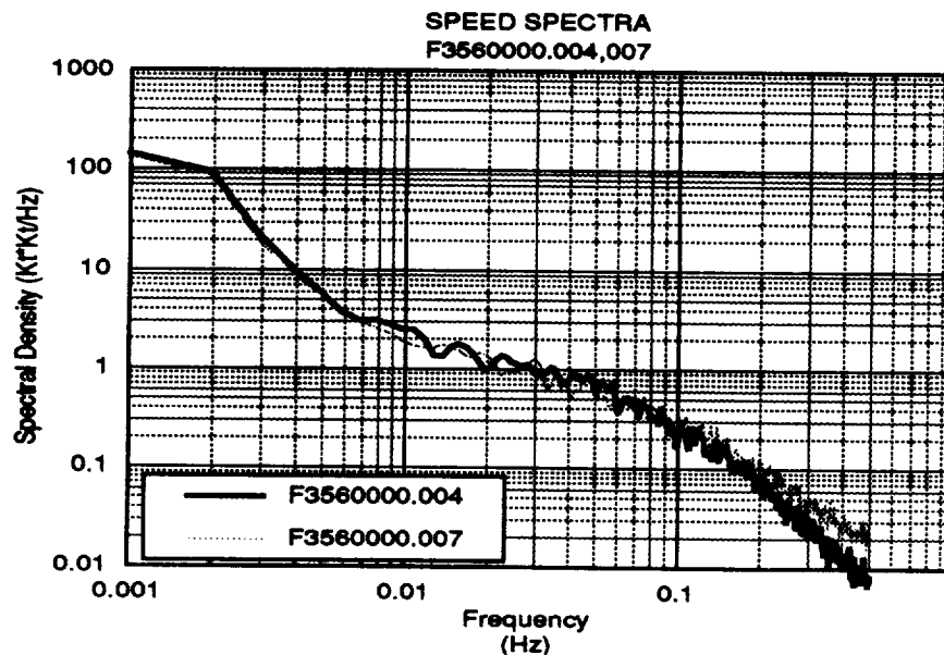
Figure 24. Atypical Wind Speed Spectrum
