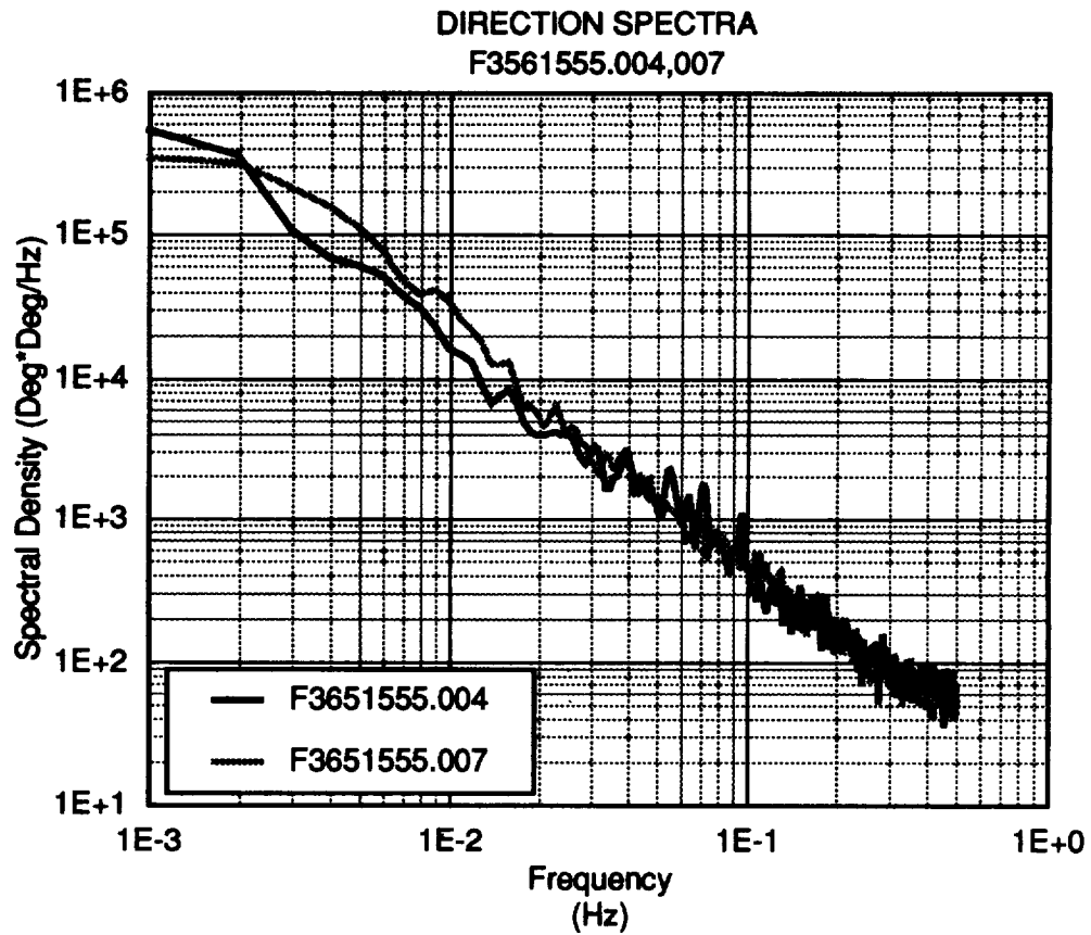
Figure 8. Wind Direction Spectra
