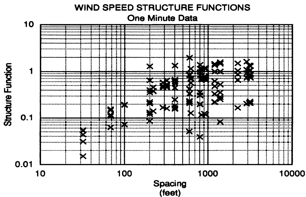
Figure 20. One Minute WS Structure Function
