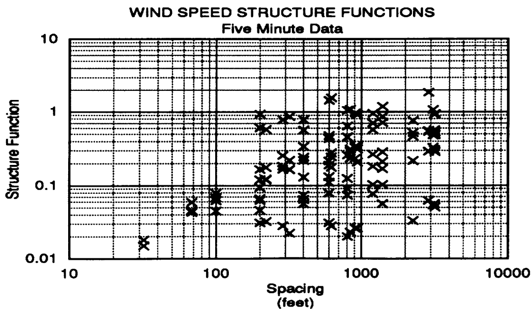
Figure 21. Five Minute WS Structure Function
