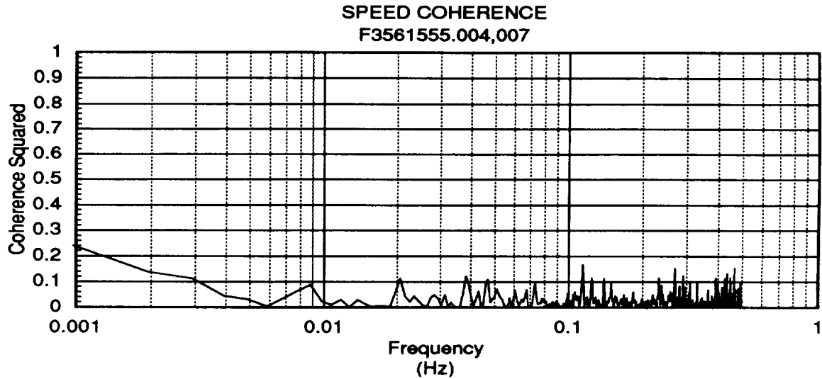
Figure 26. Coherence Spectrum, 800', No Trends
