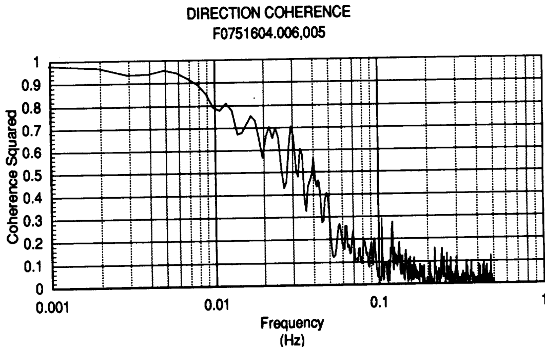
Figure 10. Wind Direction Coherence
