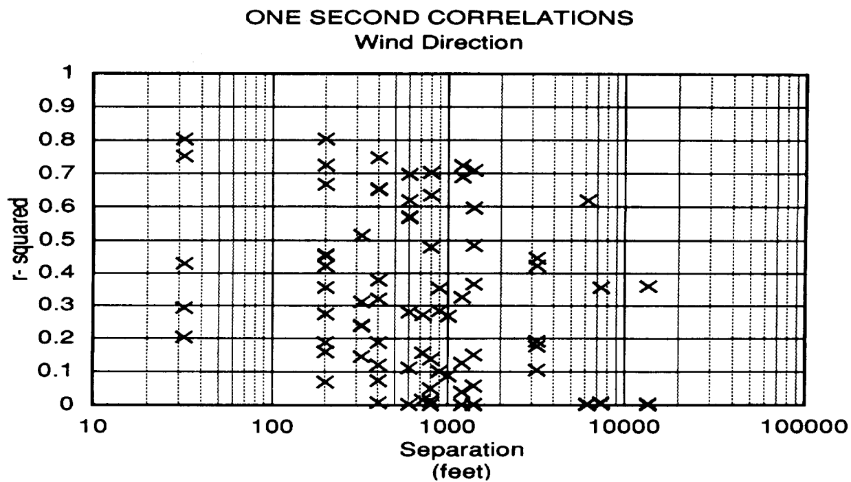
Figure 13. One Second Direction Correlation at Zero Lag
