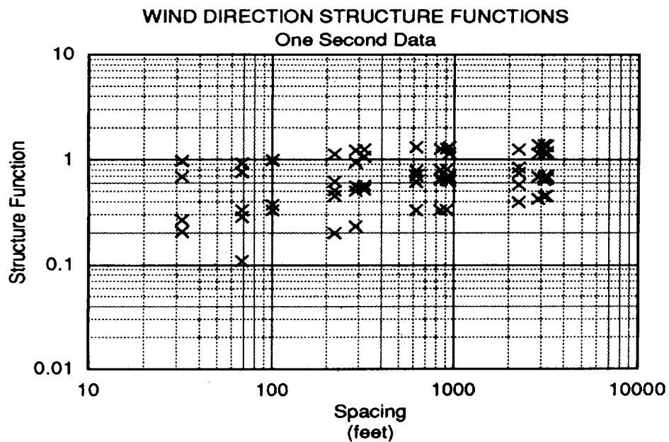
Figure 19. One Second WD Structure Function
