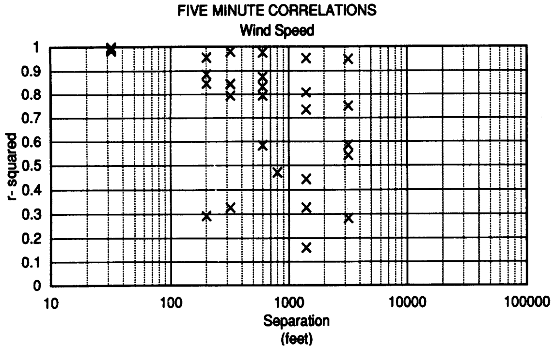
Figure 14. Five Minute Wind Speed Correlation at Zero Lag
