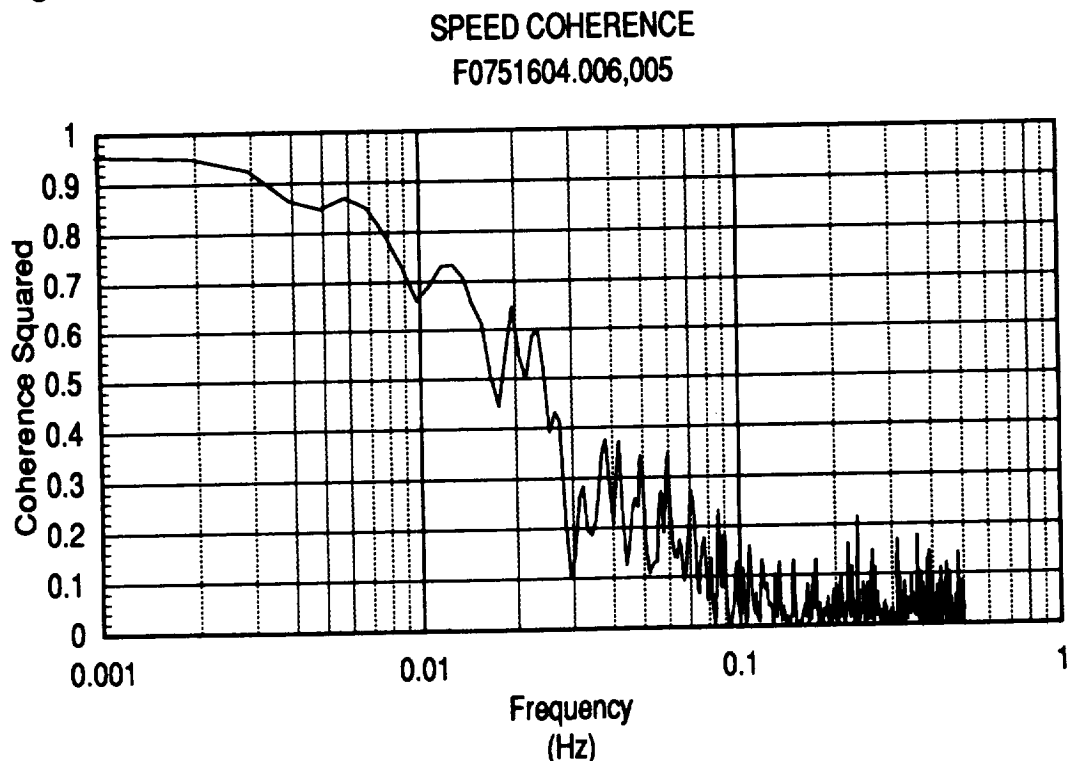
Figure 11. Wind Speed Coherence Corresponding to Figure 10
