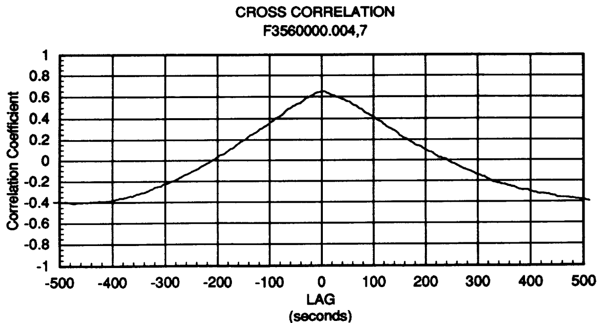
Figure 15. One Second Lagged WS Correlation, Files F3560000.004, 7
