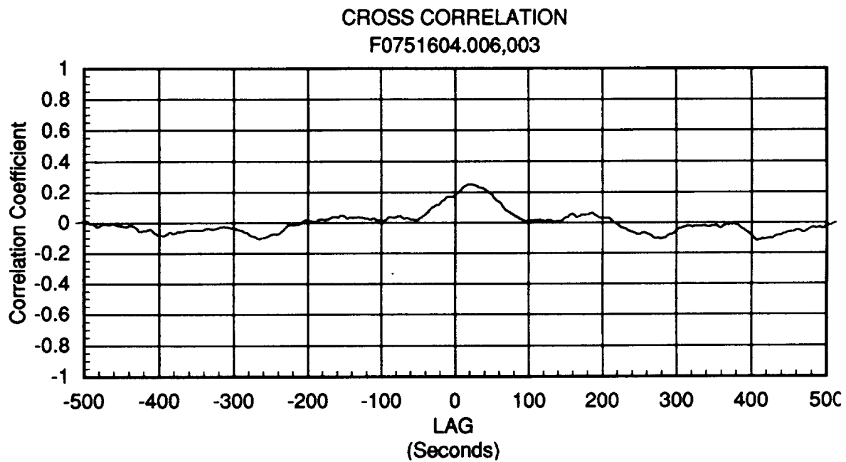
Figure 7. Wind Speed Correlation Corresponding to Figure 6
