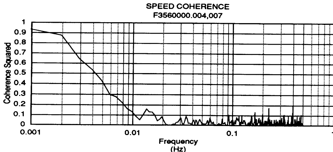
Figure 25. Coherence Spectrum, 800', With Trends
