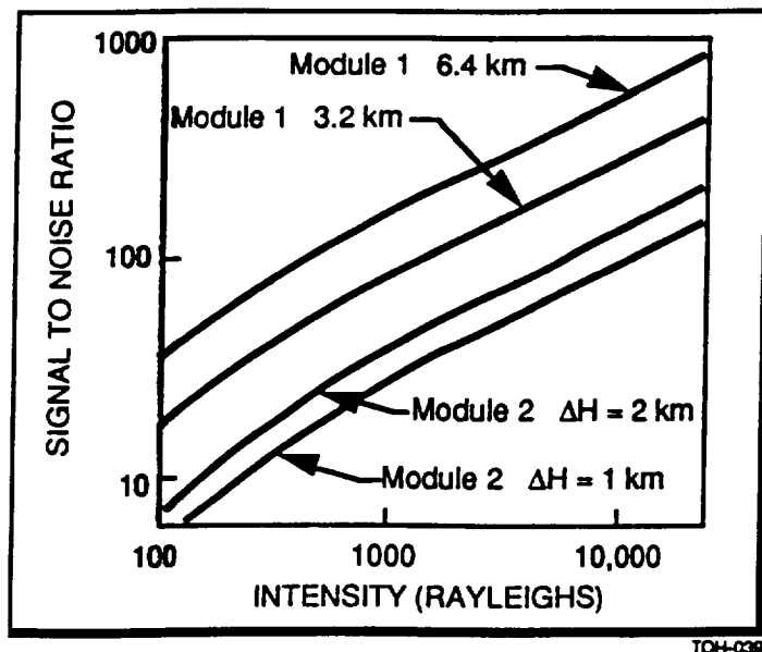
Figure 2-3. The signal to noise ratio of typical modules of the TIPE Instrument, including quantum, read out, and dark current noise contributions. The top two curves refer to a nadir view module with pixel sizes of 6.4 and 3.2 km. The bottom two curves refer to a limb view module with height resolution binning of 1 and 2 km.
