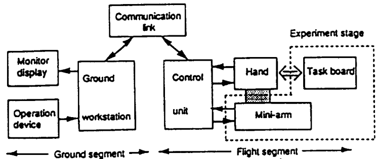
Figure 3. System Configuration
