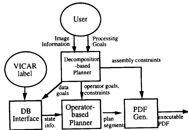
Figure 1: MVP Architecture
