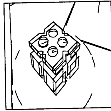
Figure 8: Last iteration
