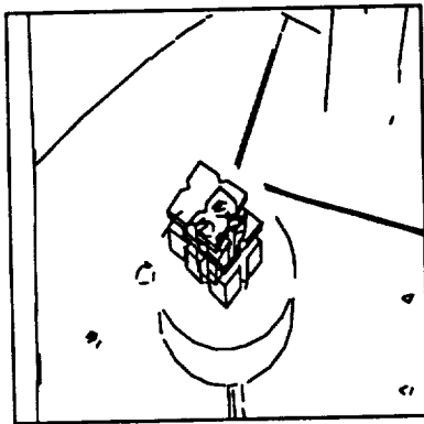
Figure 7: First localization
