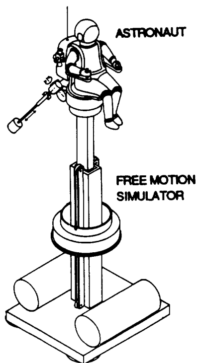
Figure 7. Application of simulator for astronaut extra vehicular activity training.
