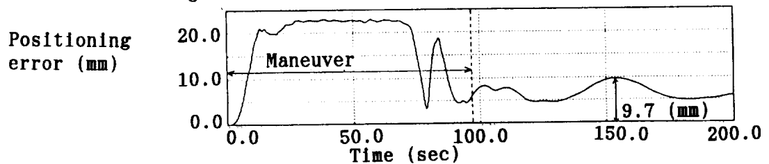
Figure 4. Position error in handling the 2300 Kg payload.
