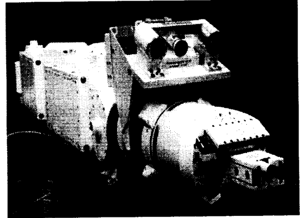
Figure 3. End-of-Arm Tooling with Wrist Camera & Lights
