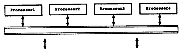
Figure 2: System architecture
