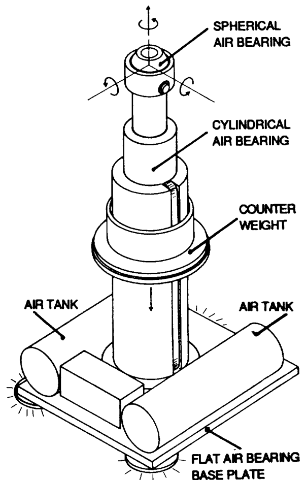
Figure 2. Configuration of free motion simulator.
