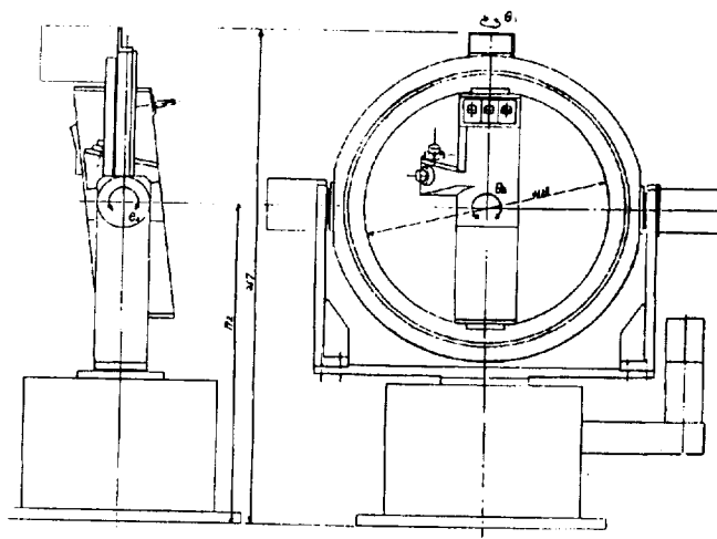
Figure 3. Structure of the hybrid master handle
