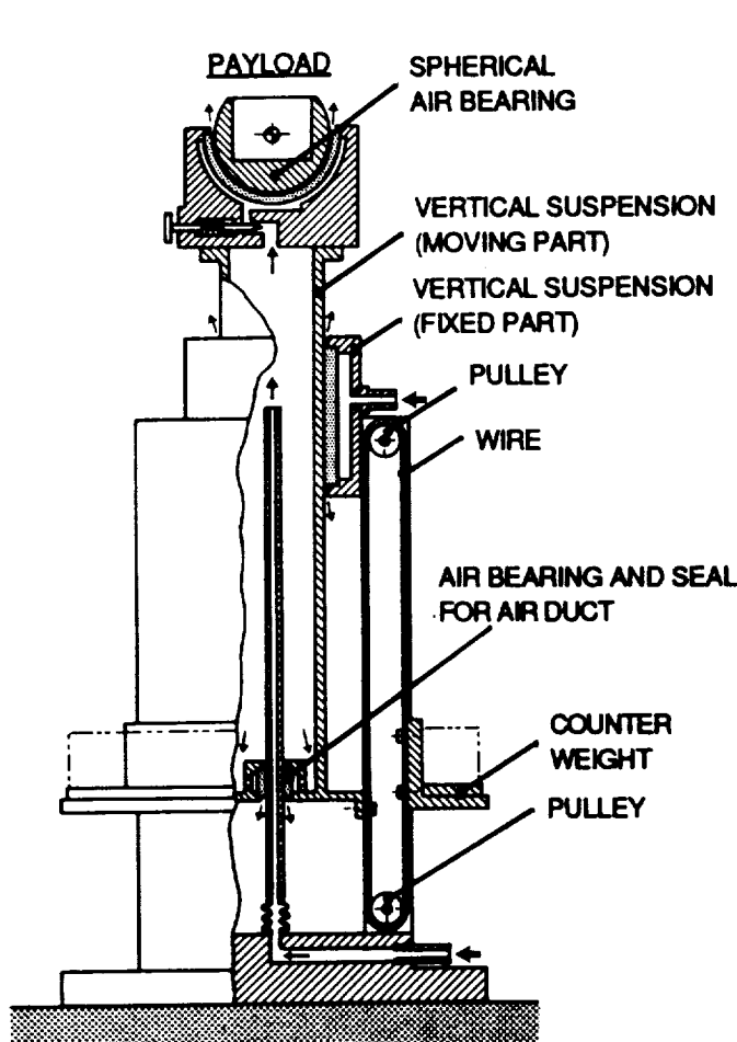
Figure 1. Illustration of sectional view of air duct mechanism.
