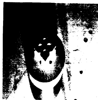
Figure 4: First image
