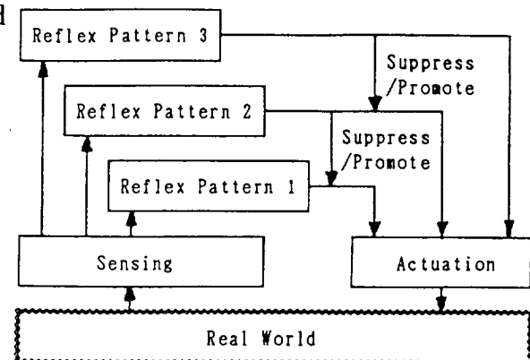
Figure 1. Subsumption Architecture
