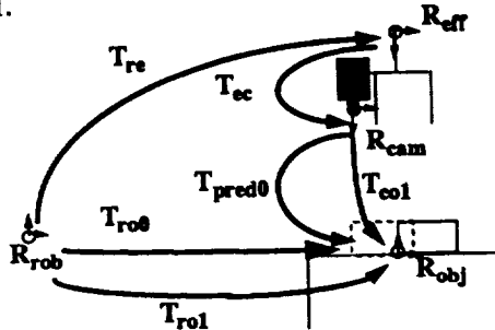
Figure 6: Model prediction
