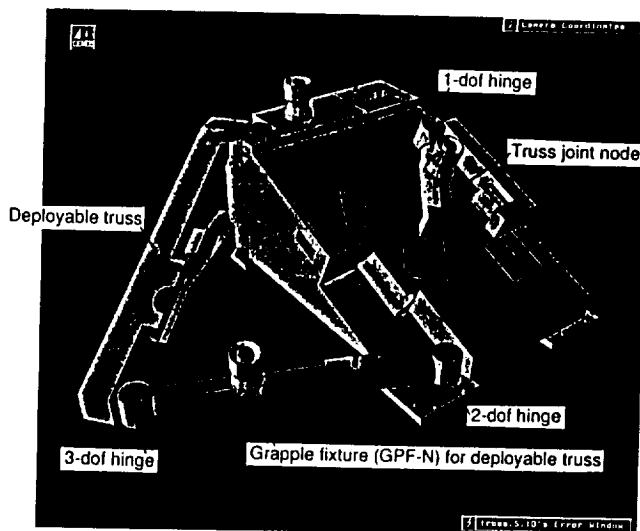
Fig.3 Deployed configuration
