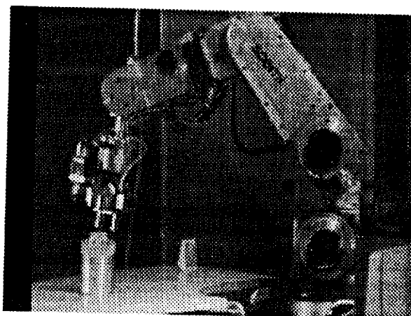
Figure 1: The LAAS experimental testbed work, we only use a classical "Look and
