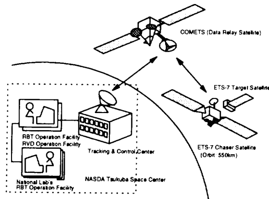
Figure-3 ETS-7 RVD & RBT Experiment System
