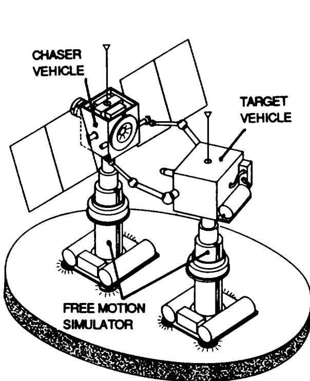
Figure 6. Method of simulating docking or berthing systems.
