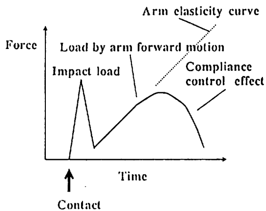
Figure 1. Typical transient force profile on capture and berthing of satellite
