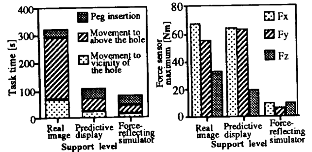
Figure 8. Force sensor maximum (Time delay : 4 [s])
