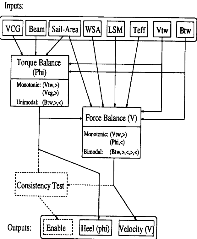
Figure 2: Yacht Velocity Model Dataflow Graph
