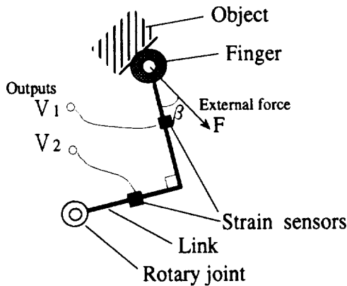
Fig.5 Grip force sensor
