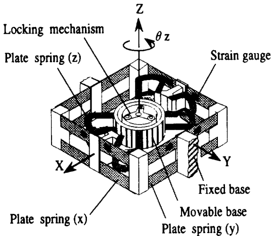
Fig.6 Wrist compliance device
