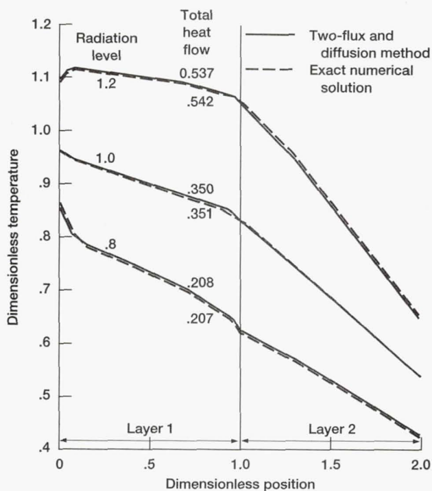
Temperatures and heat flows predicted by combined two-flux and diffusion method in two-layer composite with refractive indices of 1.5 and 3.
