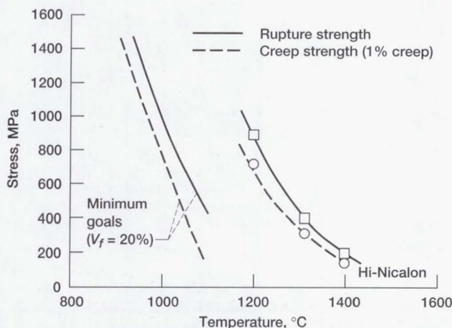
Fiber minimum creep and rupture strength goals based on composite performance equivalent to superalloys.
