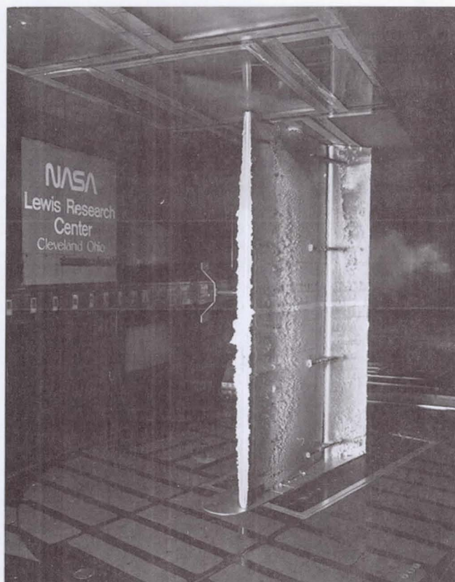
Ice on multielement wing in Lewis Icing Research Tunnel.
