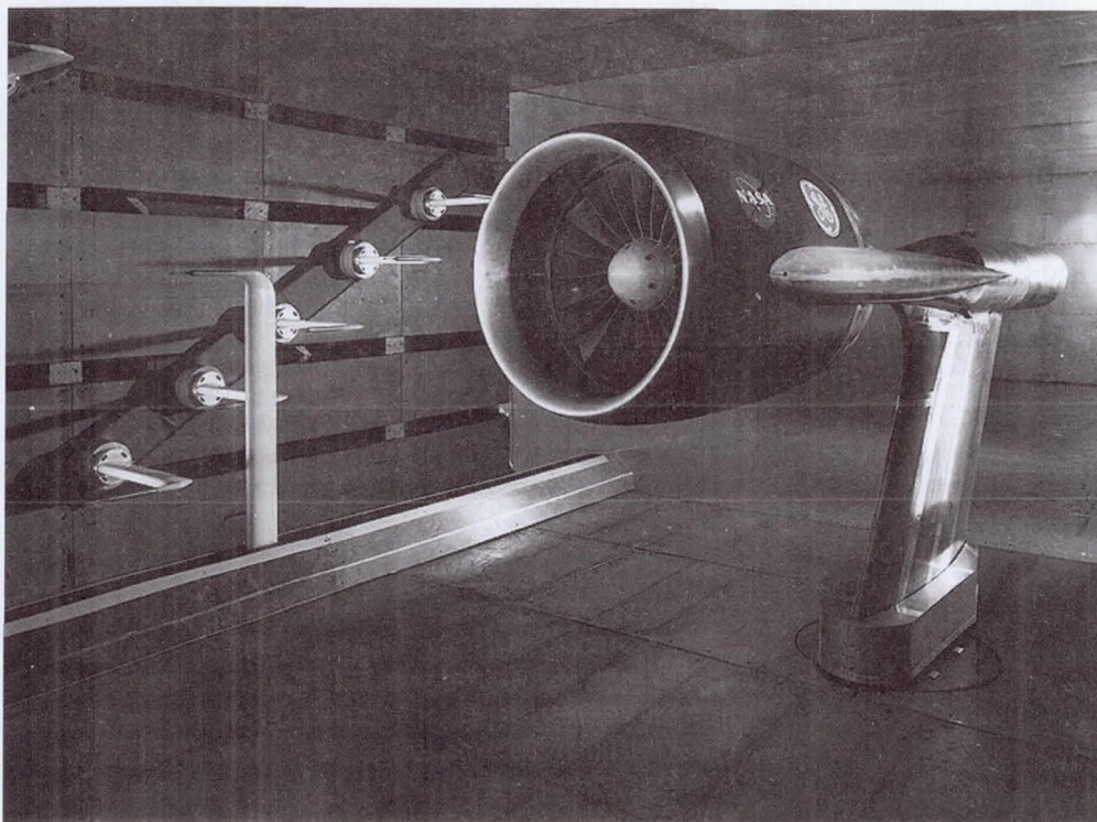
GE universal propulsion simulator installed in wind tunnel.
