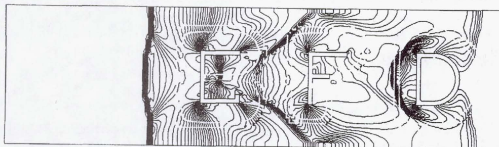
Top: DRAGON grid for letters "CFD." Bottom: Evolution of pressure contours at two representative times.
