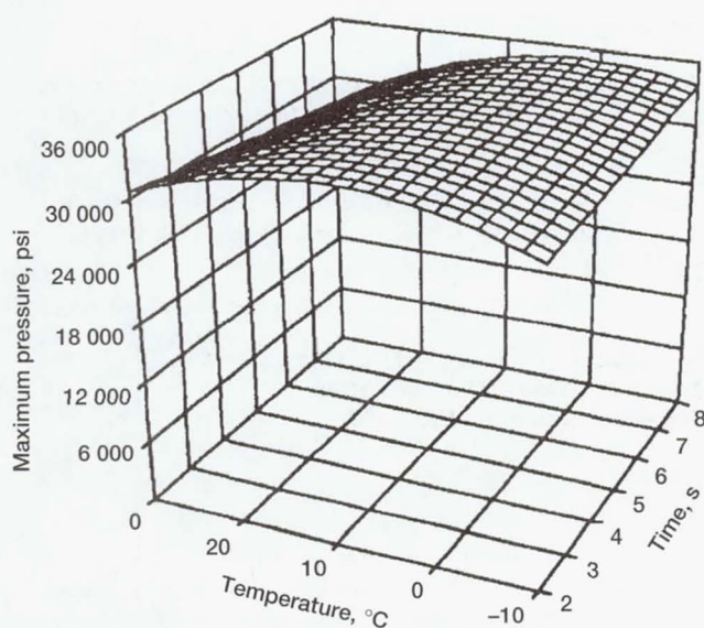
Predicted response surface for maximum mechanical stress in terms of oxidation conditions of conductive polymer films.
