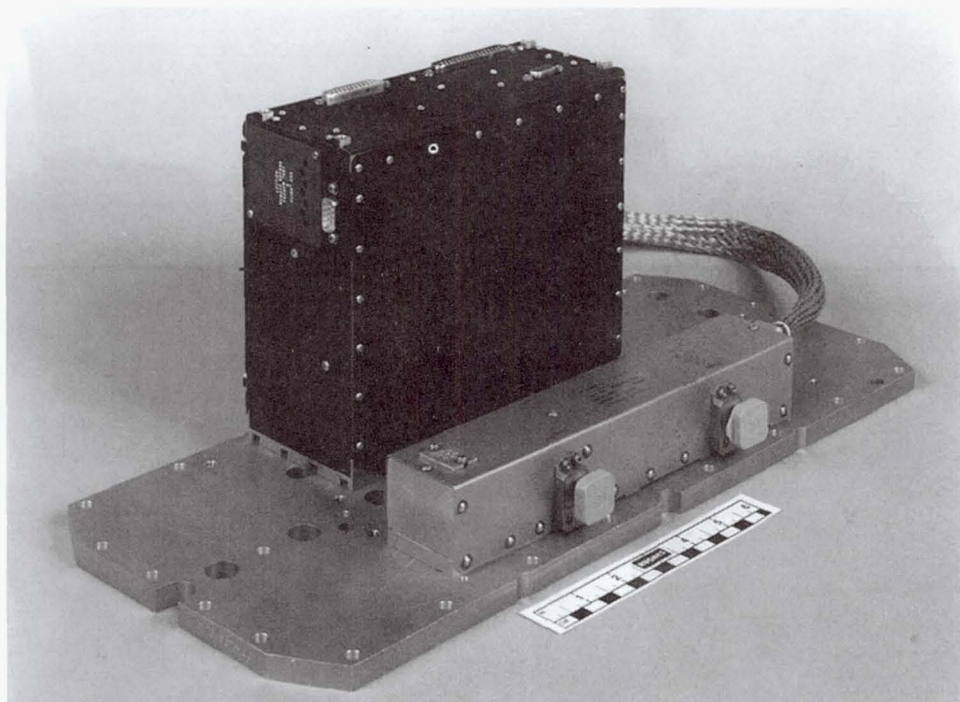
Packaged engineering qualification model Ka-band TWTA for the Cassini mission. The TWT is shown in the foreground. (Courtesy of Hughes Industrial Electronics Co.)
