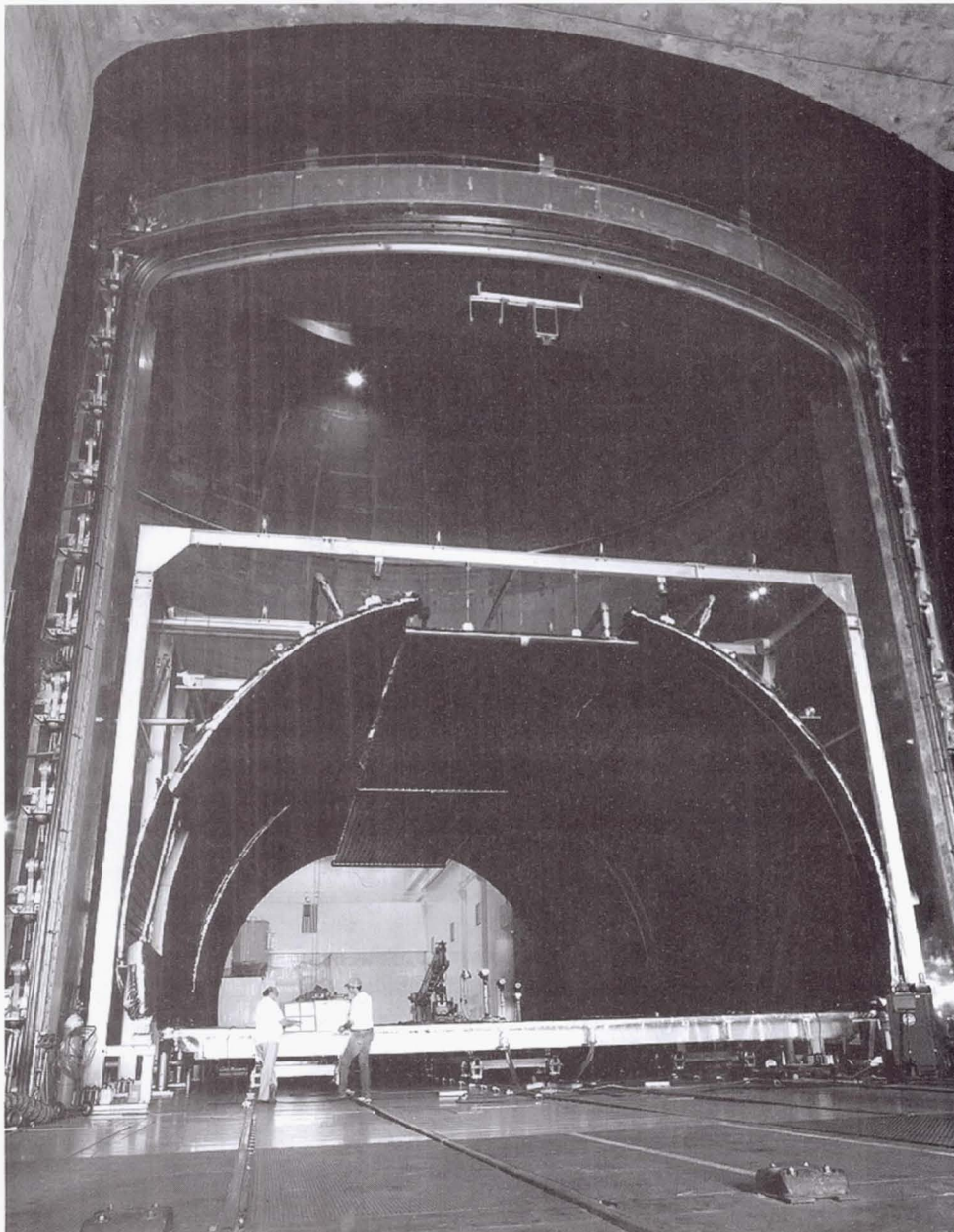
Cryoshroud for thermal vacuum testing at SPF.
