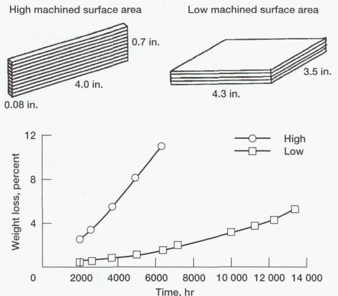
Results of aging PMR-15 composites at 500 °F in air.
