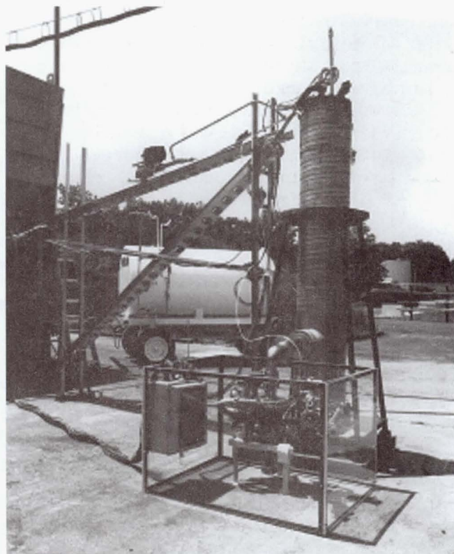
RL-10 turbopump and supply tank before installation of quartz viewing tube.
