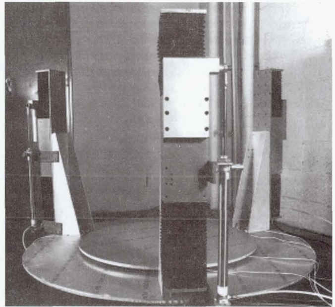
Reaction-compensating platform.
