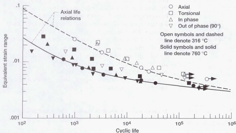
Summary of axial-torsional fatigue data on Haynes 188 at 316 and 760 °C.
