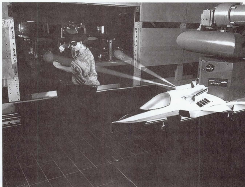
Spectral Rayleigh system in 9- by 15-Foot Low-Speed Wind Tunnel.
