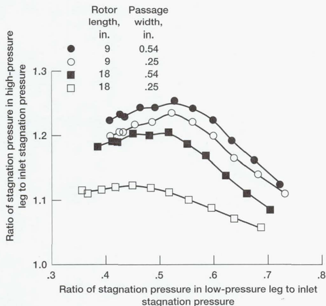
Wave rotor performance.
