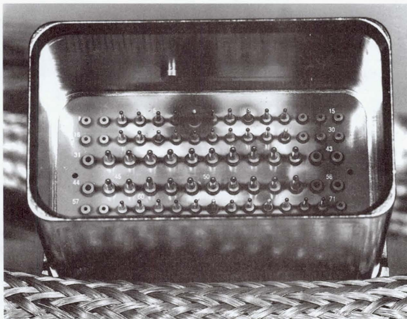
Charred 56-pin male D-connector after testing.
