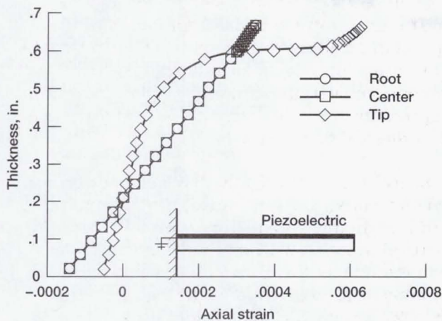
Typical mode shape and associated electric potential in top surface of sensory beam (second bending mode).
