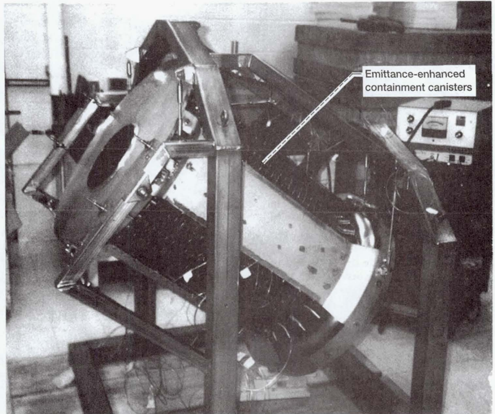
Partially assembled SD GTD heat receiver revealing some emittance-enhanced containment canisters.
