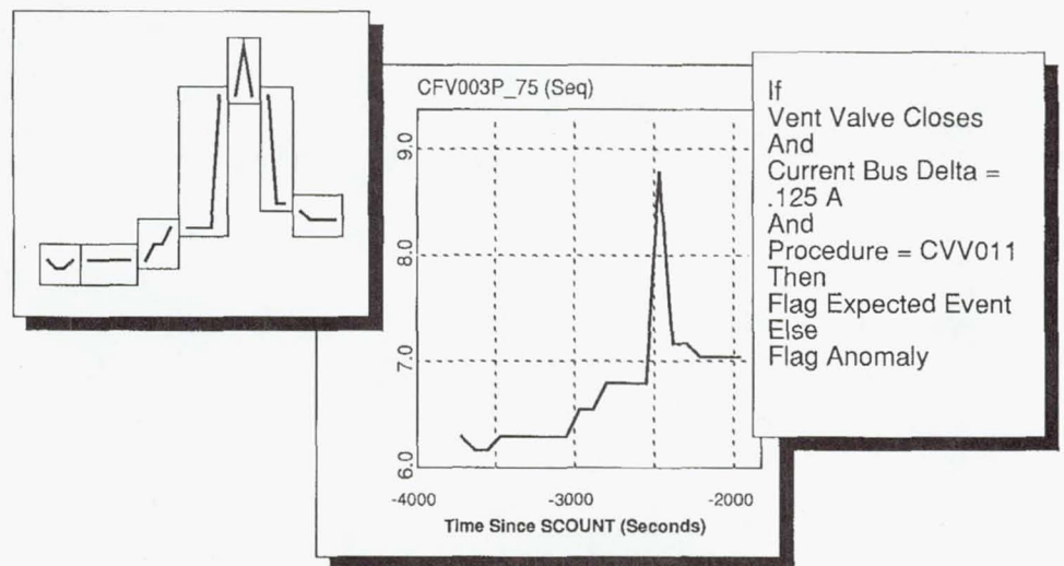
Feature extraction.
