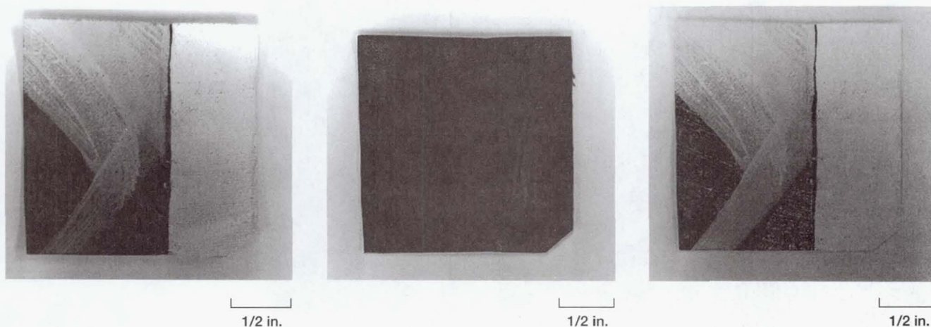
Original painting sample on canvas (left), sample after exposure to smoke (center), smoke-exposed sample after atomic oxygen cleaning (right).
