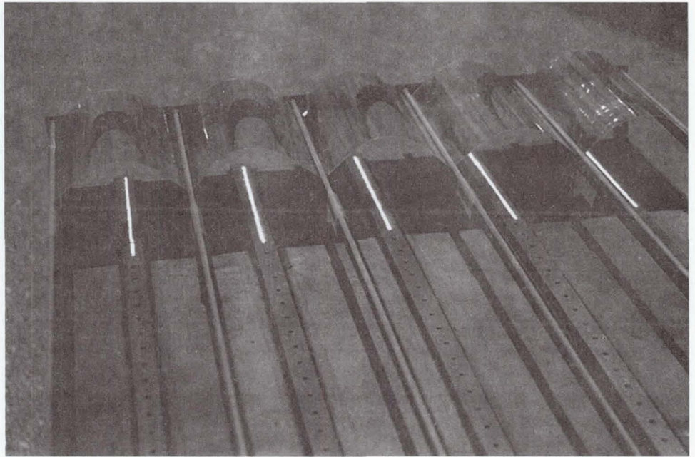
Prototype module of linear refractive concentrator focusing sunlight.
