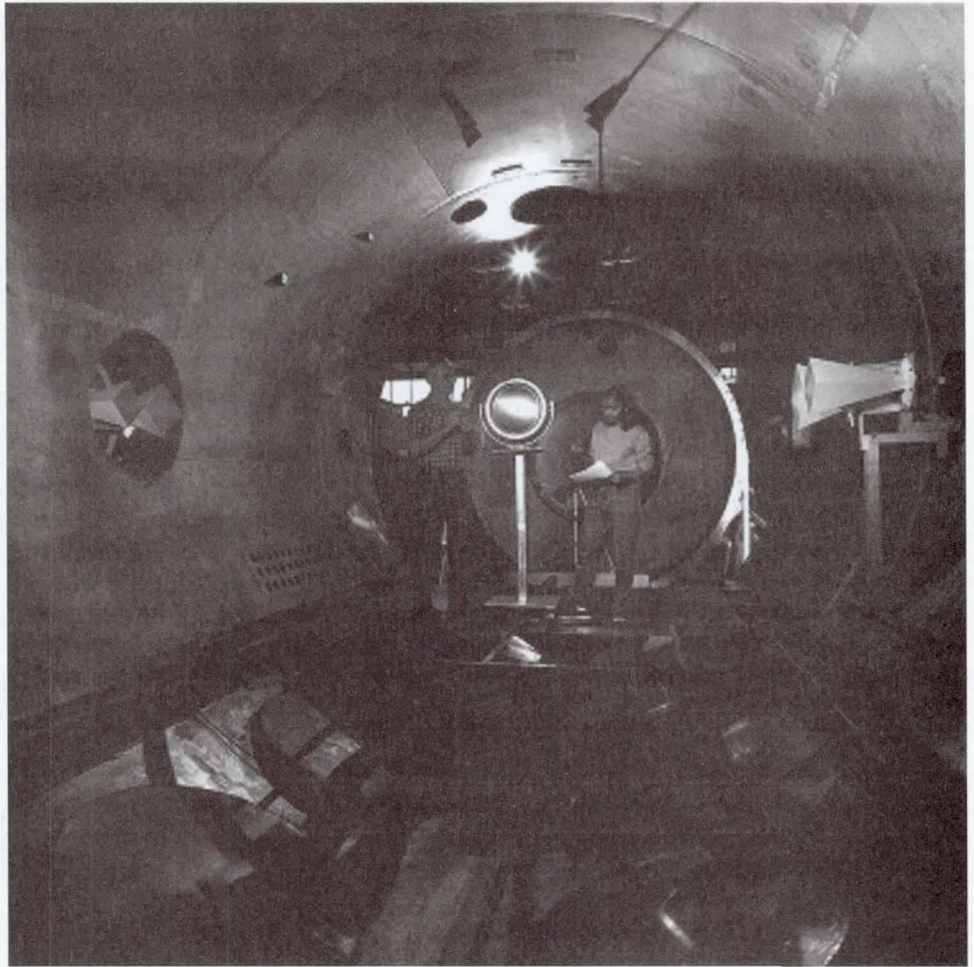
New NASA plume impacts test bed.
