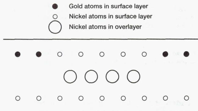
Lowest energy configuration for gold-nickel surface alloy for 0.067 monolayer coverage.
