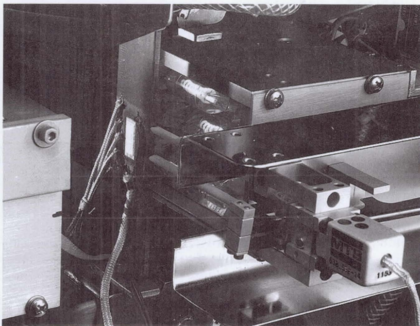
Gaged IN100 test specimen in thermomechanical loading frame equipped with quartz-lamp heating system.
