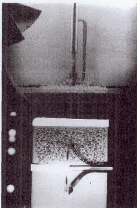
Side and bottom views of R-113 at 8 \text{ W/cm}^2 boiling on Earth (left) and during STS-47 mission (right).
