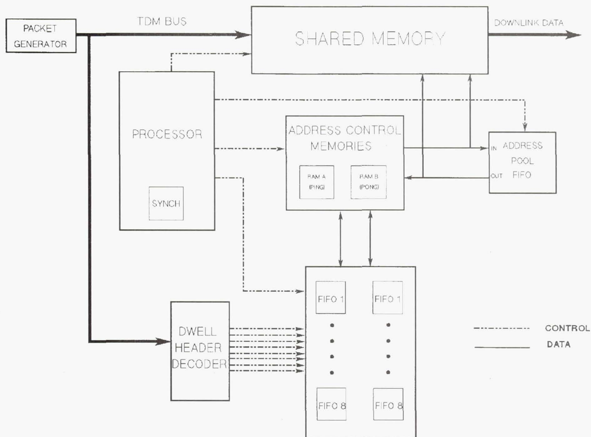
Shared-memory-per-beam architecture.
