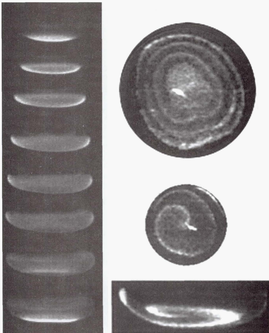
(Left) Axial view of propagating radial pulsation as flame propagates through tube. (Right top) Radial view of first four frames. Time between consecutive images, 1/500th sec. (Right bottom) Axial and radial views of rotating spiral wave.
