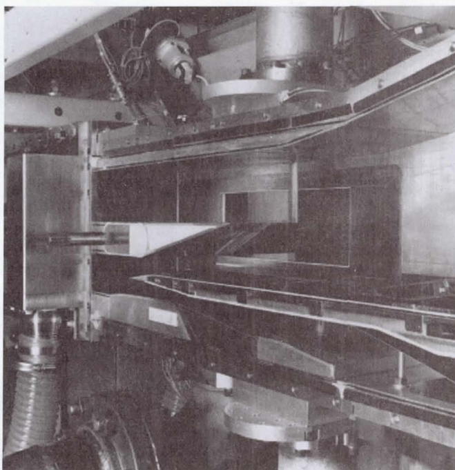
Core inlet/bypass nozzle installed in UTRC dual-flow test facility.
