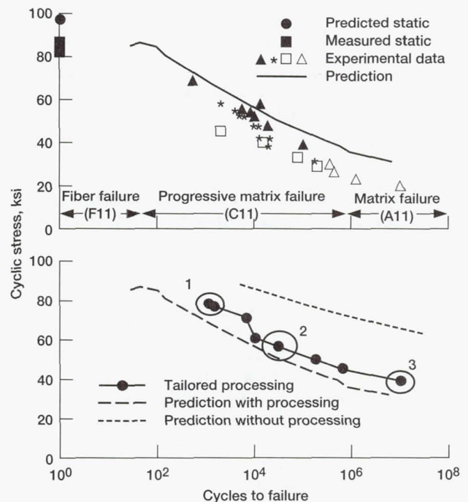
Isothermal fatigue prediction (top) and effect of processing optimization on fatigue life (bottom) for SiC/Ti-24Al-11Nb at 650 °C.
