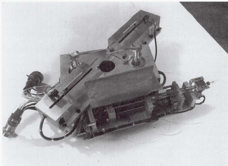
Droplet Combustion Experiment internal apparatus for drop tower testing.
