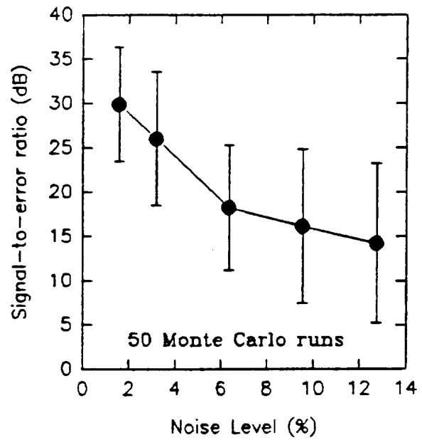
Fig. 15. S/E statistics
