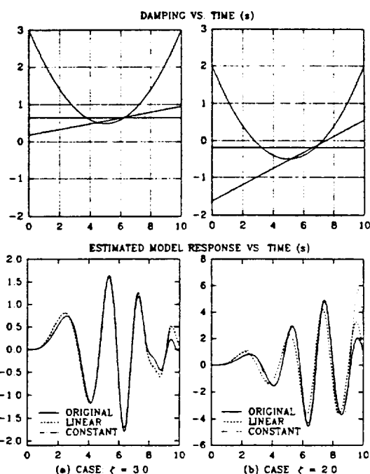
Fig. 11. Structural error effects.
