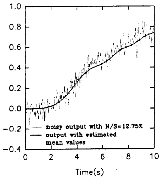
Fig. 14. Output data and model response
