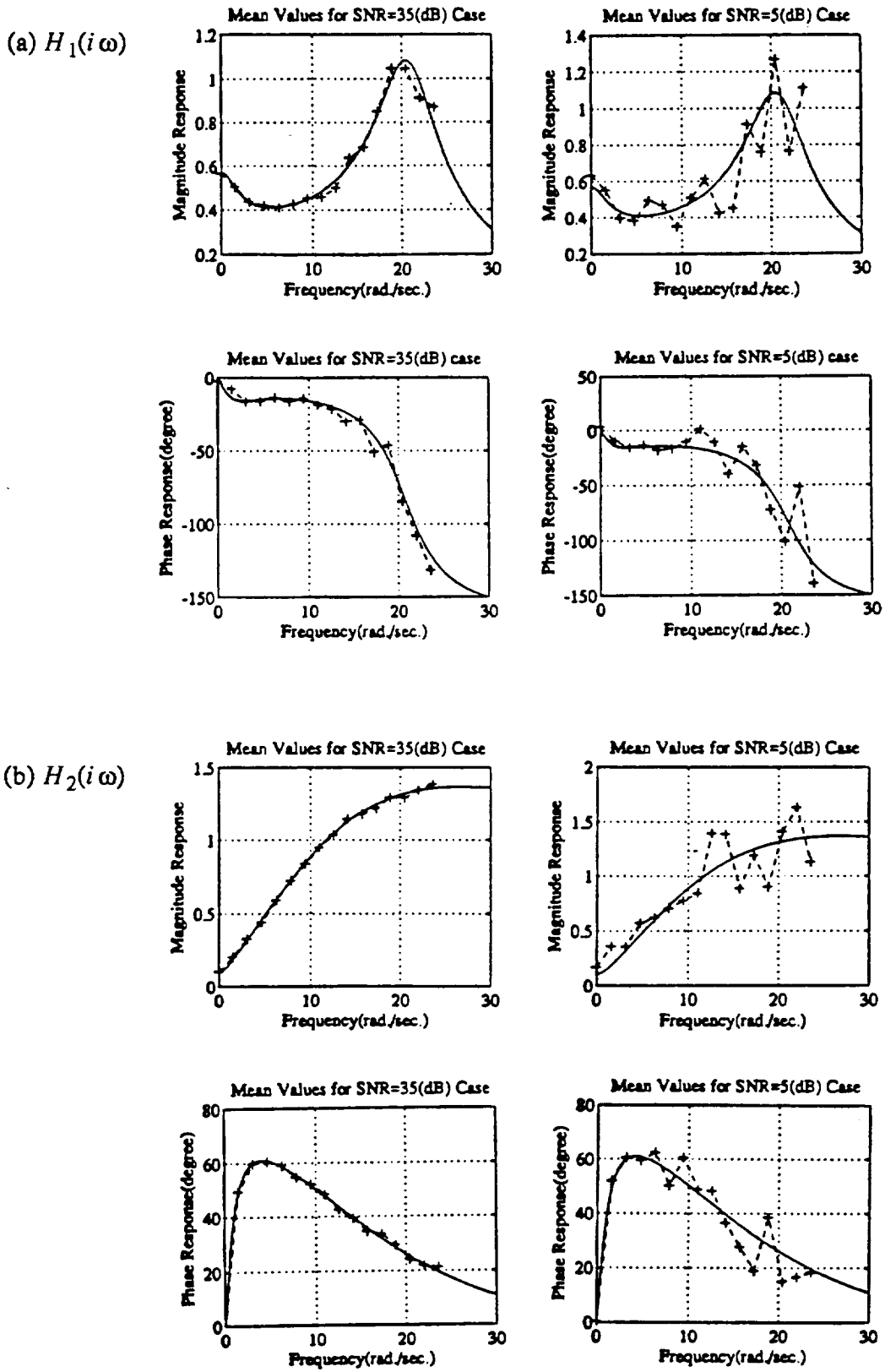
Fig. 9. Measurement noise effects for H_1 and H_2
