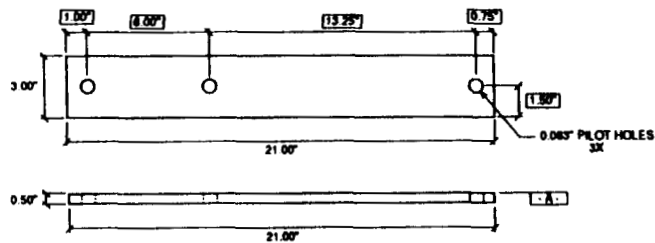
PL3 (5 REQD)
