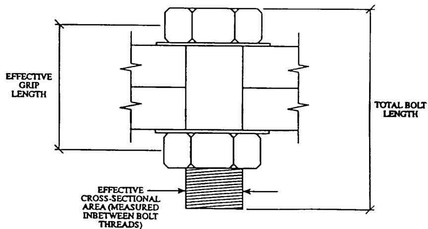
Figure 4.6 Input Dimensions for BoltMike.
