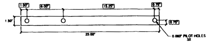
PS3 (5 REQD)
