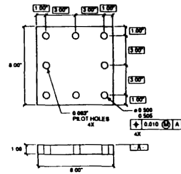
CPU (2 REQD)
