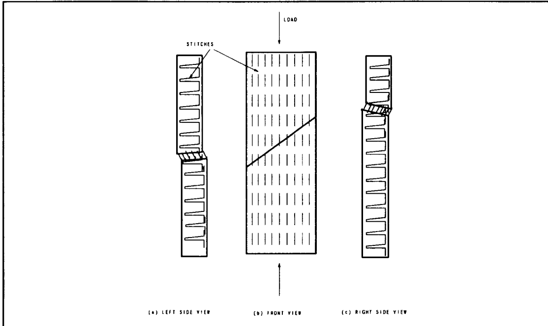
Figure 2-11: A sketch of a typical stitched sublamine buckling failure mode
