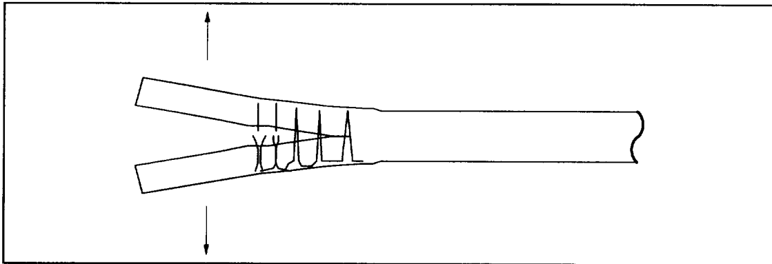
Figure 3-9(e): P-\delta continue to rise. After some time crackling sounds heard again. Crack extends to fifth stitch. Second stitch fails completely. Third partially debonded can be seen. Fourth appears bonded.
