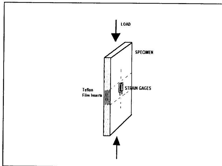
Figure 2-2: A sketch of typical sublamine buckling specimen
