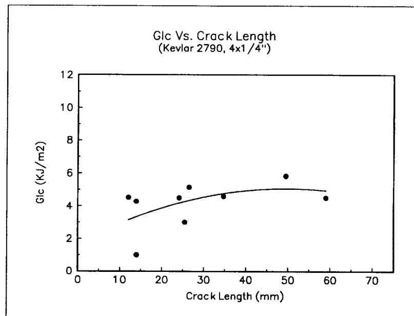
Figure 3-6: G_{Ic} vs. Crack length for Kevlar-2790, 4x1/4" stitched laminate
