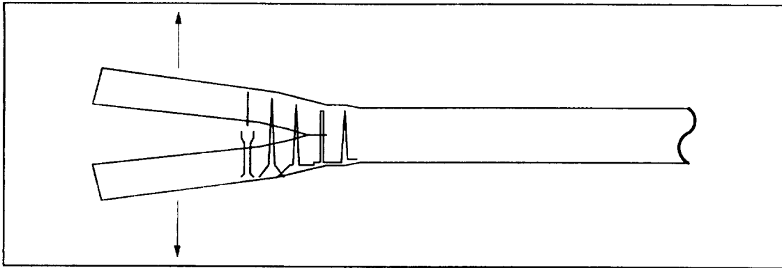
Figure 3-9(d): A little more loading breaks the first stitch. No perceptible load drop is observed at this point. Crack propagates up to the 4th stitch. Second partially debonded stitch can be seen. Third appears bonded.
