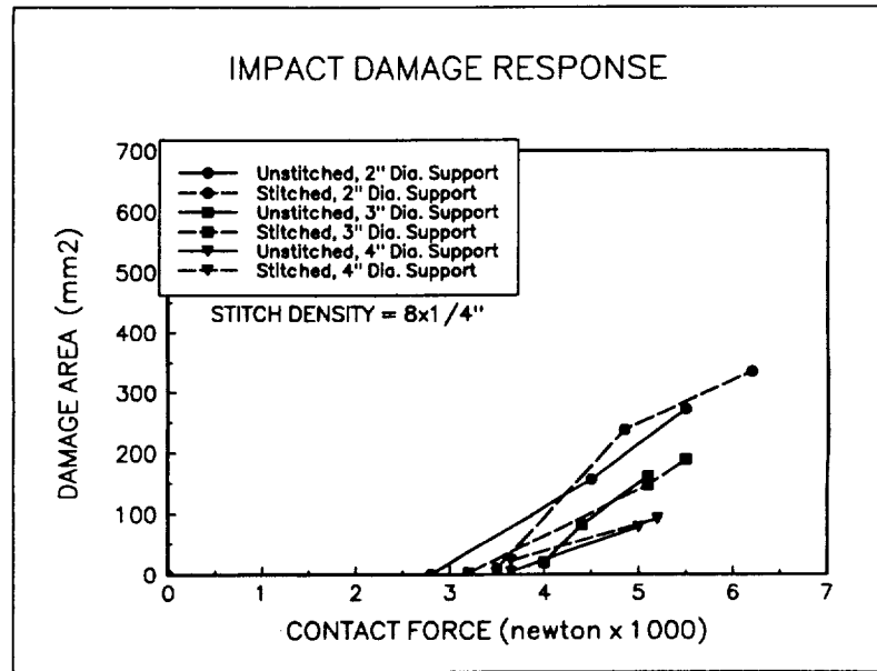
Figure 5-10: Impact Damage Area (C-Scan) vs. Contact Force for the unstitched and 8 \times 1/4" stitched laminates with variation in support ring diameter.
