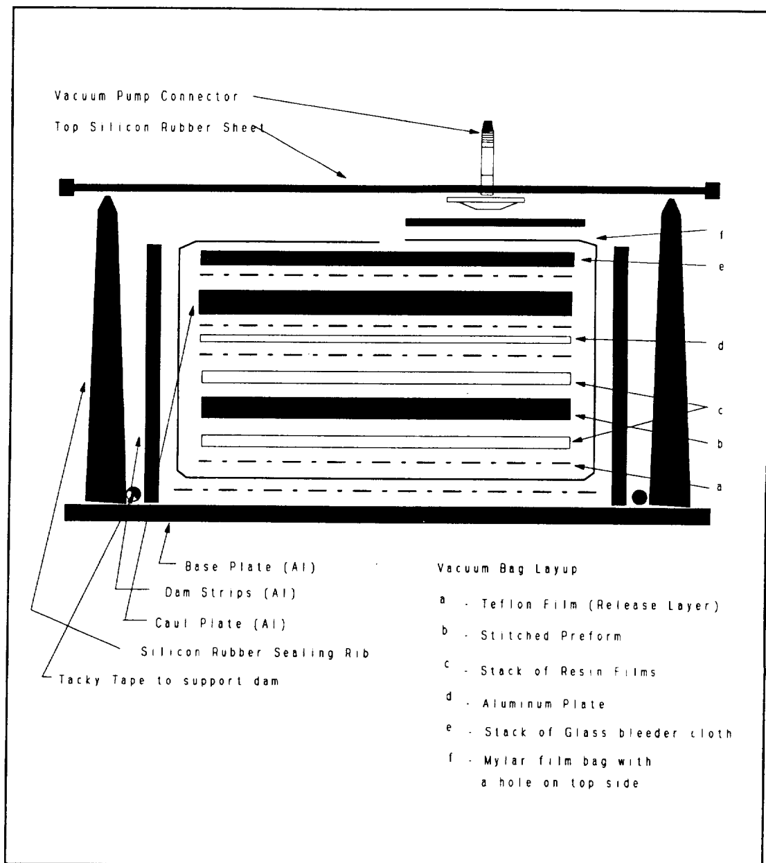
Figure 5-1: Vacuum bag lay-up of stitched graphite preform and resin films used for autoclave processing of the stitched laminates at the Center for Studies of Advanced Structural Composites.
