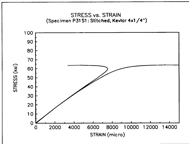
Figure 2-4: A typical stress-strain response for a stitched laminate.
