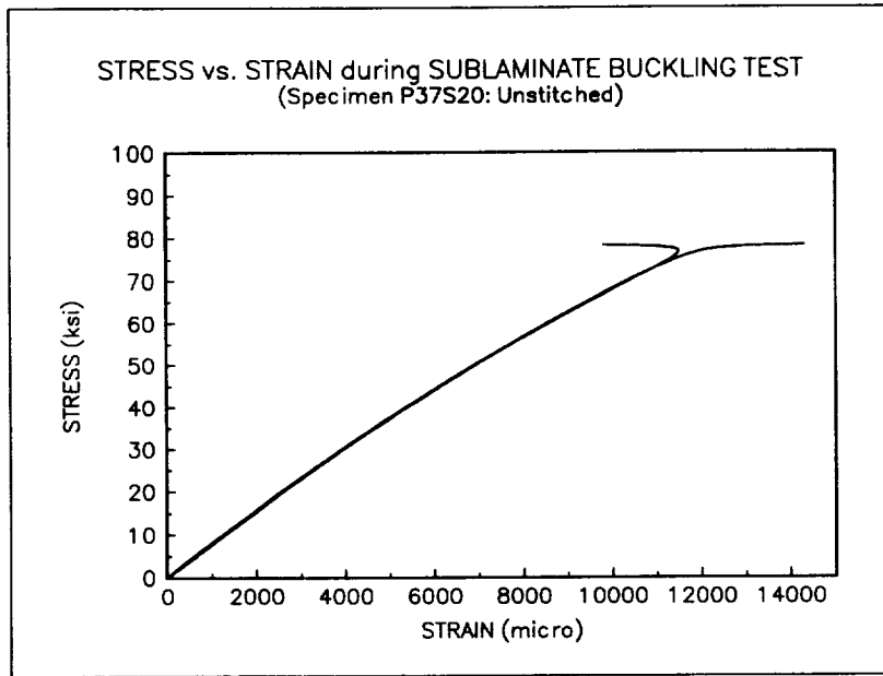
Figure 2-3: A typical stress-strain response for an unstitched laminate.
