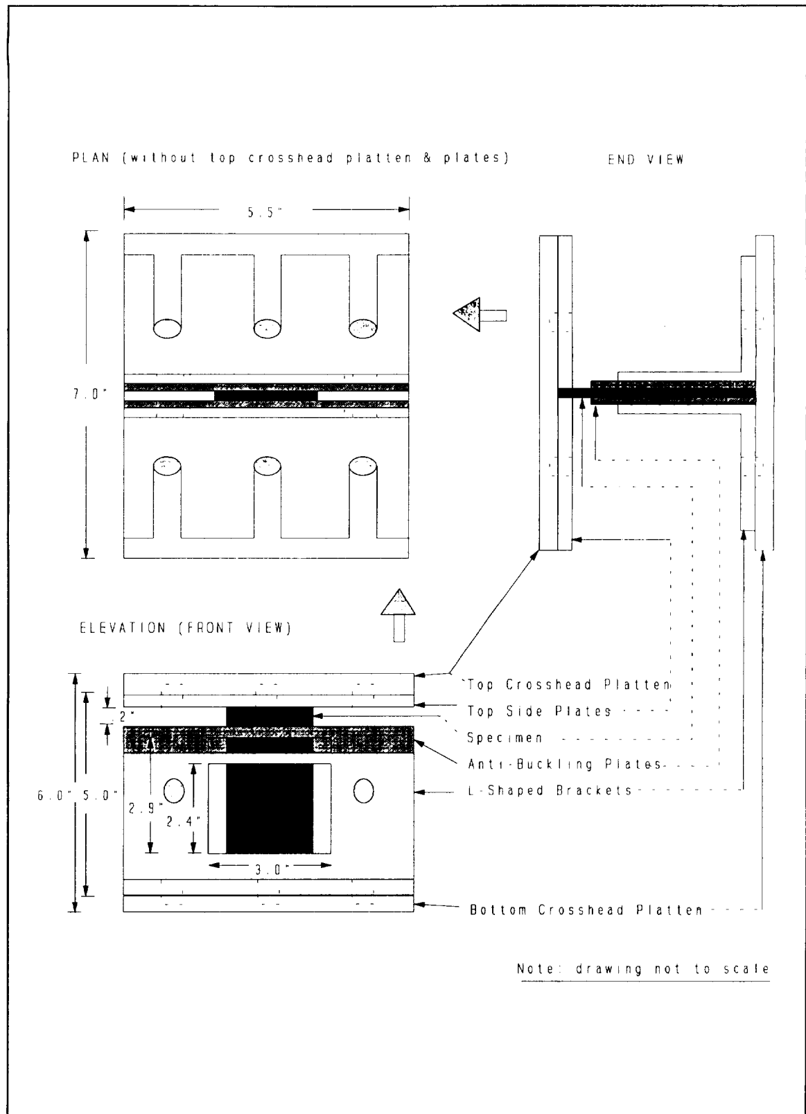
Figure A-3: Key dimensions of the UF-CAL test fixture shown for a 5" tall specimen
