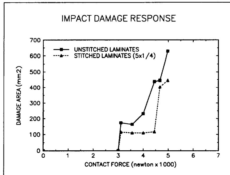
Figure 5-11: Impact Damage Area (C-Scan) vs. Contact Force for the unstitched and 5 \times 1/4" stitched laminates with 3" support ring diameter.
