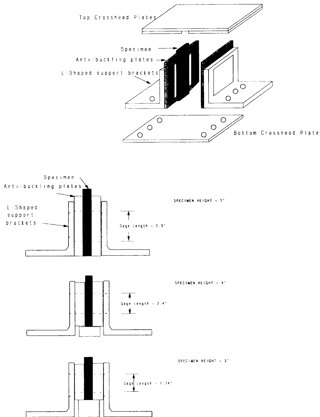
Figure 2-1: A sketch of the University of Florida Compression-After-Impact (UF-CAI) test fixture along with adaptations required for different specimen heights
