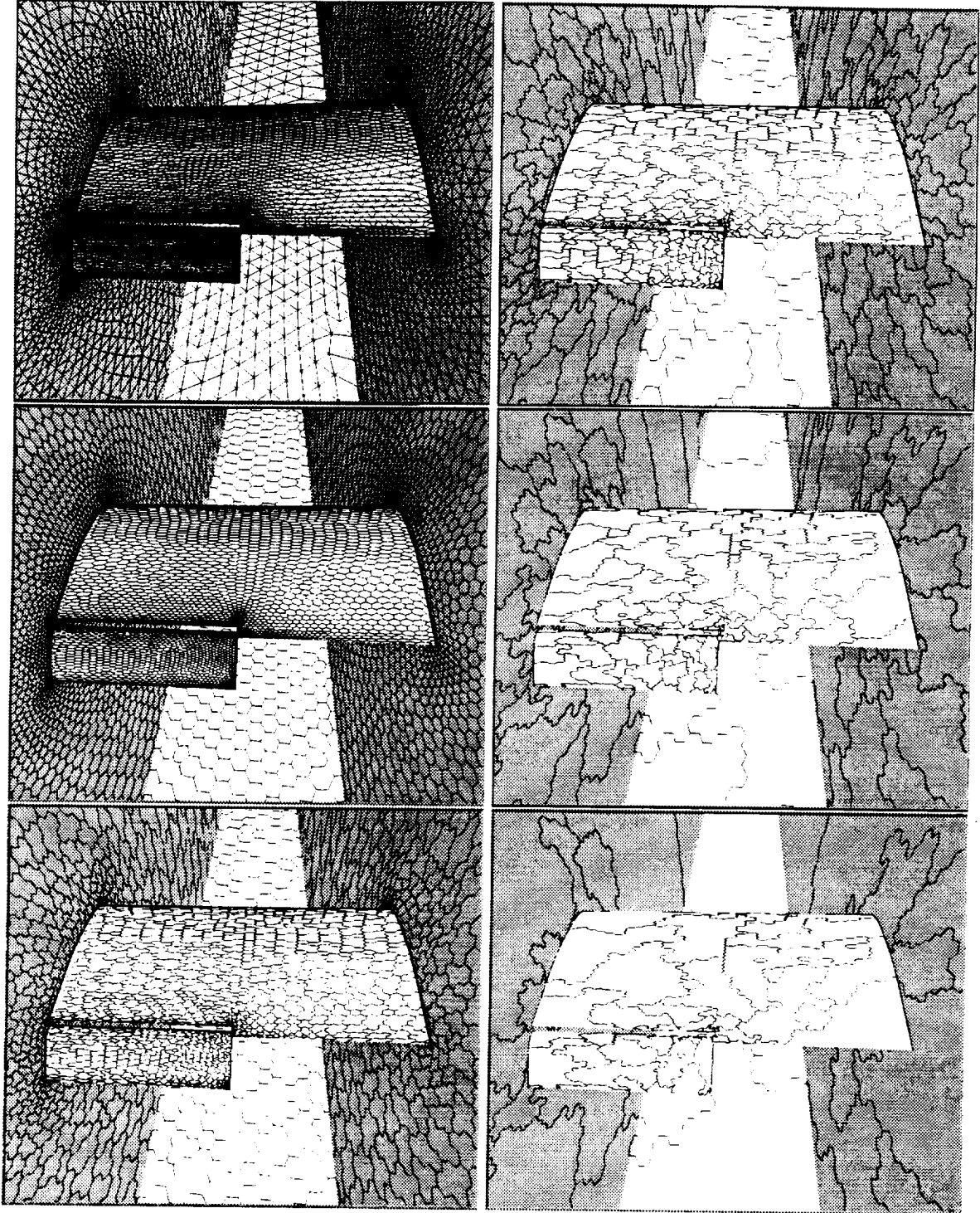
Figure 12: Initial Unstructured Grid, its Dual Mesh, and Four Agglomerated Coarse Mesh Levels Employed for the Multigrid Algorithm for the Partial-Span-Flap Wing in Wind-Tunnel Geometry (3000,000 points, 1.7million tetrahedra, wall spacing 10^{-5} ).
