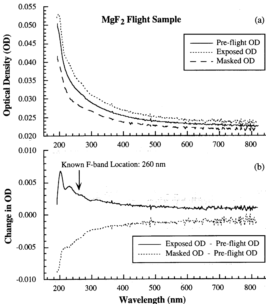
Figure 3. (a) Pre-flight and post-flight optical density (OD) spectra of the exposed and masked areas of sample \text{MgF}_2 -2. (b) The change in optical density due to the space exposure determined by the difference between the post- and pre-flight spectra from figure (a). The post-flight spectra show absorption features that could be associated with F-center formation only on the exposed side of the sample. Sample temperature varied with the ambient environment during space exposure.
