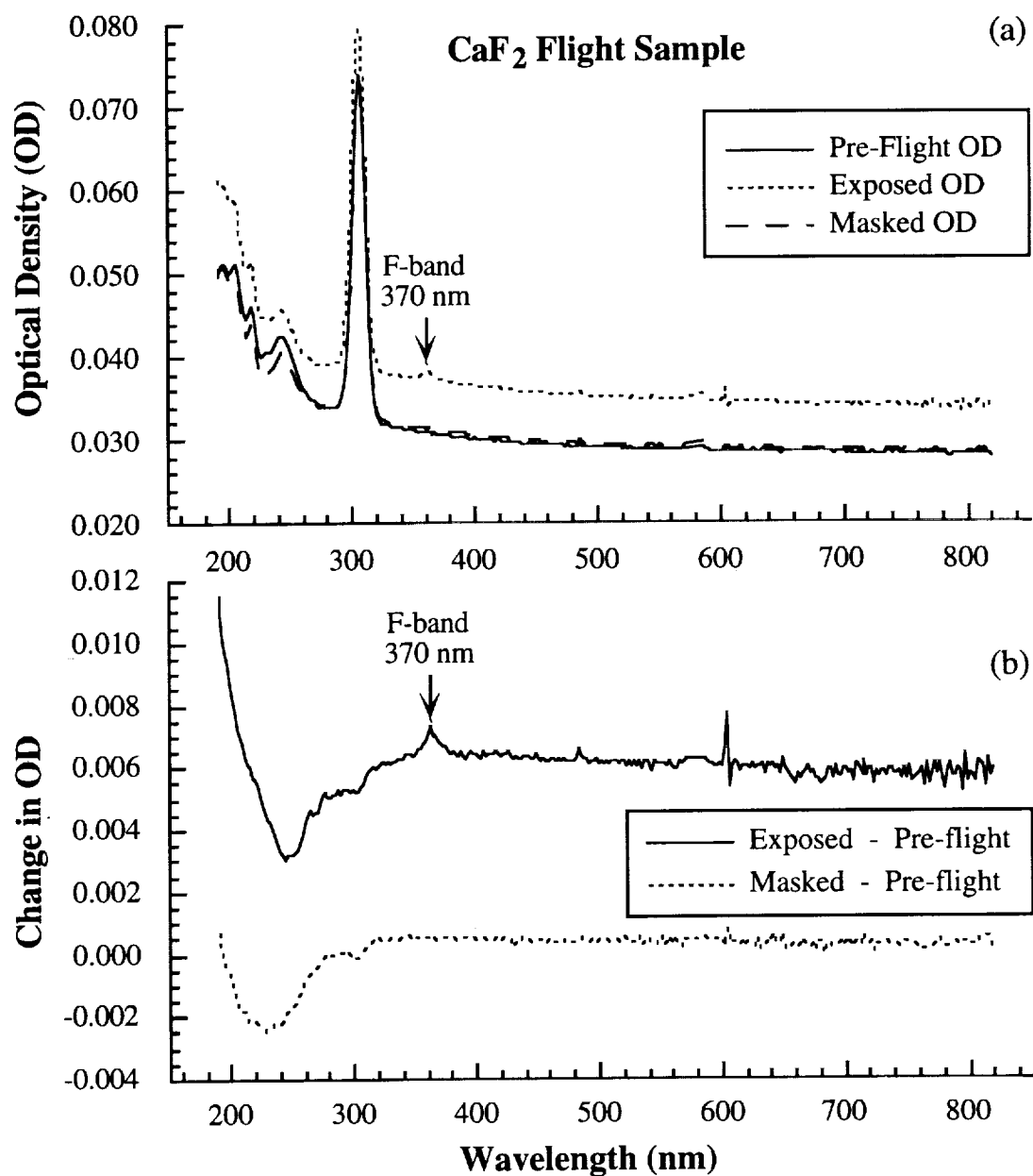
Figure 1. (a) Pre-flight and post-flight optical density (OD) spectra of the exposed and masked areas of sample \text{CaF}_2 -1. (b) The change in optical density due to the space exposure determined by the difference between the post- and pre-flight spectra from figure (a). The post-flight spectra show the formation of an F-band at 370 nm only on the exposed side of the sample. Sample temperature was held at 60°C during space exposure.
