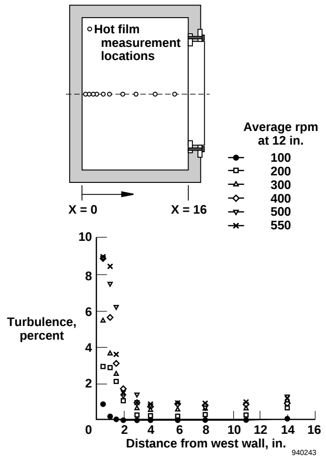
(b) Percent of turbulence as a function of distance from the west wall.
