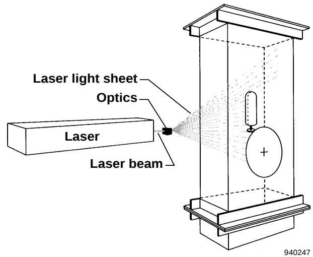
Figure 10. Laser light sheet system
