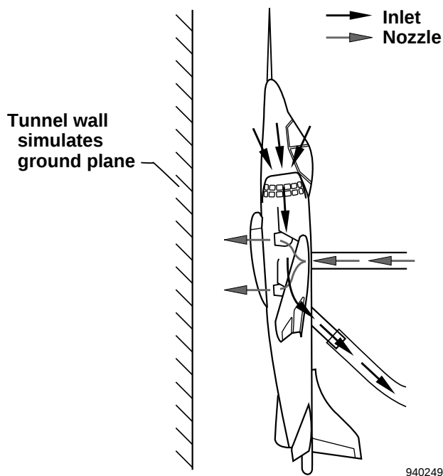
Figure 14. Harrier model with blowing and suction capabilities.
