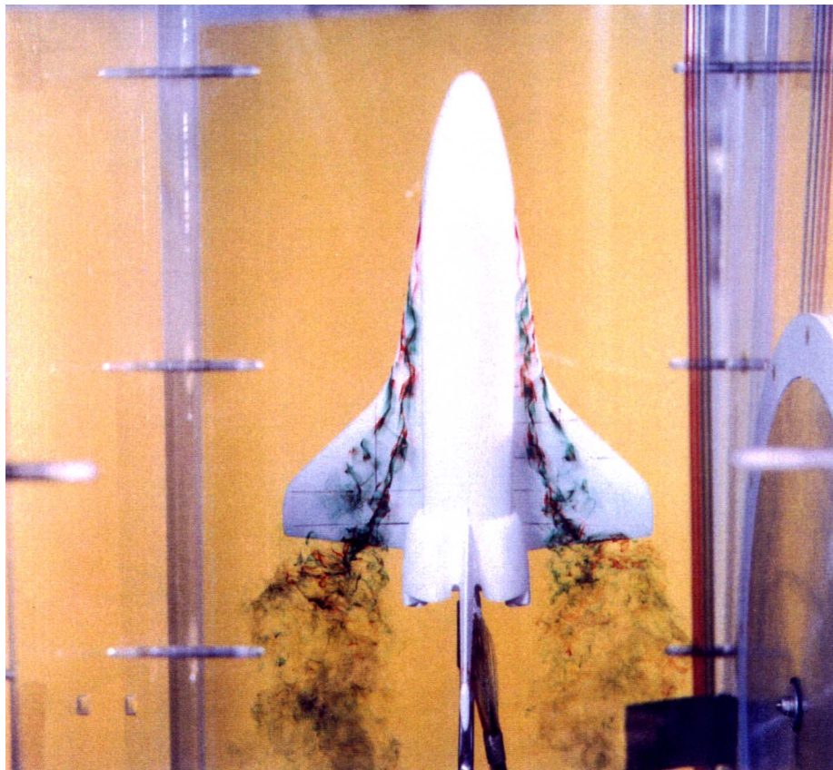
Figure 8. Top view of a shuttle model operating with the dye tracer technique in the vertical test section.
