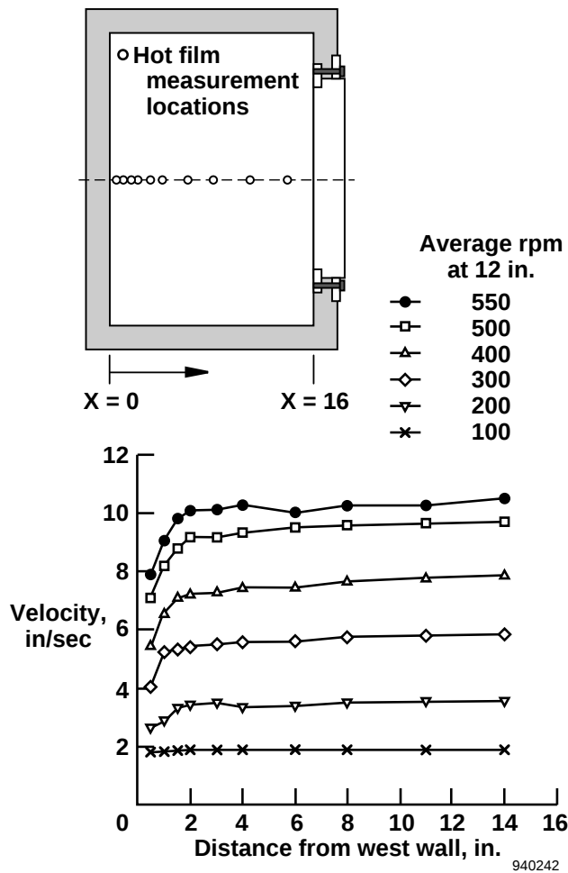
(a) Velocity as a function of distance from the west wall.
