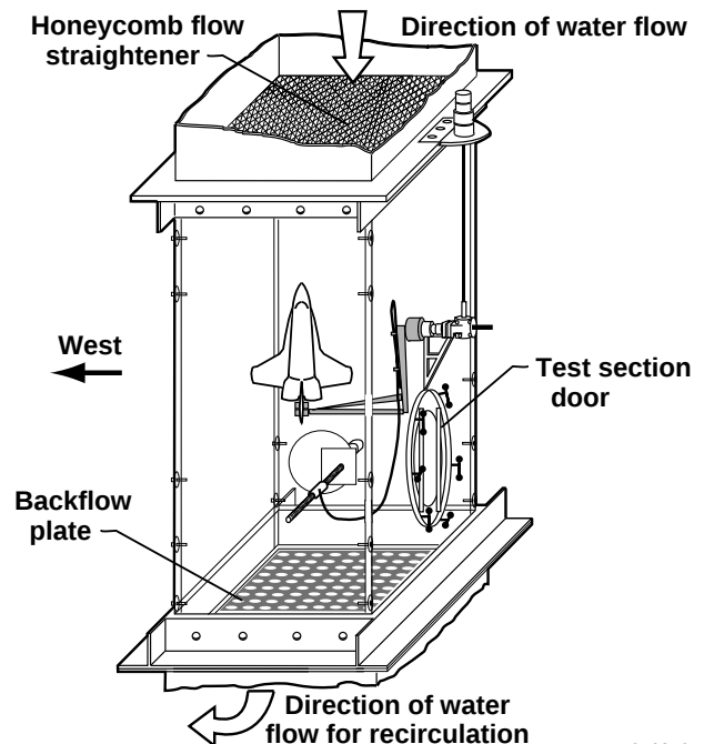
Figure 3. Vertical test section.
