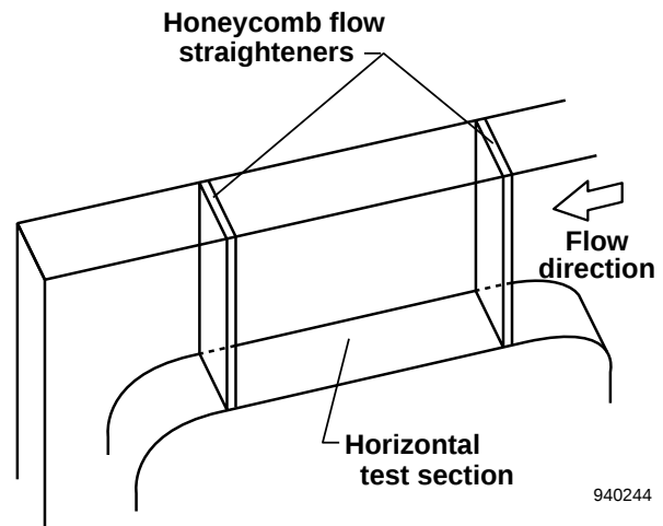
(a) Normal configuration.
