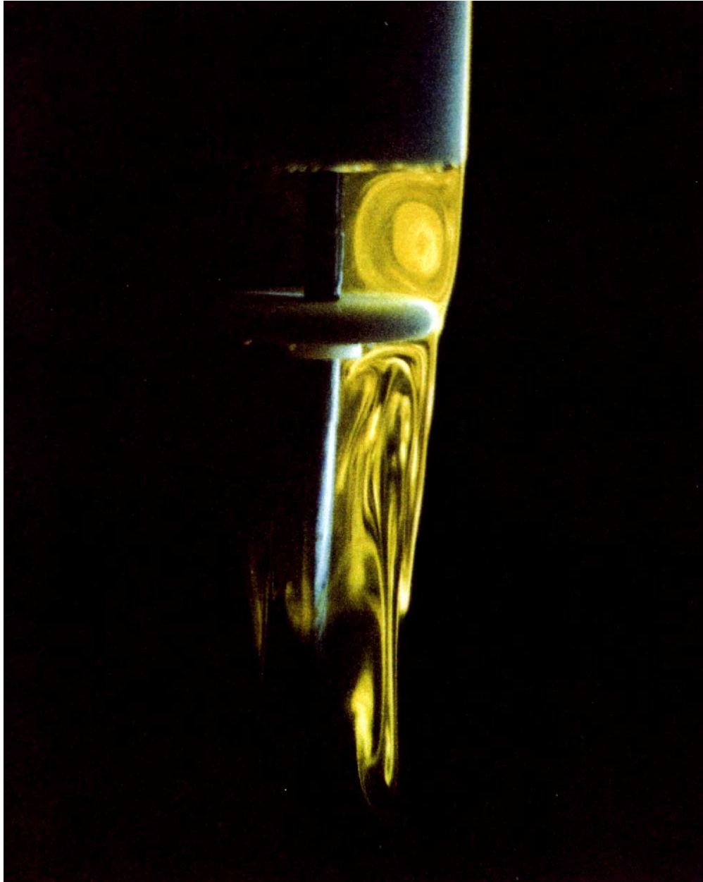
(b) Tracer material: Fluorescein sodium dye.
