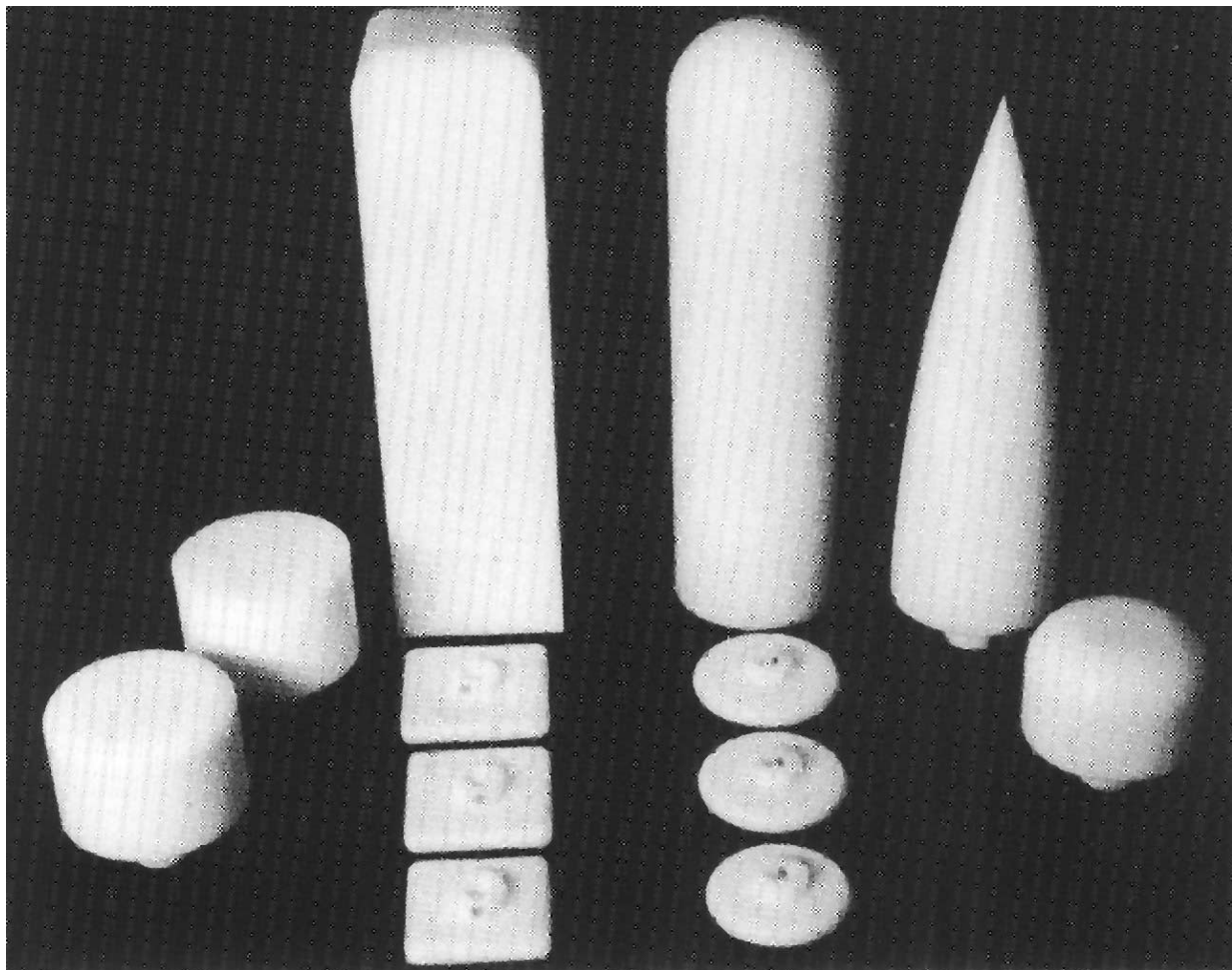
(a) Nose shapes, bodies, and disks used in the experiment.
