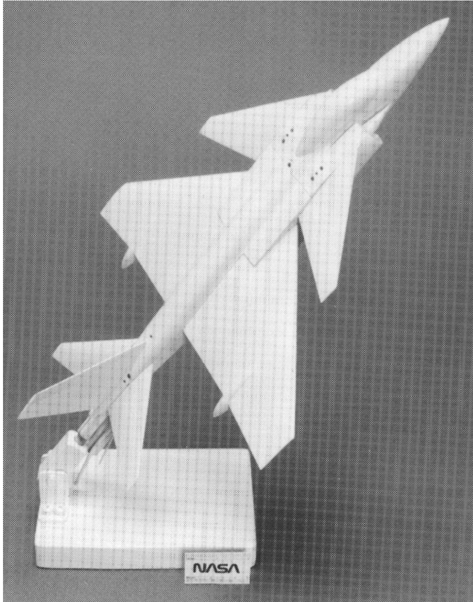
Figure 18. MCAIR 279 water tunnel model.
