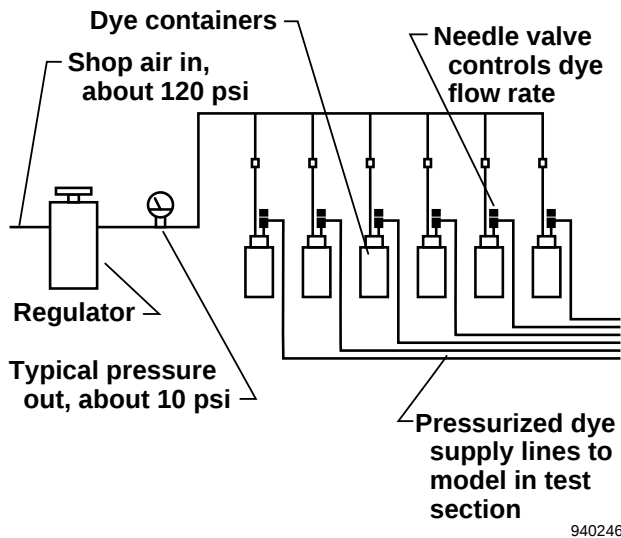
Figure 9. Schematic of dye supply system.
