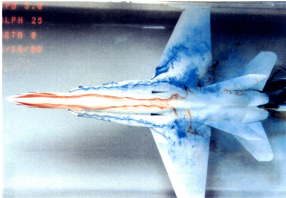
Figure 7. Side view of an F-18 model operating with the dye tracer technique in the vertical test section.
