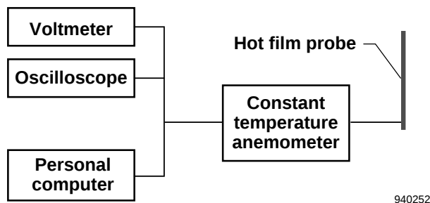
Figure A-1. Hot film constant temperature anemometer system assembled for use in the Flow Visualization Facility.
