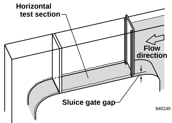
(b) Sluice gate configuration.
