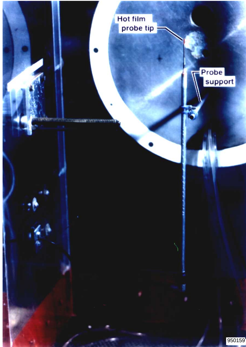
Figure A-2. Hot film probe installed in the vertical test section.
