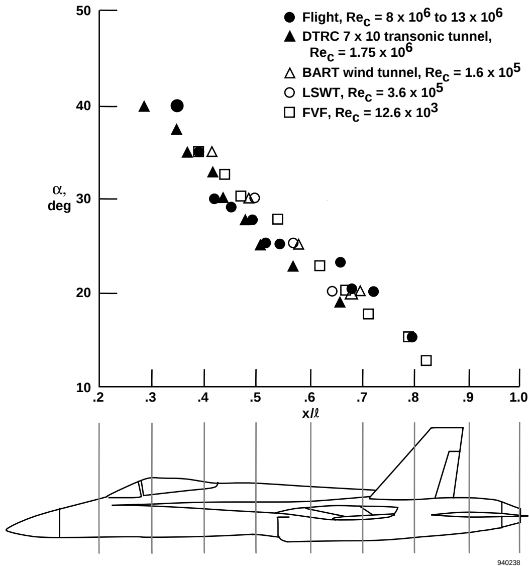
Figure 1. Comparison of F-18 airplane leading edge extension vortex core breakdown location between flight, water tunnel, and wind tunnel facilities.
