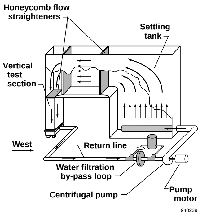
Figure 2. Flow Visualization Facility.
