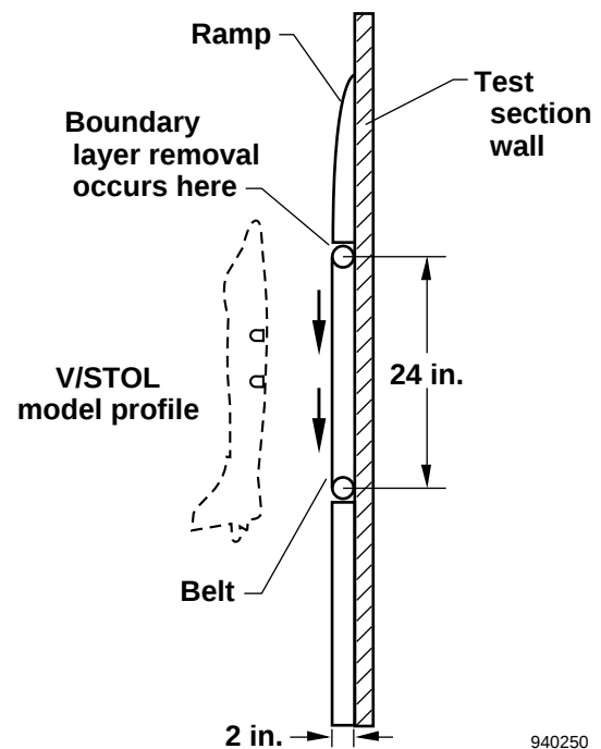
(a) Side view.
