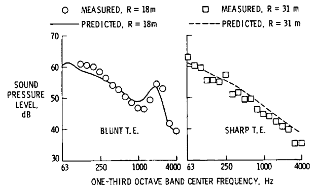
Figure 12. - Comparisons of measured and predicted broad band noise spectra for two different blade trailing edge configurations of the U.S. windpower inc. machine.
