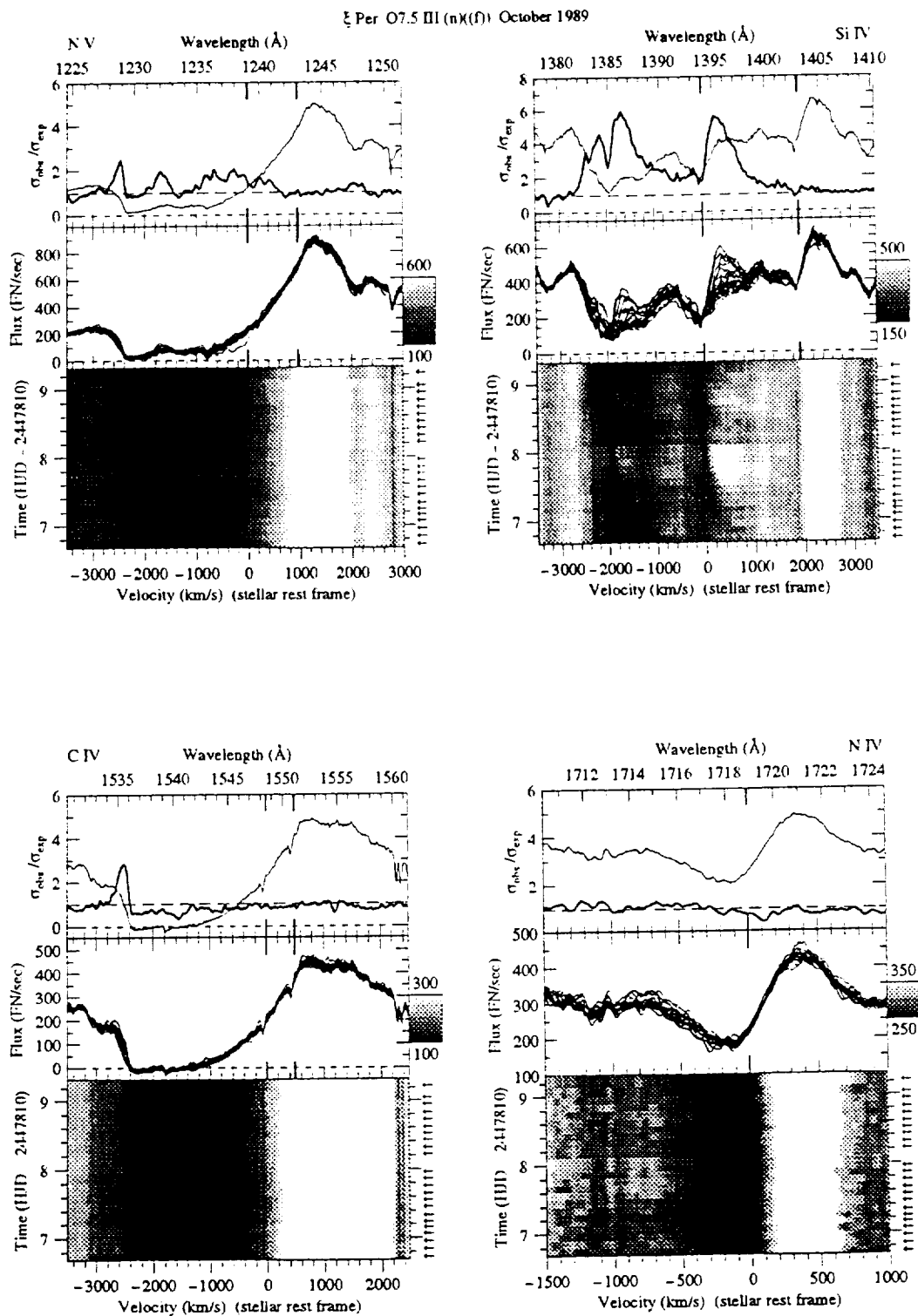
Fig. 3. As in Fig. 1: \xi Per October 1989, 23 spectra. These observations are described by Henrichs et al. (1994). Variations occur over the full range of wind velocities ( \sim -100 to -2750 \text{ km s}^{-1} ), from almost zero (in Si IV and N IV), to intermediate (in Si IV and N V) and the highest velocities (in N V and C IV). Note the "crossing" of DACs at about Day 8.1
