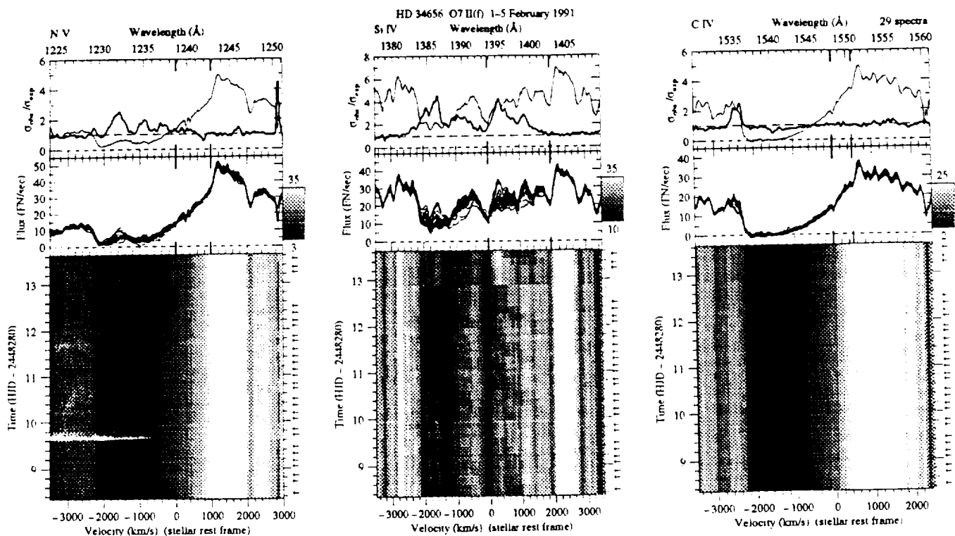
Fig. 6. As in Fig. 1: HD34656 O7 II(f) in February 1991. The Si IV line exhibits the migration of several DACs on a timescale of about 1 day. The detailed variability pattern is very complicated. Although the maximum velocity reached by these DACs is about -1900 \text{ km s}^{-1} , wind variability extends from almost zero to -2600 \text{ km s}^{-1} . The C IV edge varies around -2400 \text{ km s}^{-1} as reflected by the \sigma -ratio
