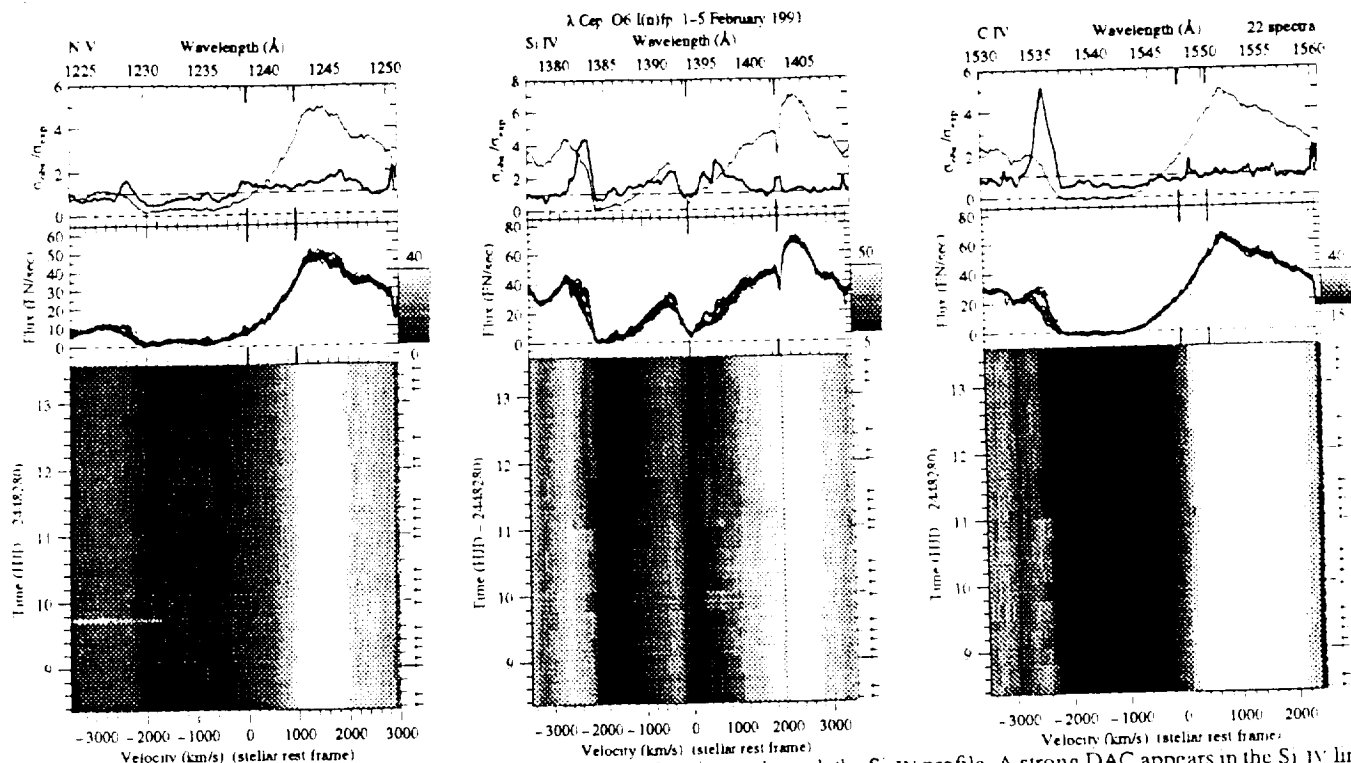
Fig. 24. As in Fig. 1: \lambda Cep O6 (n)fp in February 1991. Several DACs migrate through the Si IV profile. A strong DAC appears in the Si IV line at Day 11 while an evolved component (which appeared at Day 10) arrives at its asymptotic velocity of -2000 \text{ km s}^{-1} . During this occasion the C IV edge shifts more than 200 \text{ km s}^{-1} towards the blue. The amplitude of the edge variability in this dataset is the largest we encountered for \lambda Cep
