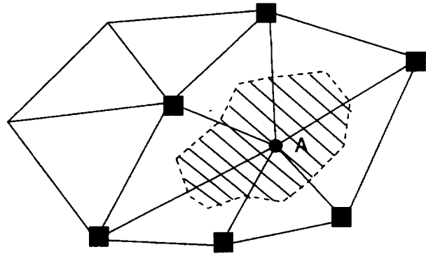
Figure 2: Control volume and stencil for a first order accurate cell-vertex scheme.
