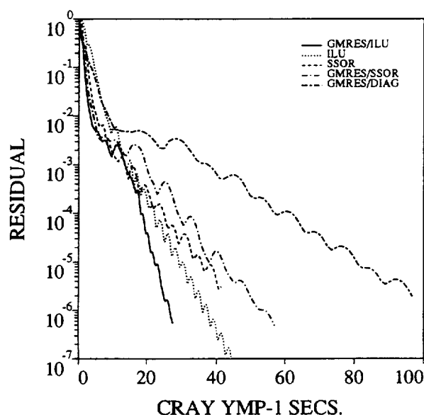
Figure 8: Convergence histories for inviscid flow over an NACA0012 airfoil ( M_\infty = 0.8 , \alpha = 1.25^\circ ).
