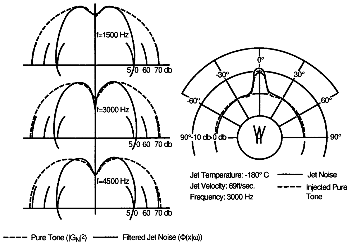
Fig. 2. Match of noise intensity patterns to indicate refraction-dominated zone. Left-hand side: room temperature jet ( M=0.5 ) with reduced intensity 'cone of silence' (rays turn outward); right-hand side; very cold jet ( -180^\circ\text{C} ) with enhanced intensity lobe (rays turn inward to a quasi-focus). (After ref. 29, based on refs. 32 and 33).
