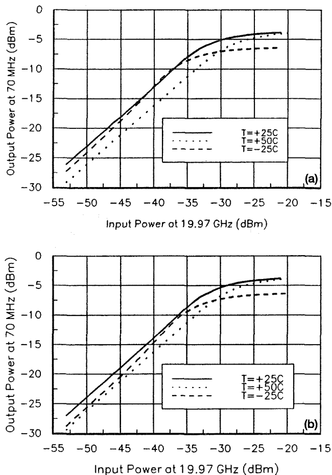
Figure 7.—Power transfer characteristics. (a) 9.90 GHz DRO sn141 at 12.98 dBm. (b) 9.95 GHz DRO sn137 at 13.04 dBm.
