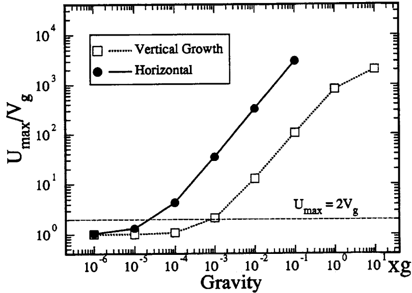
Figure 6. Effects of gravity on the strength of convection in the melt measured by the maximum total velocity, U_{\max} , which includes the growth rate V_g and the thermal buoyancy-driven convective velocity.
