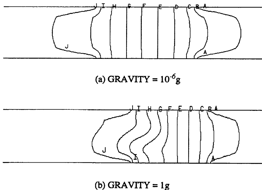
Figure 14. MEPHISTO 2 temperature contour plots for (a) 10^{-6}g and (b) 1g in the horizontal configuration. The temperature difference between isotherms is 47K.
