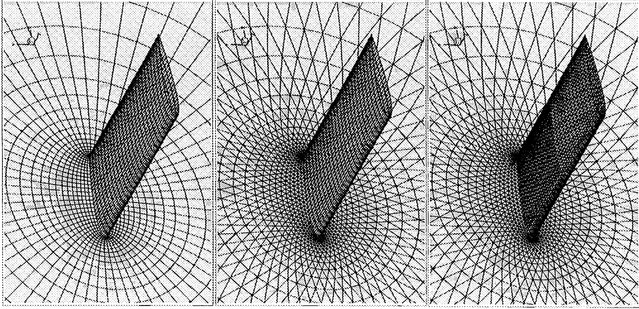
Figure 2: Hexahedral, Prismatic, and Tetrahedral Meshes about NACA 0012 Wing
