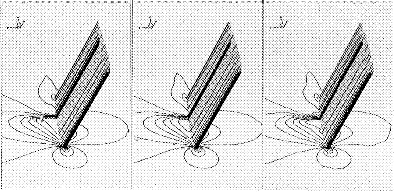
Figure 3: Computed Mach Contours for Flow over NACA0012 Wing on Hexahedral, Prismatic, and Tetrahedral Meshes
