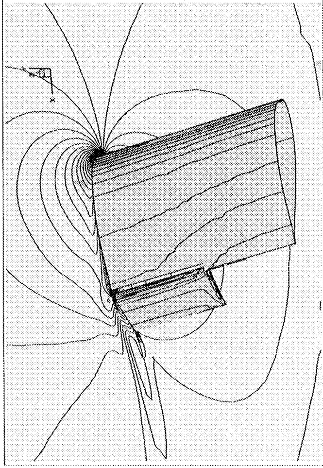
Figure 15: Computed solution displayed as Mach contours on wind-tunnel wall and pressure contours on airfoil surfaces for partial-span flap geometry
