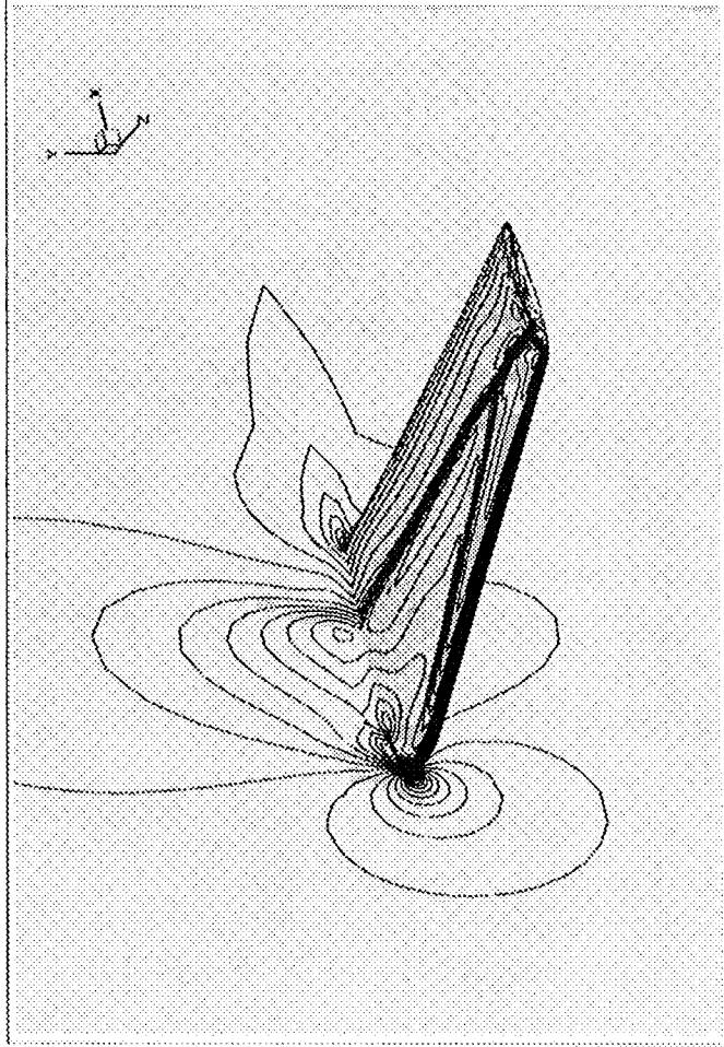
Figure 7: Computed Mach Contours on ONERA M6 Wing (Mach = 0.84, Incidence = 3.06 degrees)
