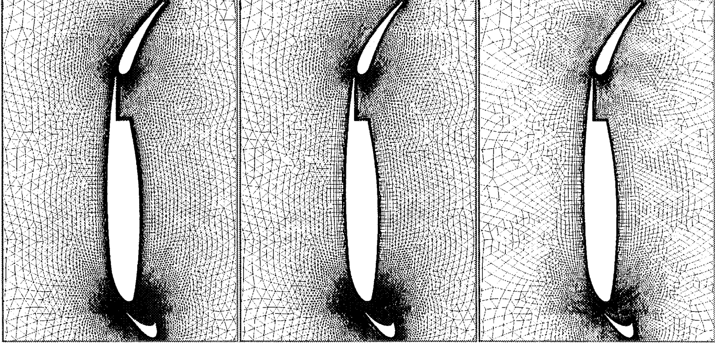
Figure 10: Fully triangular, partially, and fully merged meshes using two-dimensional mesh merging algorithm for three-element airfoil geometry
