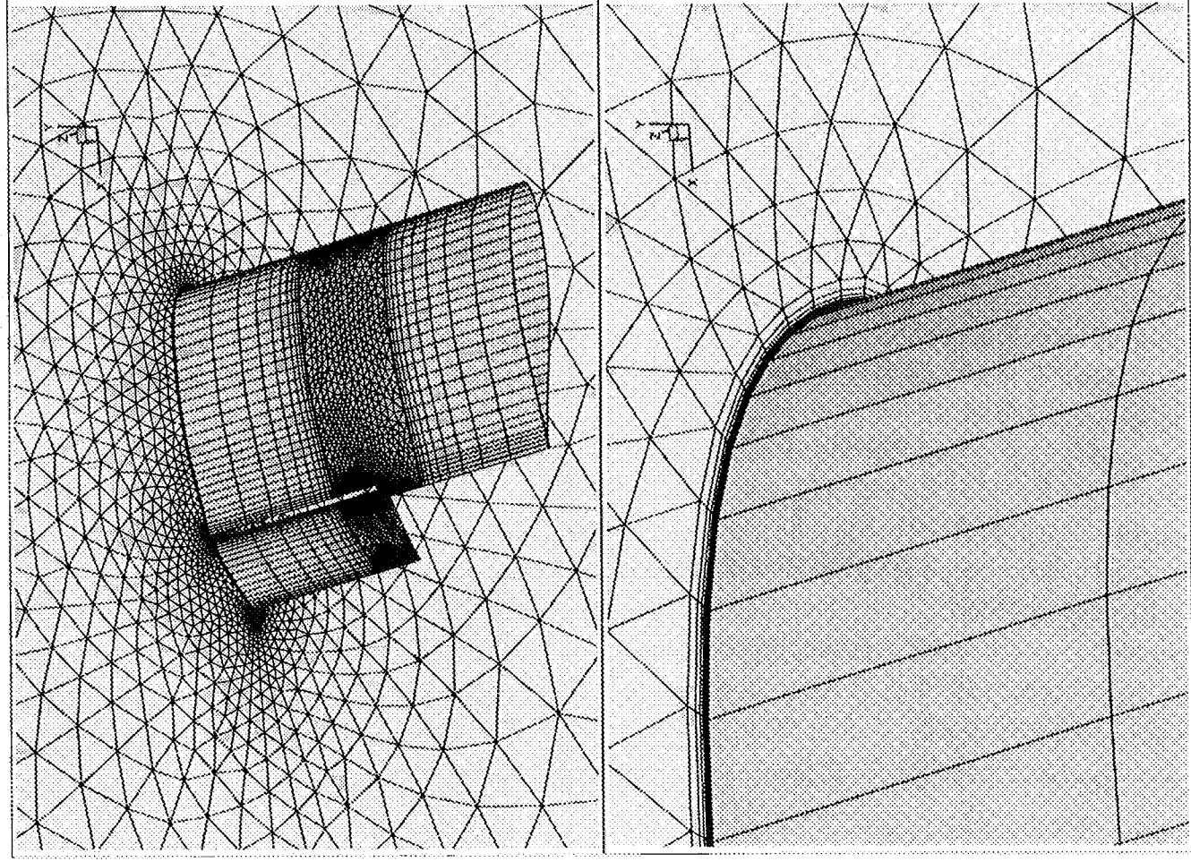
Figure 13: Mixed element mesh showing detail in near wall region for partial-span flap geometry
