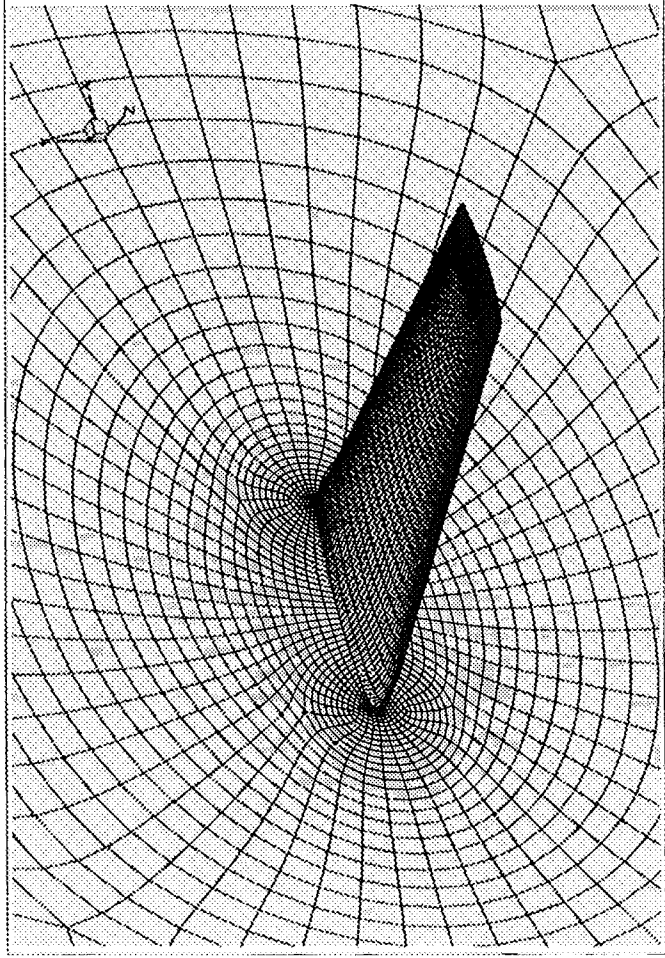
Figure 6: Block Structured Mesh about ONERA M6 Wing
