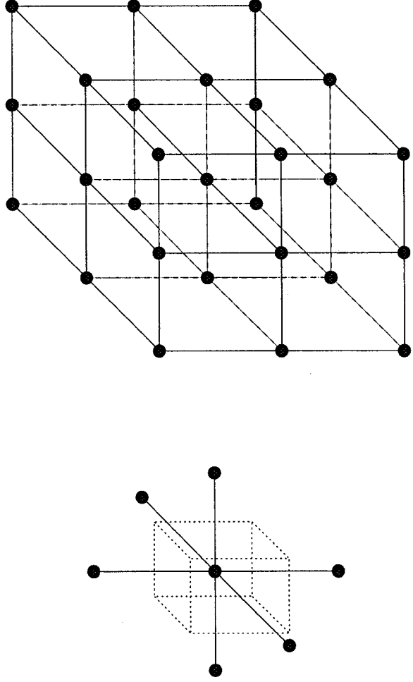
Figure 1: Illustration of 7 point finite-volume and 27 point finite-element stencil and associated control-volumes for hexahedral mesh
