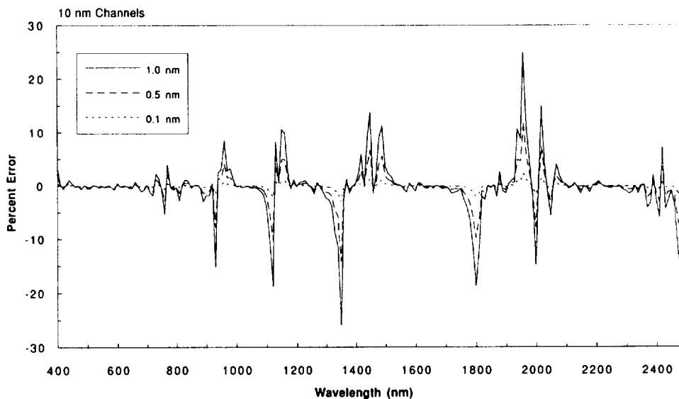
Figure 4. Error in AVIRIS modeled upwelling radiance with errors of 1.0, 0.5 and 0.1 nm in the calibration of channel center position.
