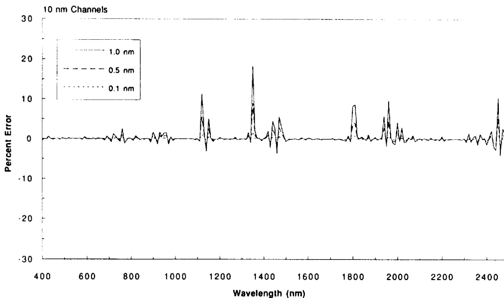
Figure 5. Error in modeled AVIRIS upwelling radiance with errors of 1.0, 0.5 and 0.1 nm in the calibration of channel FWHM.
