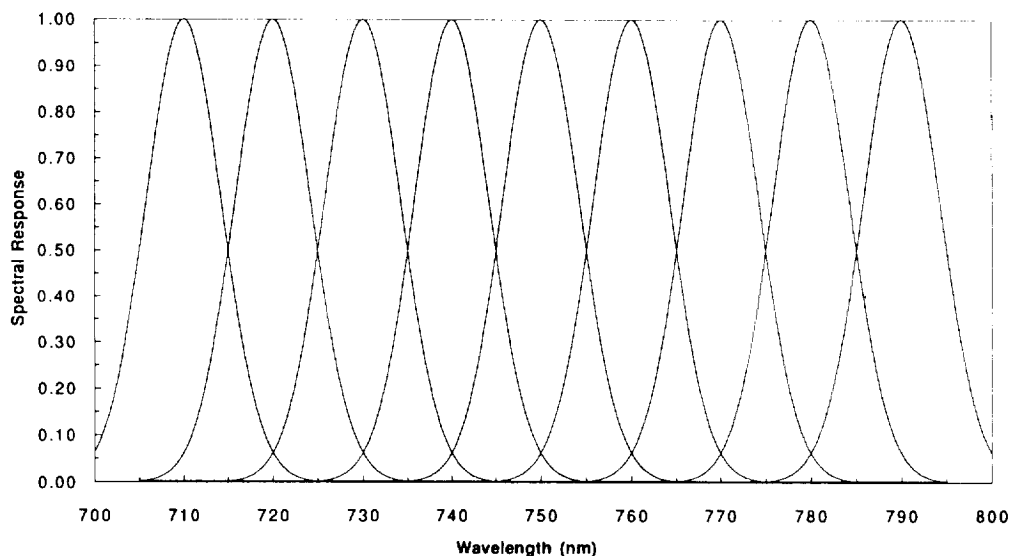
Figure 1. Modeled spectral response functions of 9 AVIRIS channels.
