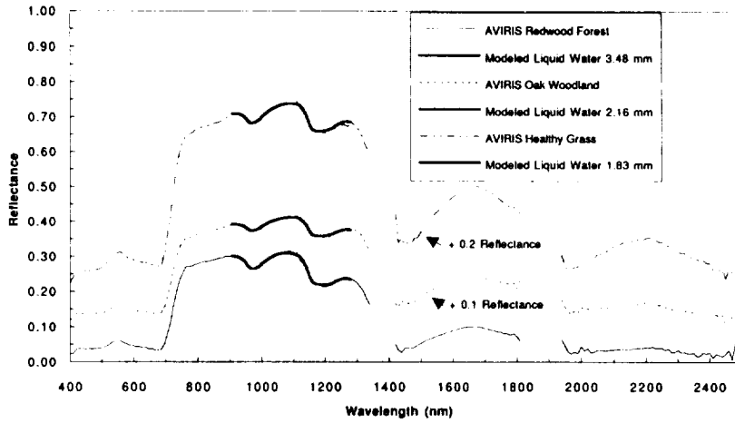
Figure 2. Equivalent path transmittance leaf water for healthy grass, oak woodland, and redwood forest in the 1000-nm spectral region.
