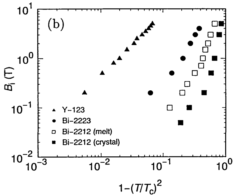
Fig. 1. (a) Calculated irreversibility lines and (b) observed irreversibility lines for melt-processed Y-123 (▲), silver-sheathed Bi-2223 tape wire (●), melt-processed Bi-2212 (□) and TSFZ-processed Bi-2212 single crystal (■).
