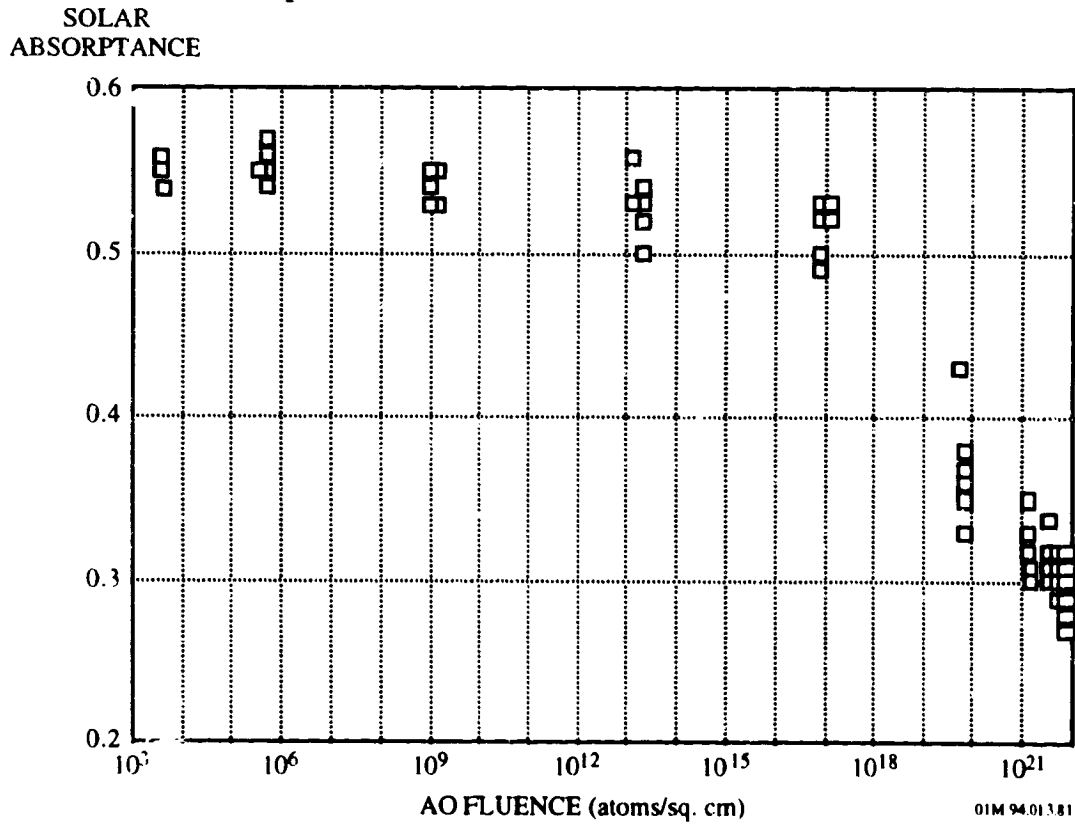
Figure 10-10. Solar Absorbance For A276 White Paint Disks Versus Atomic Oxygen Fluence
