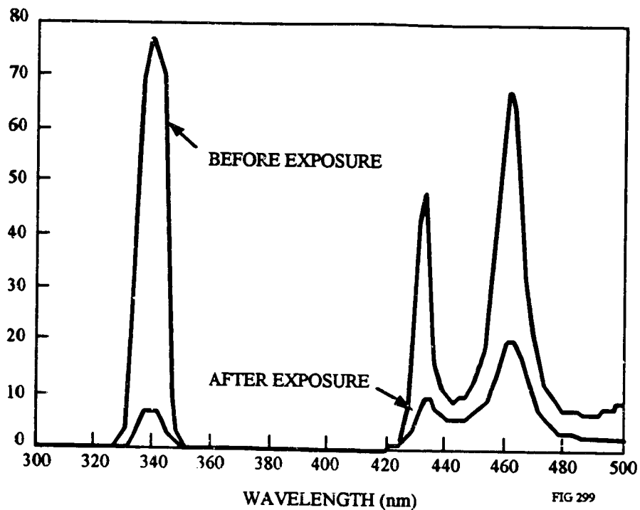
Figure 12-33. Pre-Launch and Post-Recovery Transmission of PbF 2 /Cryolite on Fused Silica (air-spaced, no cement)
