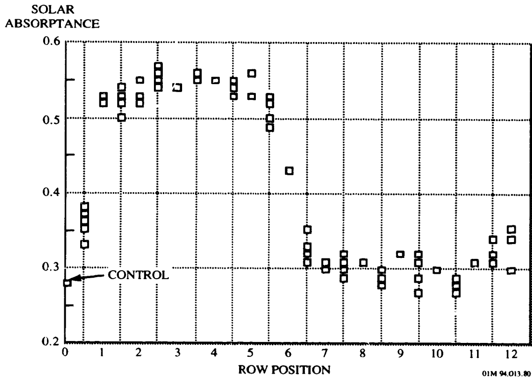
Figure 10-9. Solar Absorbance For A276 White Paint Disks Versus LDEF Row Position
