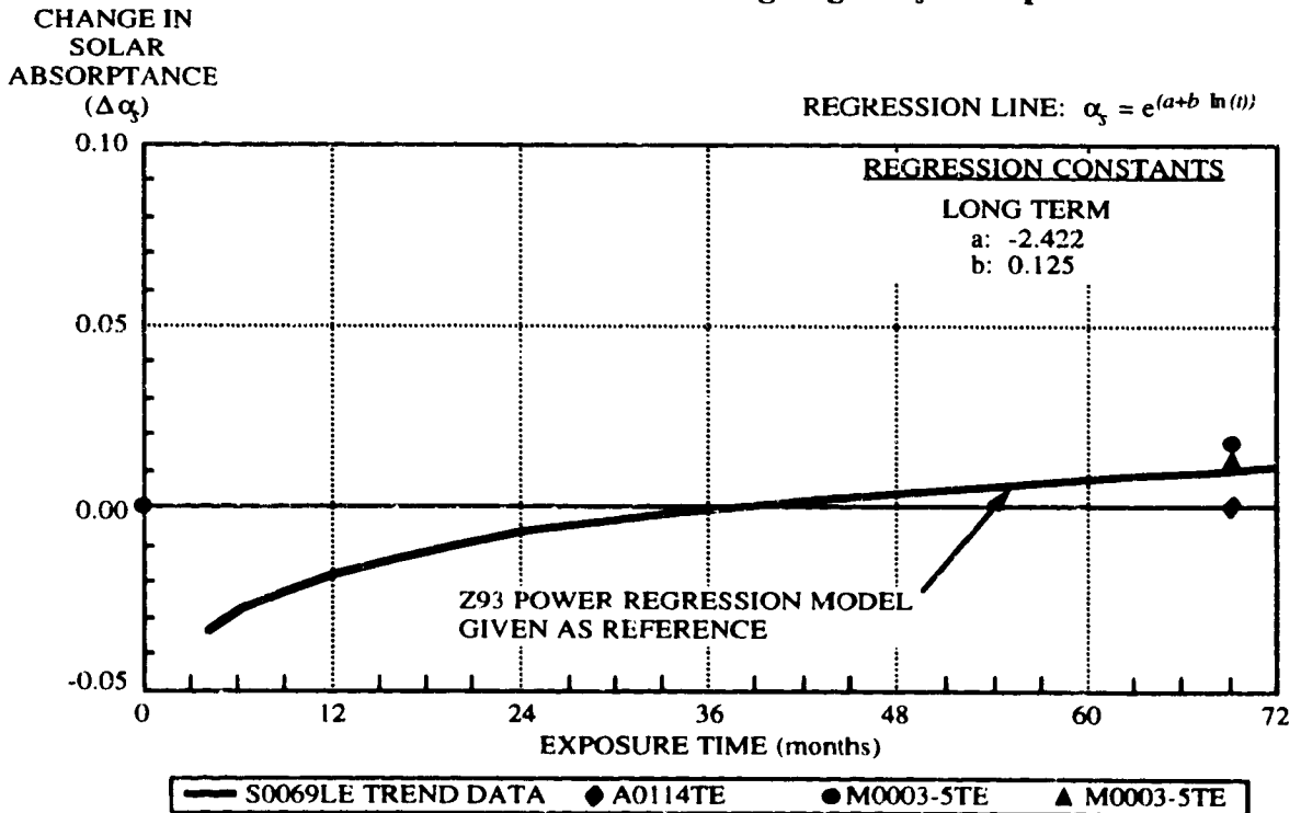
Figure 10-20. Performance of Z-93 on LDEF - Leading Edge \Delta\alpha , vs. Exposure Time
