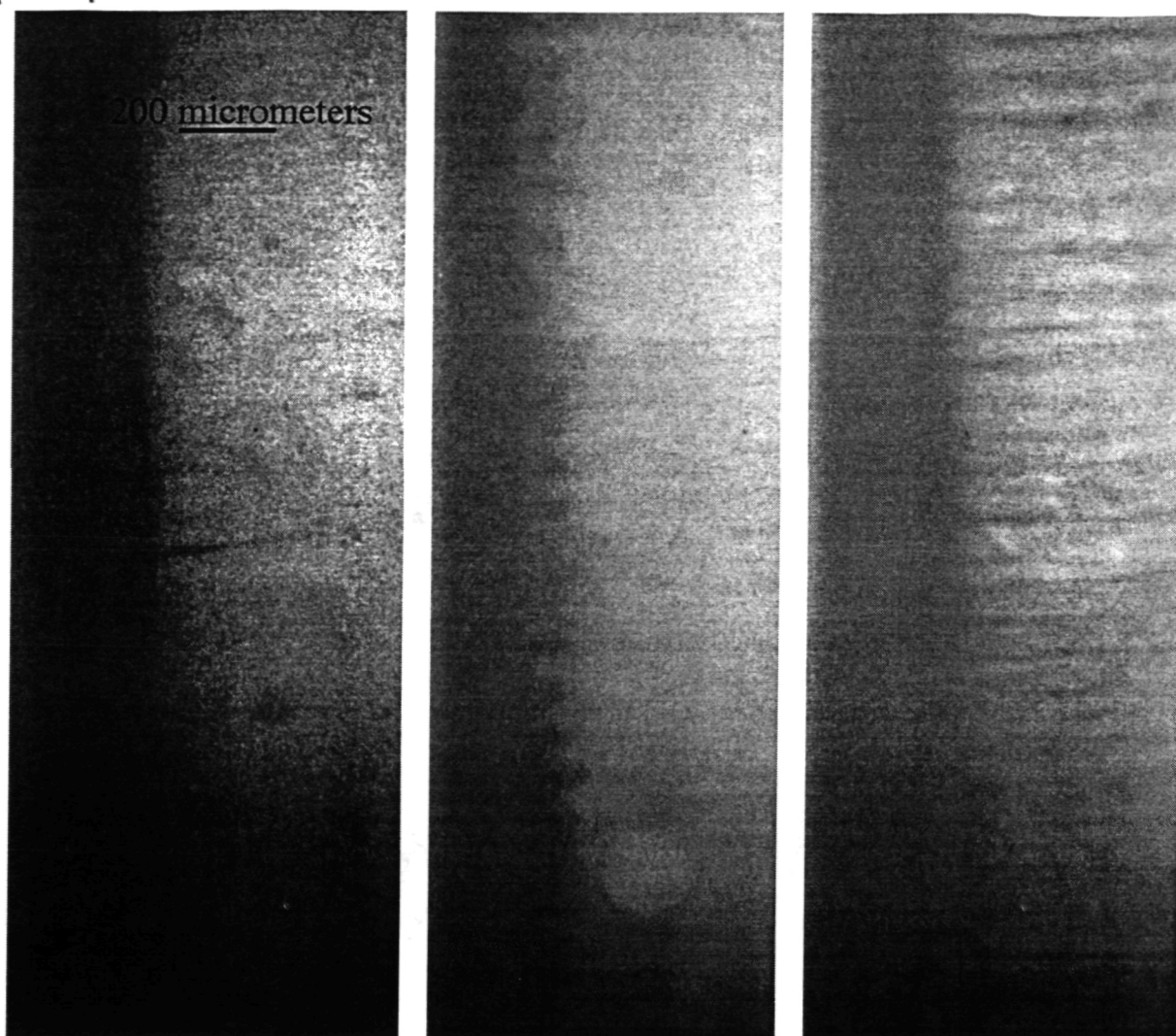
Figure 3. Al 2% Ag interfaces. Each are 2 second exposures at 55 kV acceleration and 200 \mu A current. Left figure shows planar interface growing at 1 \mu m/sec; grain boundaries intersect the interface isotherm. Middle figure captures the initial stages of cellular breakdown after the rate was increased to 2 \mu m/sec from 1.5 \mu m/sec; void was engulfed in lower segment. The right figure shows the steady state cellular growth at 2 \mu m/sec.
