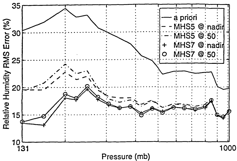
Figure 2: Comparison of cloudy retrieval accuracy over ocean.
