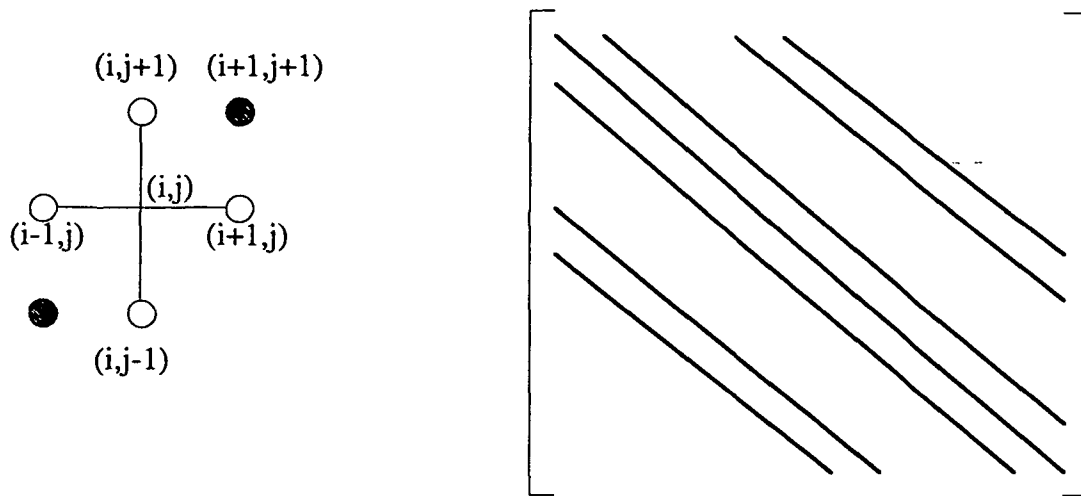
Figure 5. Modified stencil and the resulting matrix.
