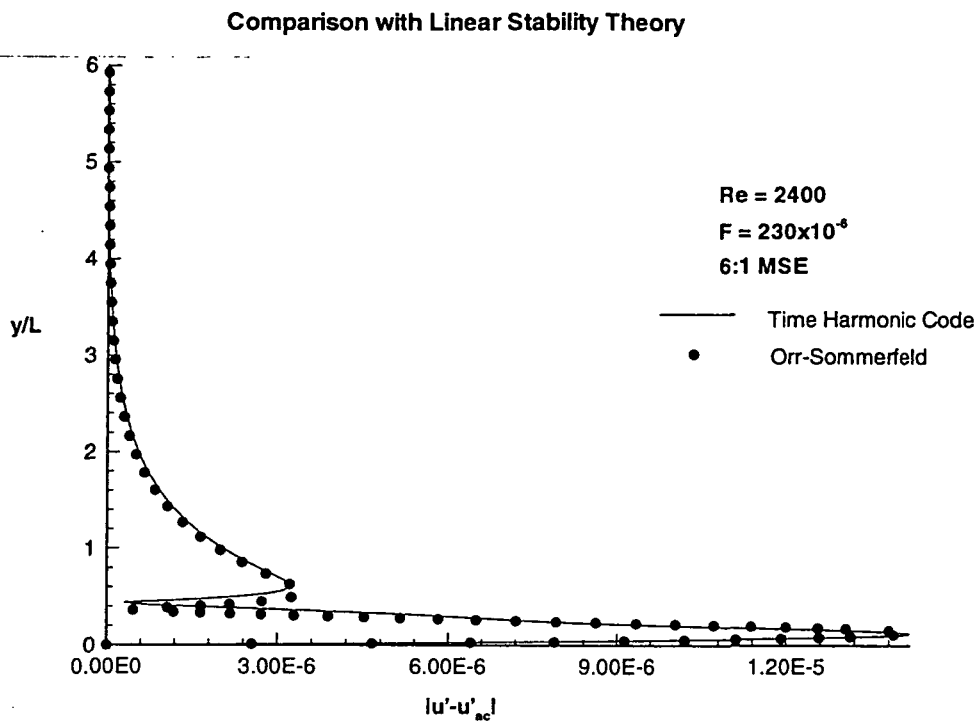
Figure 1. Comparison of TS eigenmodes from time-harmonic code and linear stability theory. The forcing amplitude was 1 \times 10^{-3} .
