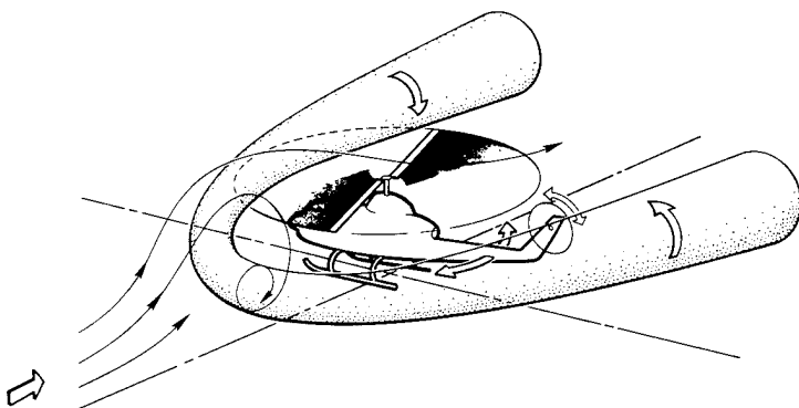
Fig. 19 Main rotor/tail rotor interaction in side wind, with horseshoe ground vortex [47]
