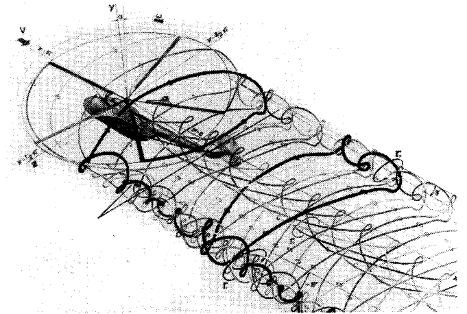
Fig. 2. Vortical wake of a helicopter in forward flight [1].
