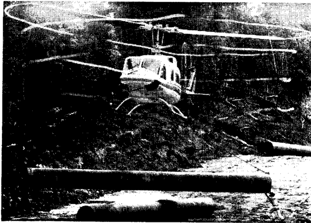
a). visualization by condensation of water vapor in the atmosphere [6]
