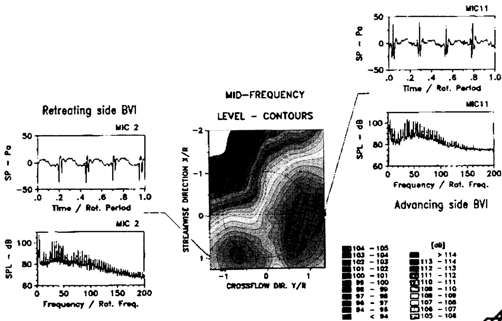
Fig. 25 BVI impulsive noise characteristics for the same conditions as Fig. 24
