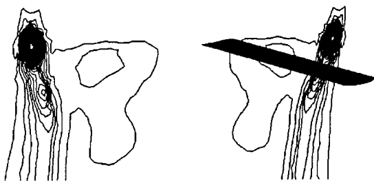
Fig. 14 Solution-adapted unstructured grid and vorticity contours at the boundaries
