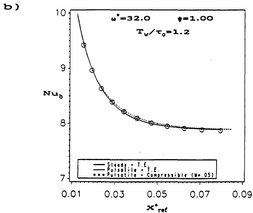
Figure 4.2.10: Comparison of the time-averaged Nusselt number in the channel between thermally expandable and compressible predictions ( Re_{\text{mean}} = 2000 , air, T_w/\tau_0 = 1.2 , \psi = 1.00 ): a) \omega^* = 0.08 [PT-1, PC-1]. b) \omega^* = 32.0 [PT-3, PC-2].
