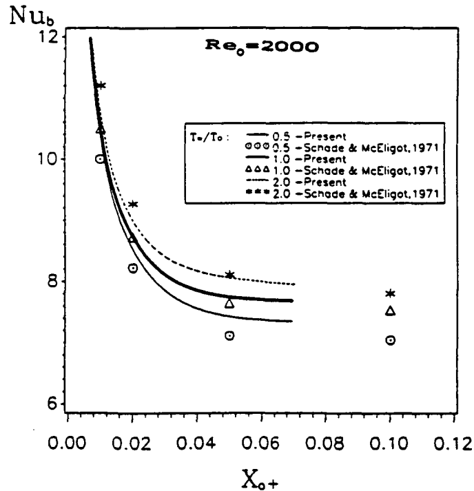
Figure 4.1.7: Local Nusselt number comparison of steady flow in the channel with data from Schade & McEligot [1971] at different wall/inlet temperature ratios, T_w/T_o=1.0 (incompressible), 0.5 and 2.0 (thermally expandable): a) Re_0=144 [SI-4, ST-1, ST-2]. b) Re_0=2000 [SI-5, ST-4, ST-9].
