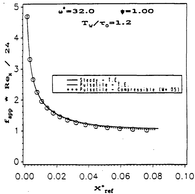
Figure 4.2.6: Comparison of the time-averaged local apparent friction in the channel between thermally expandable and compressible predictions ( Re_{mean} = 2000 , air, T_w / \tau_0 = 1.2 , \psi = 1.00 ): a) \omega^+ = 0.08 [PT-1, PC-1]. b) \omega^+ = 32.0 [PT-3, PC-2].
