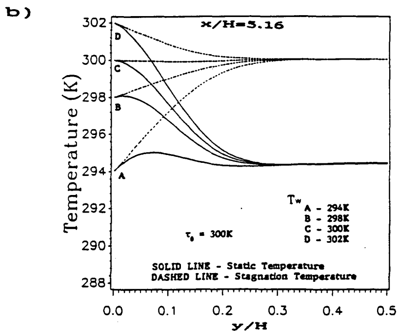
Figure 4.1.8: Comparison between static and stagnation temperature distribution in the channel at high-velocity ( M=25 ) steady flow for a fluid with Pr=1.0 [SC-1 to SC-4]: a) x/H=1.10 . b) x/H=5.16 .
