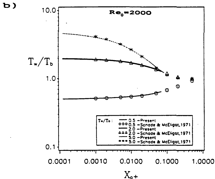
Figure 4.1.6: Ratio of wall and bulk-mean temperature comparison in the channel with data from Schade & McEligot [1971] at different wall/inlet temperature ratios, T_w/T_o = 0.5, 2.0, 5.0 (thermally expandable): a) Re_o = 144 [ST-1, ST-2, ST-3]. b) Re_o = 2000 [ST-4, ST-9, ST-10].
