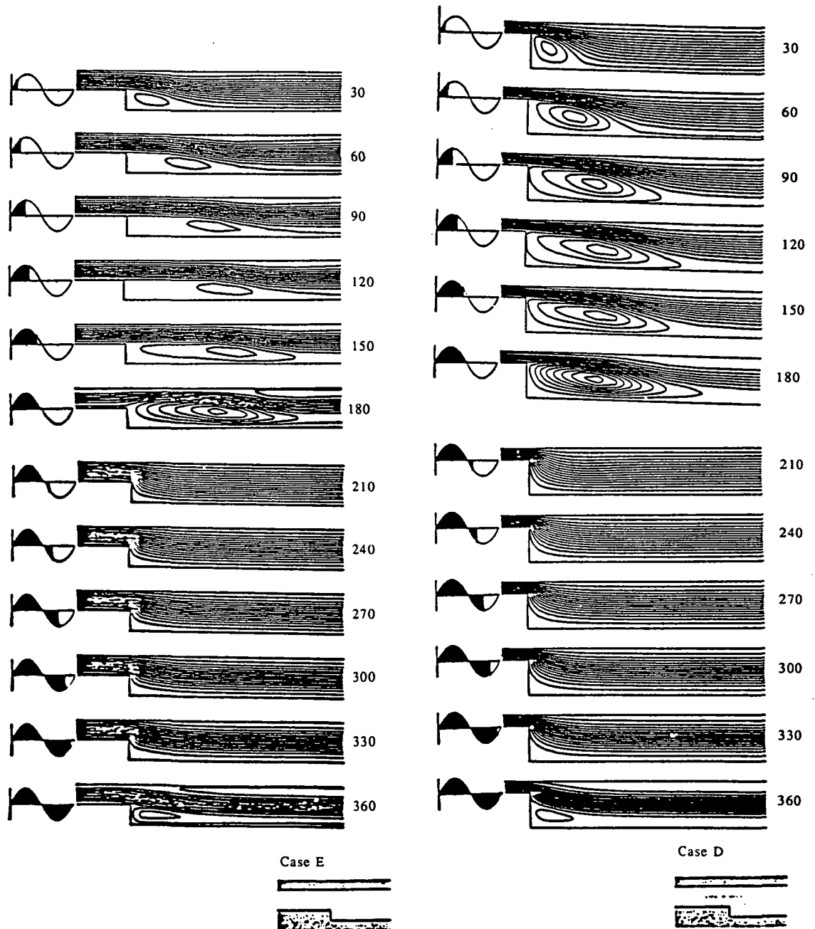
Fig. 8. Streamlines of oscillating flow at different velocity phase angles, for Re_{max} = 1000 and Va = 5.33 (Case E, asymmetric expansion/contraction with a ratio of 1:2.)
