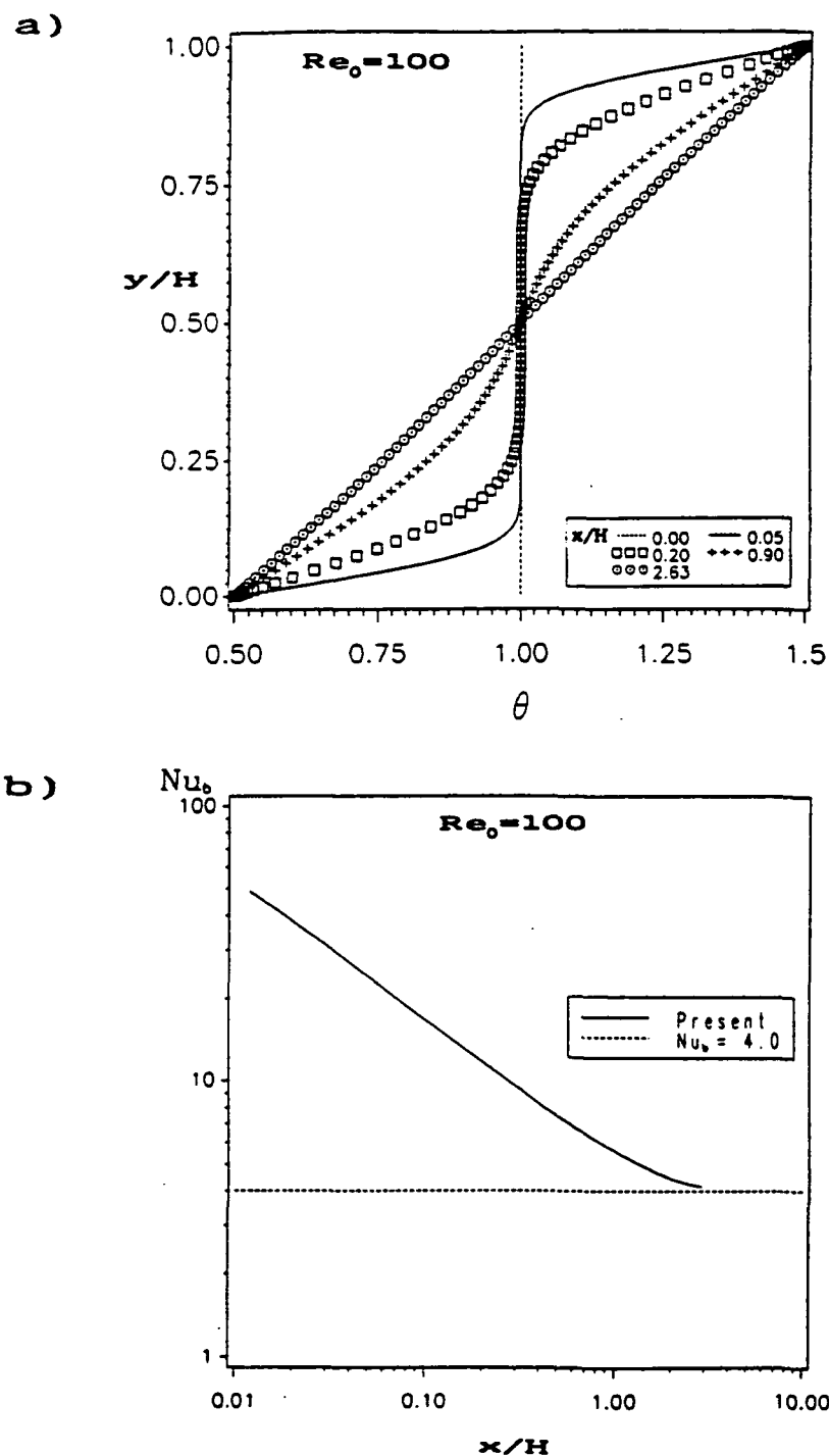
Figure 4.1.4: Heat Transfer in simultaneously developing, steady flow with different but constant wall temperatures at Re_0=100 [SI-3]: a) Temperature profiles at different developing axial locations. b) Comparison of the present developing local Nusselt number with the theoretical, fully-developed value ( Nu_b=4.0 ).
