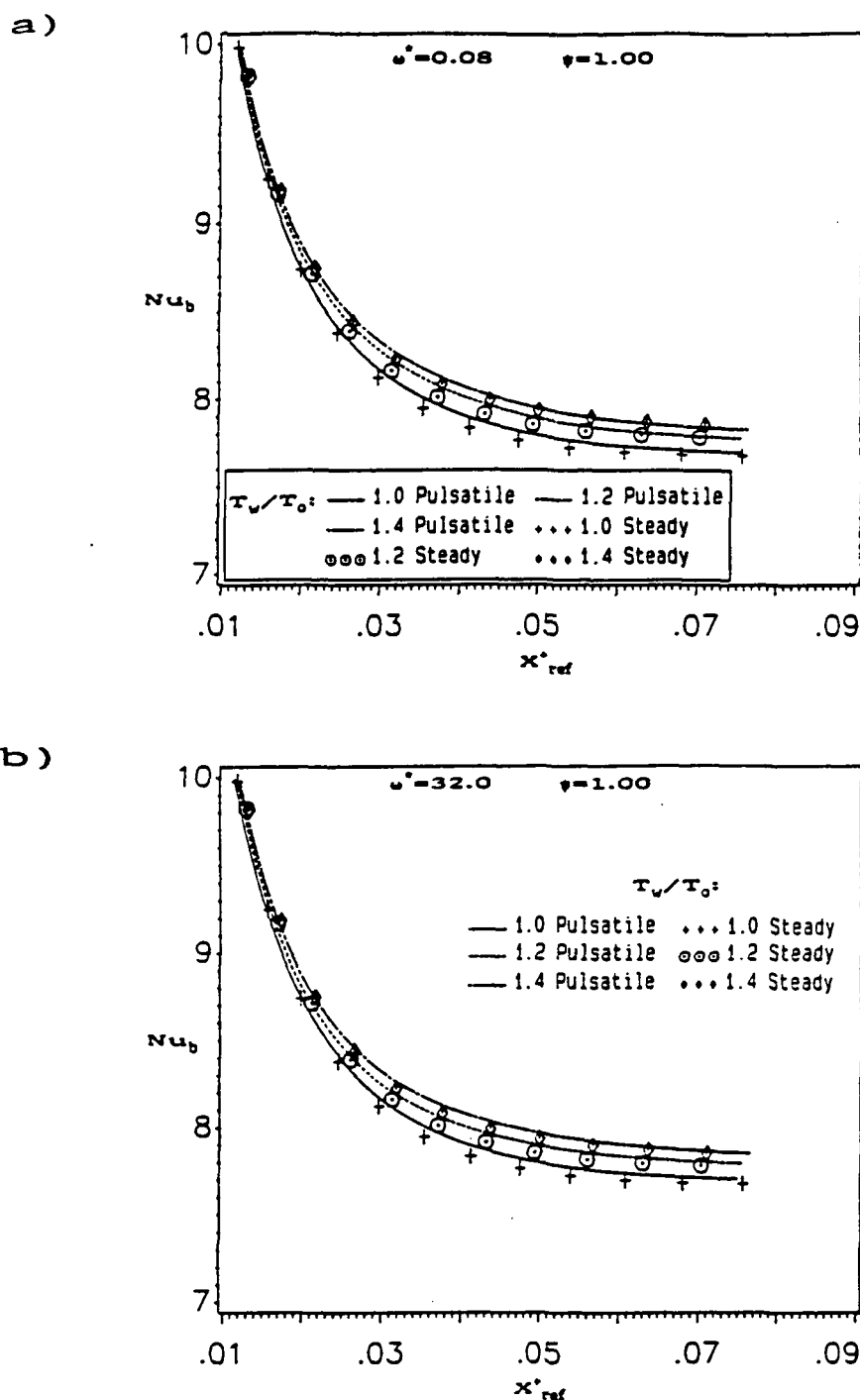
Figure 4.2.9: Time-averaged Nusselt number in the channel at different wall/inlet temperature ratios: T_w/T_0 = 1.0 (incompressible), 1.2 and 1.4 (thermally expandable); ( Re_{2020} = 2000 , Pr = 0.72 , \psi = 1.00 ): a) \omega^* = 0.08 [PI-5, PT-1, PT-2]. b) \omega^* = 32.0 [PI-6, PT-3, PT-4].
