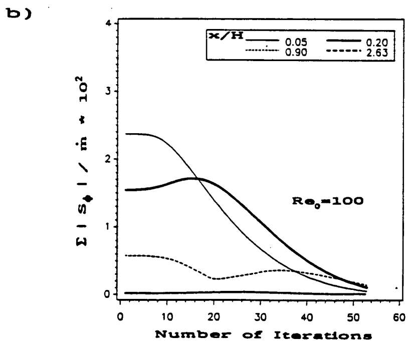
Figure 4.1.1: Convergence characteristics for incompressible, steady flow at: a) Re_0 = 40 [SI-1]. b) Re_0 = 100 [SI-2].
