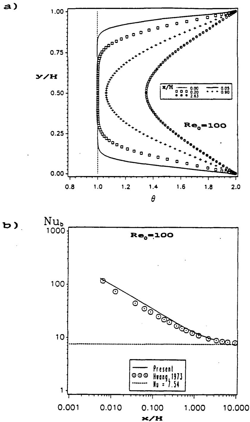
Figure 4.1.3: Heat Transfer in simultaneously developing, steady flow with equal and constant wall temperatures at Re_0 = 100 [SI-2]: a) Temperature profiles at different developing axial locations. b) Comparison of the present average heat transfer coefficient with data from Hwang [1973].
