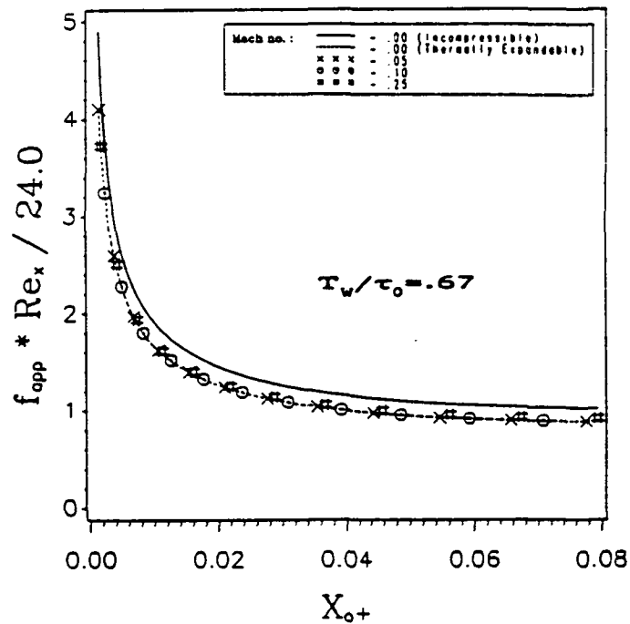
Figure 4.1.9: Comparison of steady local apparent friction in the channel at different Mach numbers, M=0.0 (incompressible), 0.0 (thermally expandable), .05 , .10 and .25 (compressible): a) T_w/\tau_0=1.5 [SI-8, ST-8, SC-8, SC-9, SC-10]. b) T_w/\tau_0=0.67 [SI-6, ST-5, SC-5, SC-6, SC-7].
