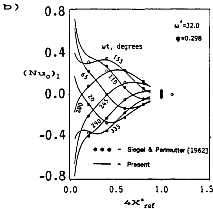
Figure 4.2.3: Nusselt number variation in the channel compared between present work and data from Siegel & Perlmutter [1962] (incompressible with pulsating slug flow approximation, Re_{mean} = 2000 , Pr = 0.72 ): a) Instantaneous Nusselt number, \omega^+ = 0.08 , \psi = 1.00 [PI-1]. b) Fluctuating component of the Nusselt number, \omega^+ = 32.0 , \psi = 0.298 [PI-3].
