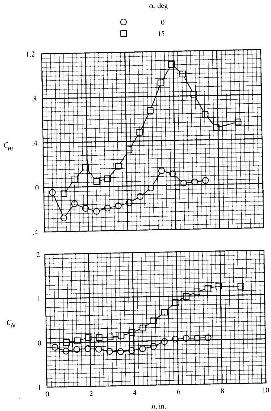
(c) Separation characteristics of cone cylinder.
