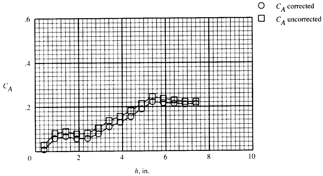
(a) Cone cylinder at \alpha = 0^\circ .
