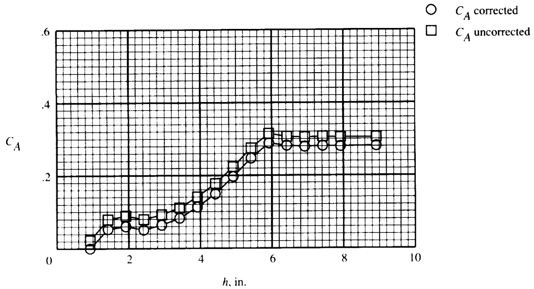
(b) Cone cylinder at \alpha = 15^\circ .
