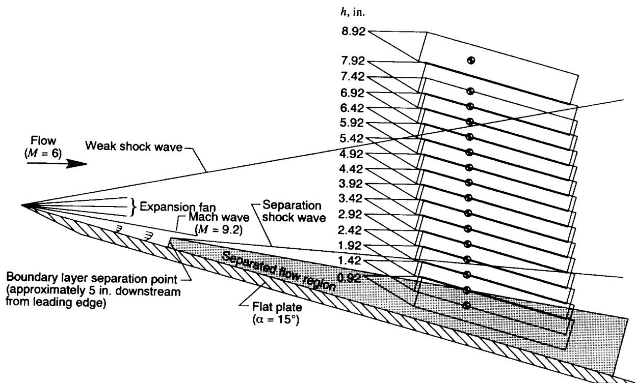
(b) Positions of cone cylinder at \alpha = 15^\circ .
