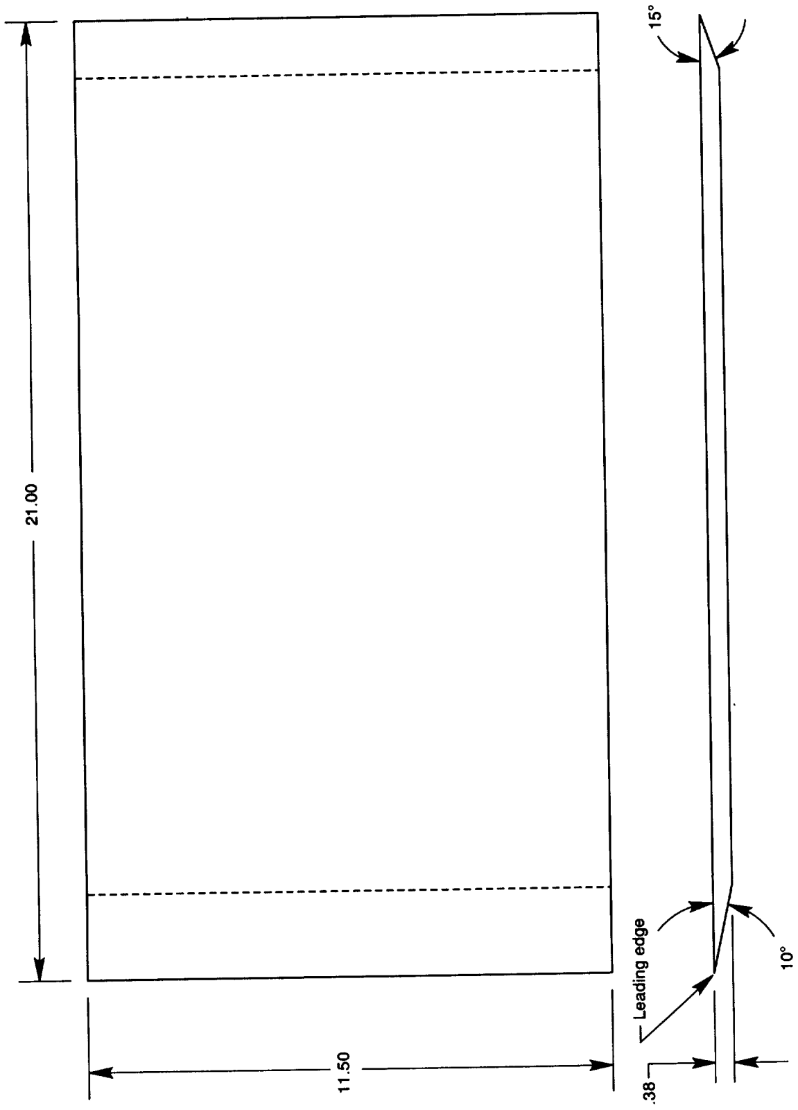
(c) Sketch of flat plate. All linear dimensions are in inches.
