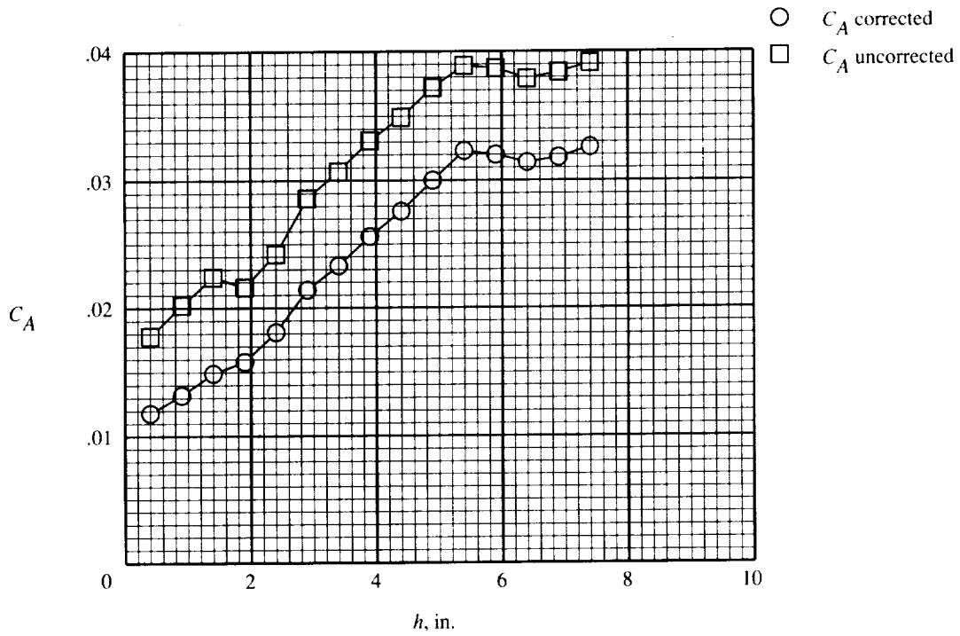
(c) Roof delta at \alpha = 0^\circ .
