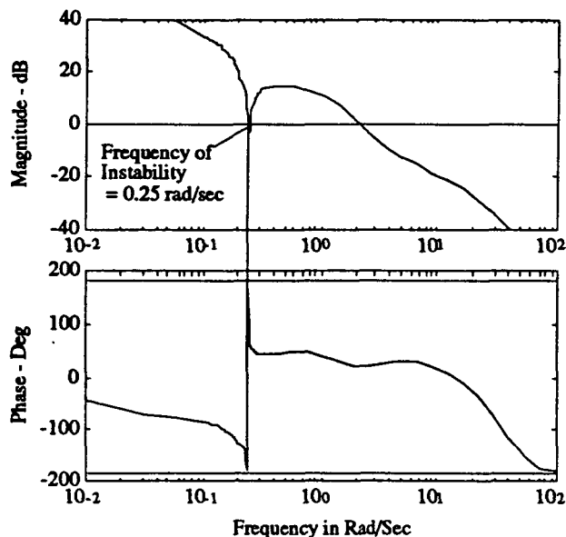
Figure 11 - Engine Loop Transfer - Increased Gains on Decentralized Control Cause Instability
