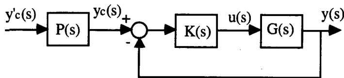
Figure 1 - The Feedback System With Pre-Filter
