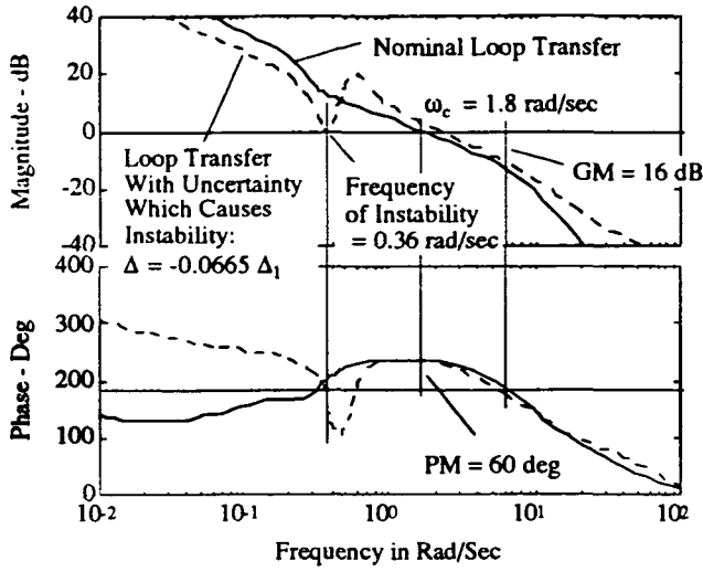
Figure 17 - Pitch Attitude Loop Transfer Function
