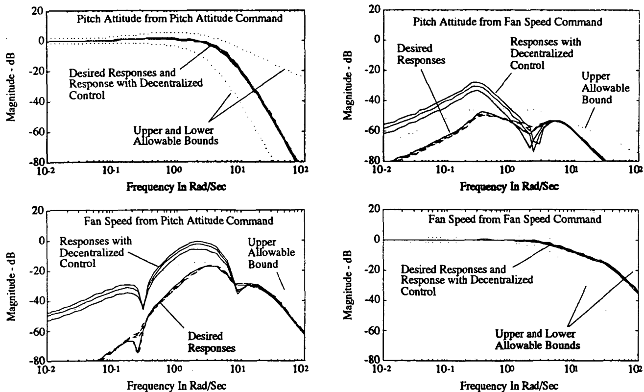
Figure 9 - Closed-Loop Frequency Response Magnitudes with Plant Uncertainty
