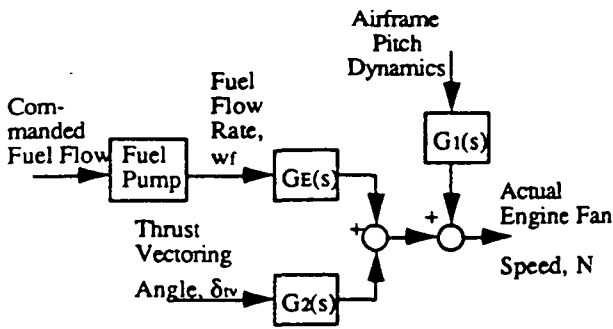
Figure 9 - Block Diagram of the Engine Influenced By the Airframe
