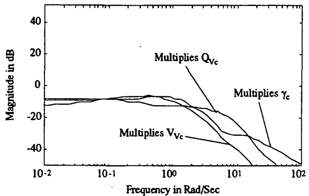
Figure 16 - Frequency Response Magnitudes Of D_A(j\omega)
