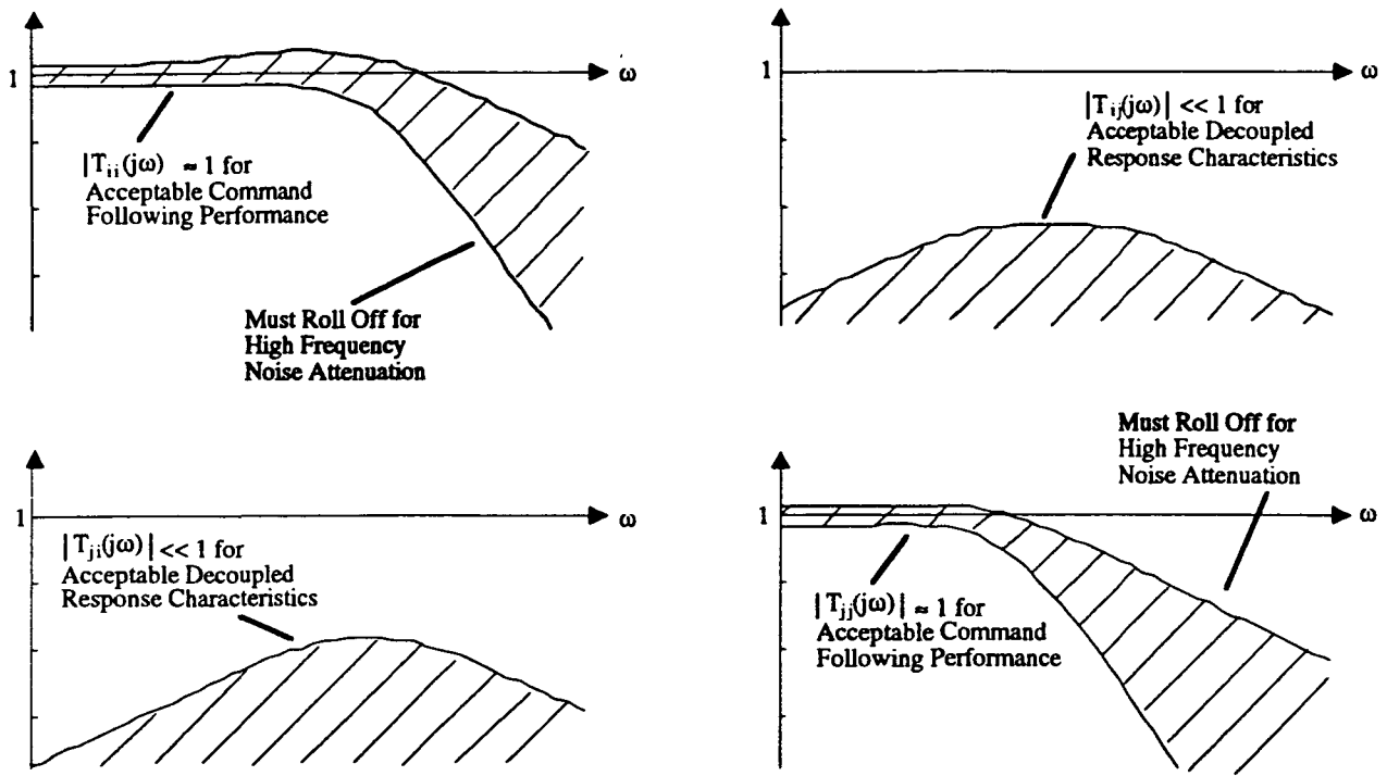
Figure 2 - Example Defined Upper and Lower Bounds on Closed-Loop Responses for Acceptable Performance
