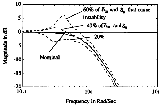
Figure 19 - Closed Loop Flight Path Angle Response From Flight Path Angle Command
