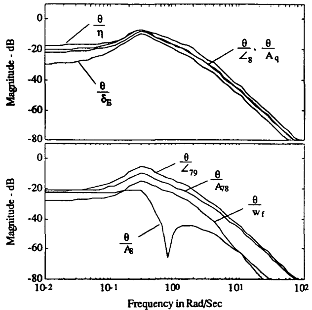
Figure 4 - Pitch Attitude Frequency Response Magnitudes
