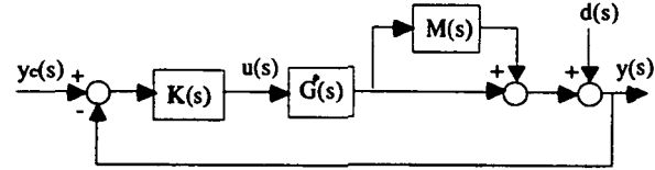
Figure 7 - Feedback System With Uncertainty, M(s)
