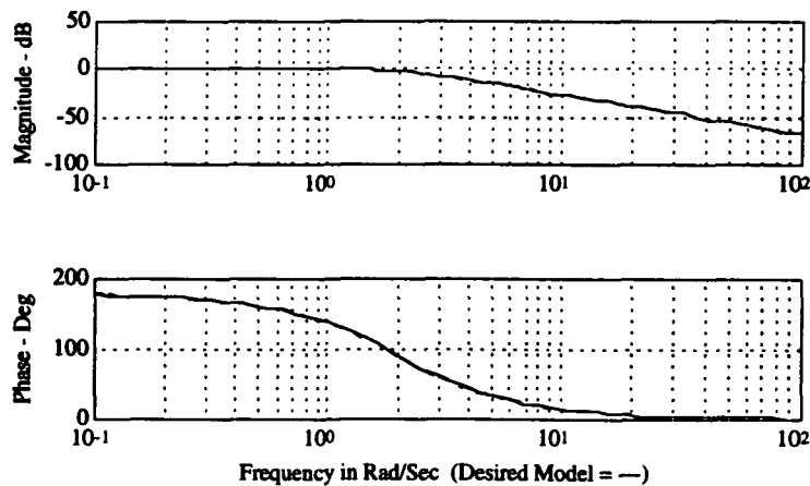
Figure 8.1 - Closed Loop Frequency Response of Angle of Attack from Pilot Stick Input (Deg/lbs)
