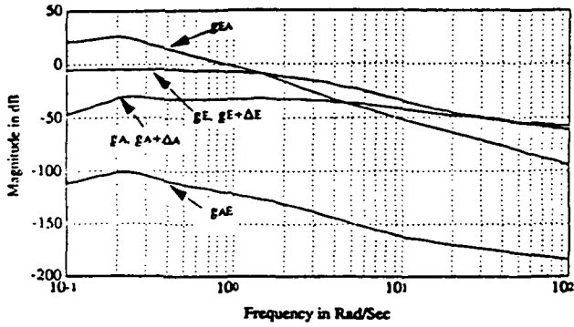
Figure 16 - Open Loop Transfer Function Magnitudes
