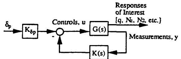
Figure 1 - Block Diagram of the Feedback Control Structure
