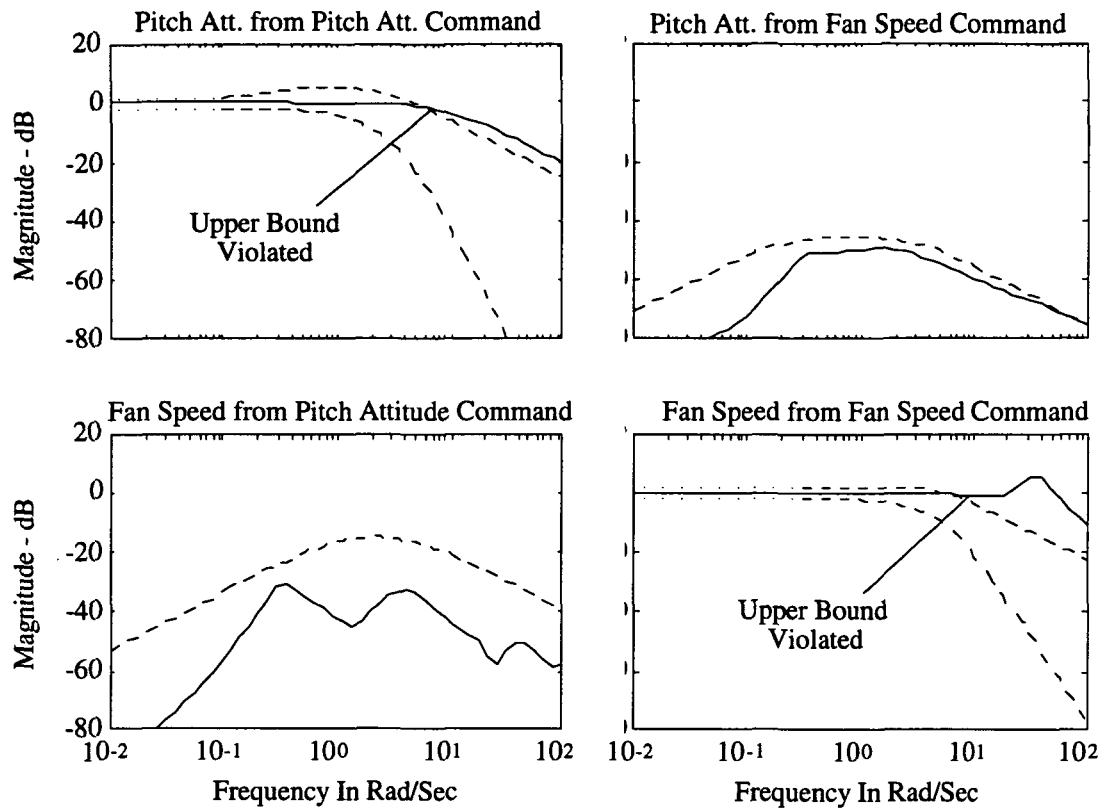
Figure 2 - Closed-Loop Frequency Response Magnitudes - Diagonal Elements of T(j\omega) Unacceptably Large At Higher Frequencies For Decentralized Control
