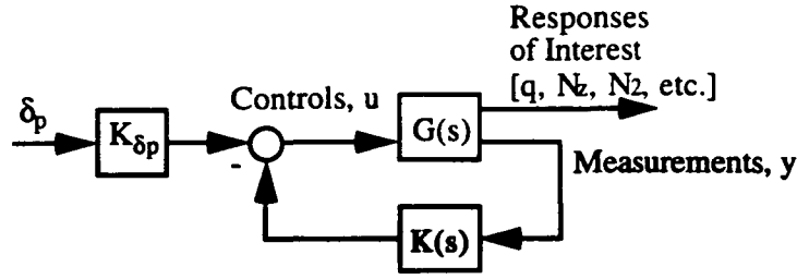
Figure 5.1 - Block Diagram of the Feedback Control Structure
