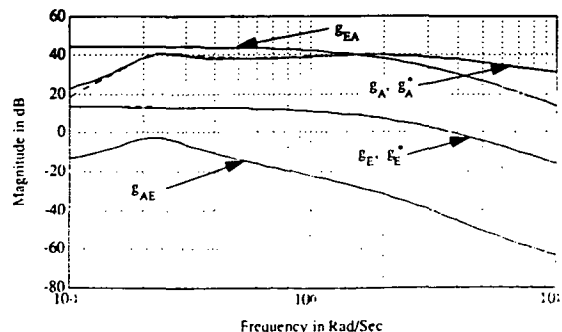
Fig. 12 Open-loop normalized transfer function magnitudes with pitch RCS control included.
