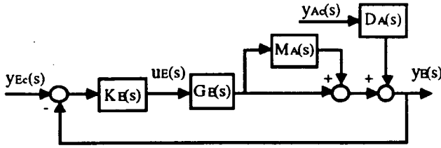
Figure 14 - Engine Loop With Effects From Airframe
