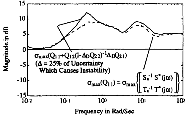
Figure 13 - Performance Robustness Criterion of Eq. (23)
