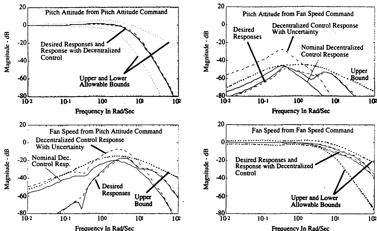
Figure 7 - Closed-Loop Frequency Response Magnitudes with Plant Uncertainty - Pre-Filter Utilized in Decentralized Control
