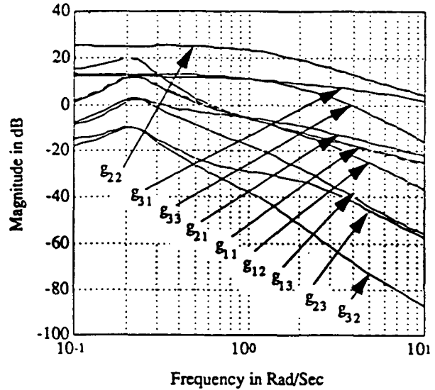
Figure 4.1 - Open Loop Normalized Input/Output Mappings
