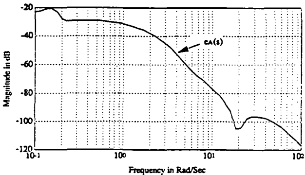
Figure 20 - Magnitude of the e_A(s) Transfer Function
