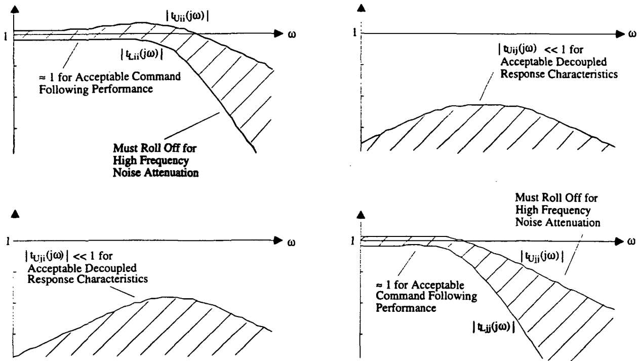
Figure 2 - Example Defined Upper and Lower Bounds on Closed-Loop Responses for Acceptable Performance
