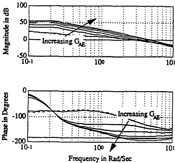
Figure 4.4 - Nominal and Coupled System's Engine Loop Transfer Frequency Responses
