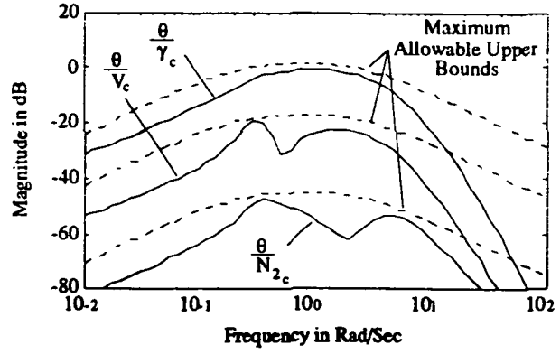
Figure 6 - Pitch Attitude From Other Commands
