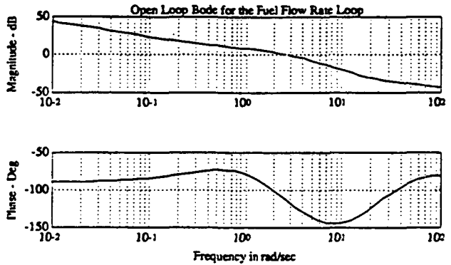
Figure 15 - Fuel Flow Rate Loop Transfer Frequency Response
