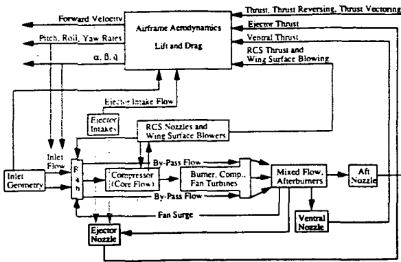
Fig. 2 Example interactions between airframe and engine subsystems.
