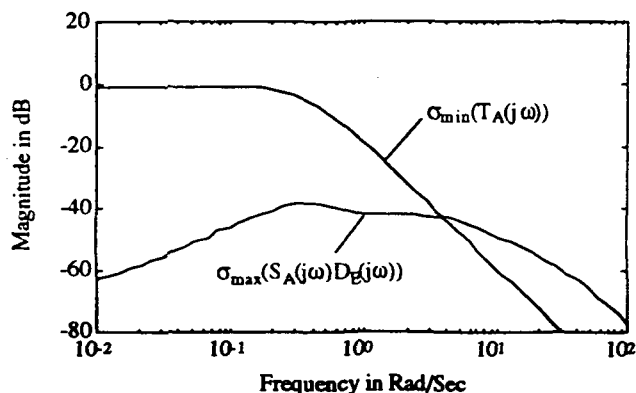
Figure 22 - A "Worst Case" Measure of the Effects of Engine Commands On Airframe Responses
