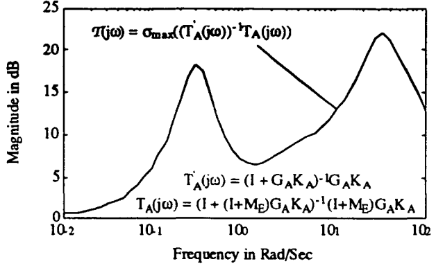
Figure 20 - Performance Robustness Measure - \pi(j\omega)
