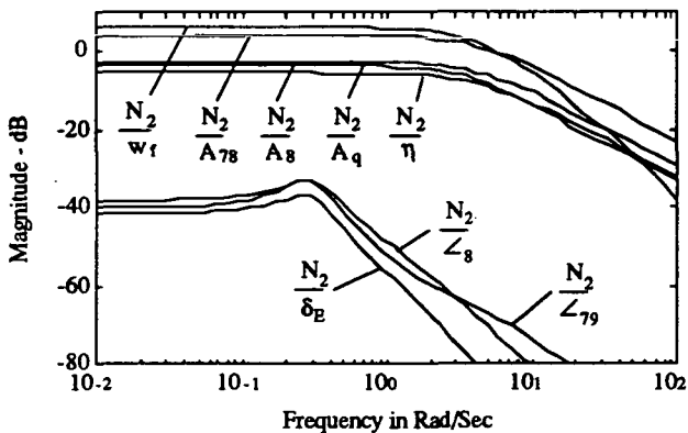
Figure 3 - Engine Fan Speed Frequency Response Magnitudes
