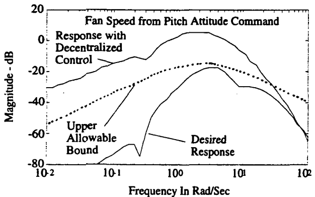
Figure 6 - Closed-Loop Frequency Response Magnitudes - All Elements of T_{AE}(j\omega) , T_{EA}(j\omega) Unacceptably Large For Decentralized Control
