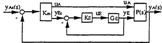
Figure 6.2 - Airframe/Engine System Framework With Engine System Explicitly Shown
