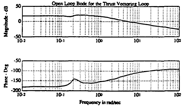
Figure 14 - Thrust Vectoring Loop Transfer Frequency Response
