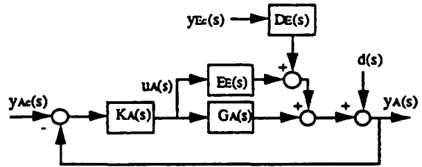
Figure 2.3 - Block Diagram of the Airframe Feedback Loop for the Coupled Airframe/Engine System
