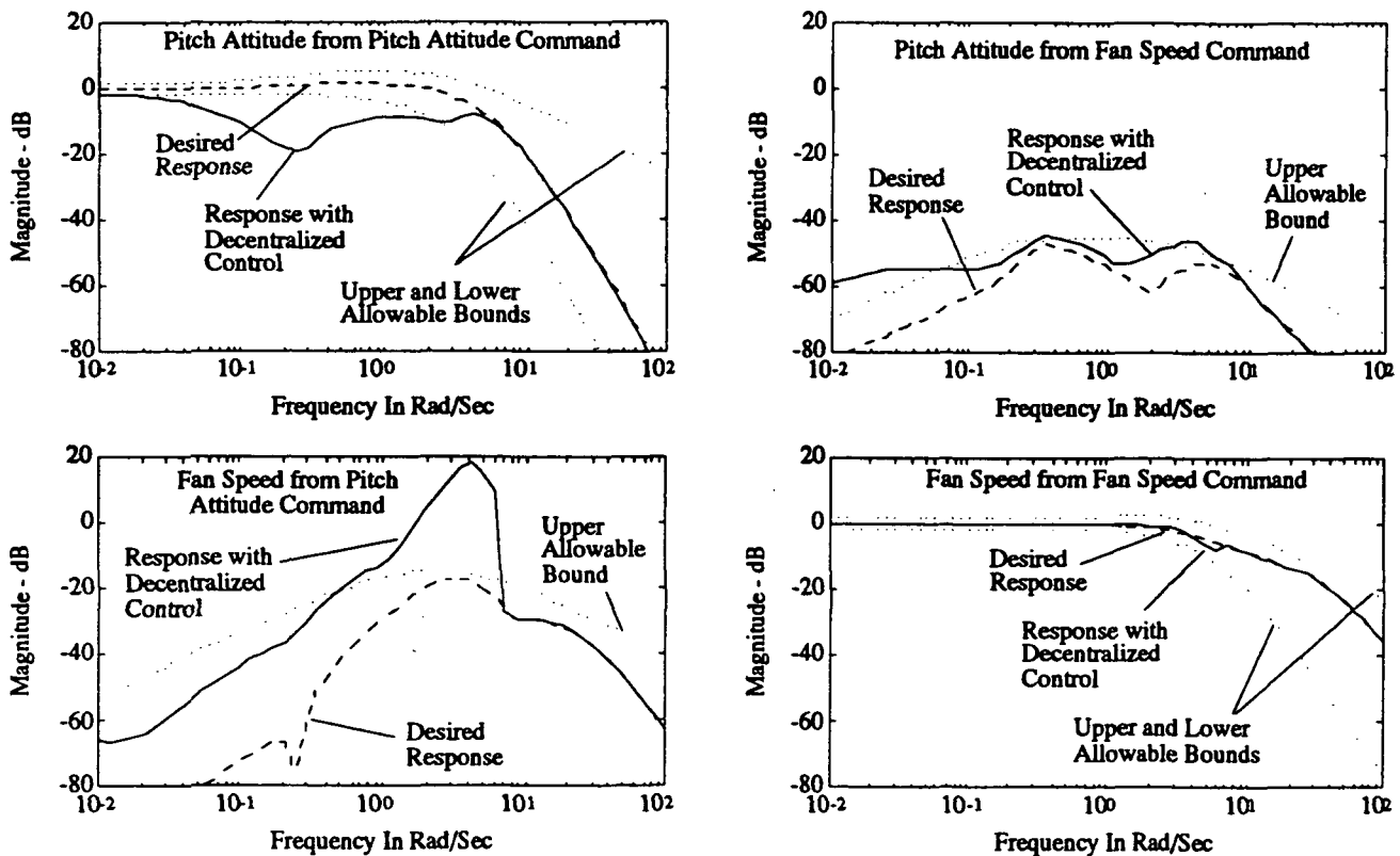
Figure 6 - Closed-Loop Frequency Response Magnitudes - T_A(j\omega) , T_{EA}(j\omega) Unacceptable
