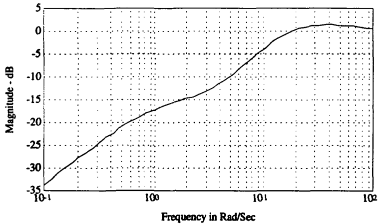
Figure 8.3 - Sensitivity Function of Measured Fan Speed-to-Fan Speed Disturbance (RPM/RPM)
