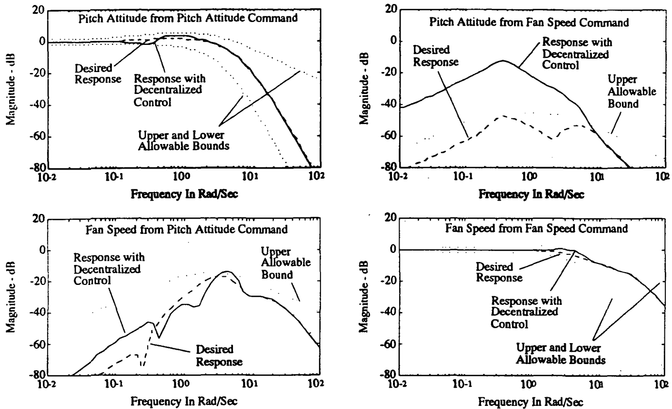
Figure 5 - Closed-Loop Frequency Response Magnitudes - T_{AE}(j\omega) Unacceptable
