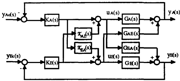
Figure 9 - Fully Interacting Airframe/Engine System
