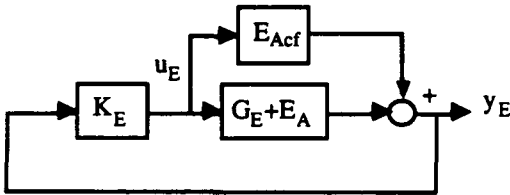
Figure 3 - Engine Loop With All Other Loops Closed
