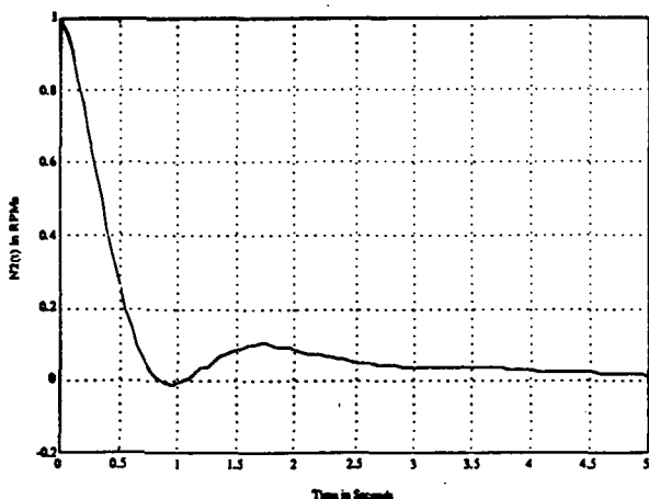
Figure 6 - Measured Fan Speed Unit Step Disturbance Response
