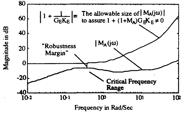
Figure 15 - IS Stability Robustness Criterion
