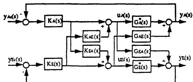
Figure 5.1 - Airframe/Engine System With Control Cross-Feeds
