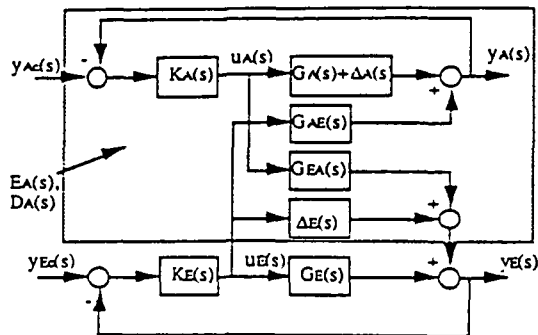
Figure 4.2 - Block Diagram of the Coupled Airframe/Engine System
