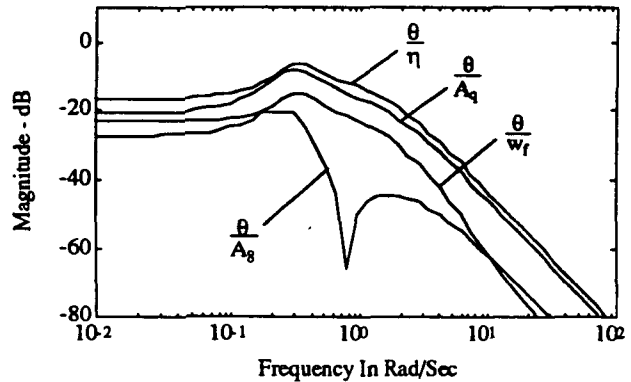
Figure 1 - Pitch Attitude Frequency Response Magnitudes
