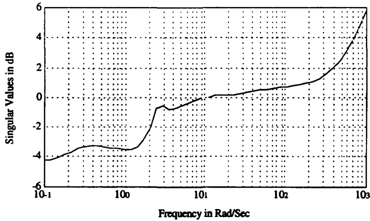
Figure 8.6 - Scaled Multivariable Singular Value Robustness Test q_0/r_0 = 2/3
