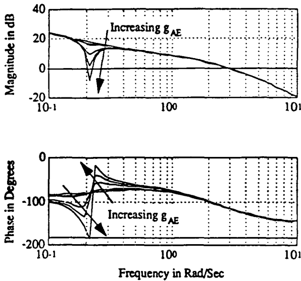
Figure 3.6 - Engine Loop Transfer Frequency Responses of Nominal ( g_E k_E ) and Coupled ( (g_E + e_A)k_E ) Systems
