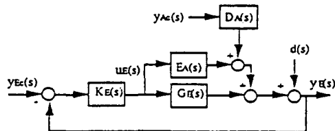
Figure 4.3 - Block Diagram of the Engine Loop for the Coupled Airframe/Engine System
