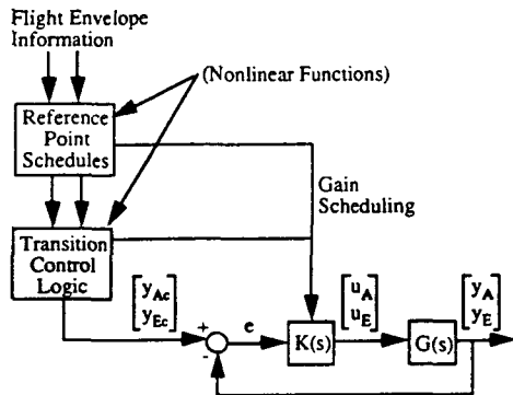
Fig. 3 Full nonlinear airframe/engine system representation.
