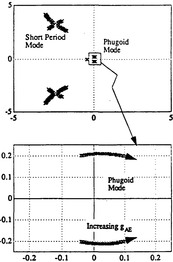
Figure 3.4 - Locus of the Airframe/Engine System's Closed Loop Poles As g_{AE}(s) Is Increased
