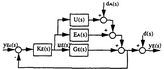
Figure 7 - Engine Loop with Coupling and Model Uncertainty
