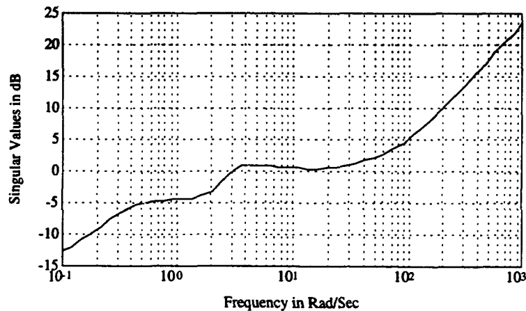
Figure 8.5 - Scaled Multivariable Singular Value Robustness Test q_0/r_0 = 10,000
