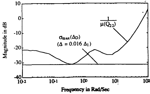
Figure 12 - SSV Stability Robustness Criterion
