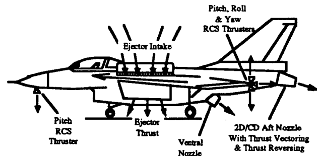
Figure 1 - IFPC Vehicle Configuration
