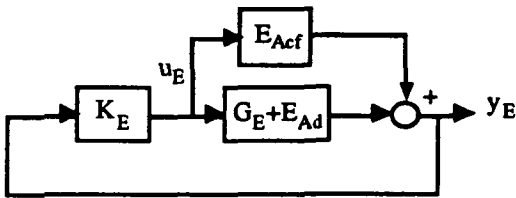
Figure 4 - Engine Loop With All Other Loops Closed
