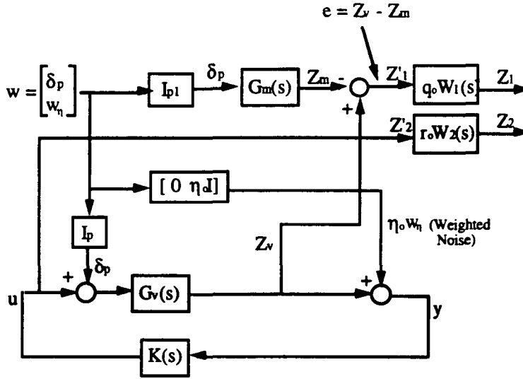
Figure 10.1 - EIMF/ H^\infty Control Design Block Diagram
