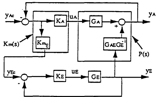
Figure 6.3 - System Framework of Refs. 3 and 6 as it Relates to the Framework of Section 4
