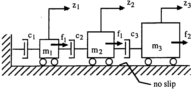
Figure 1 - Academic Example Dynamical System
