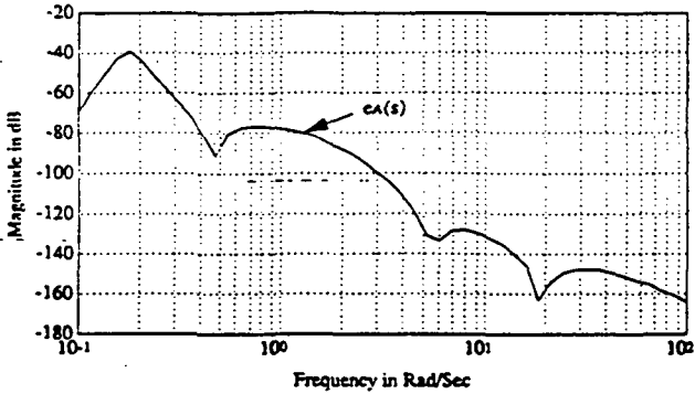
Figure 17 - Magnitude of the e_A(s) Transfer Function
