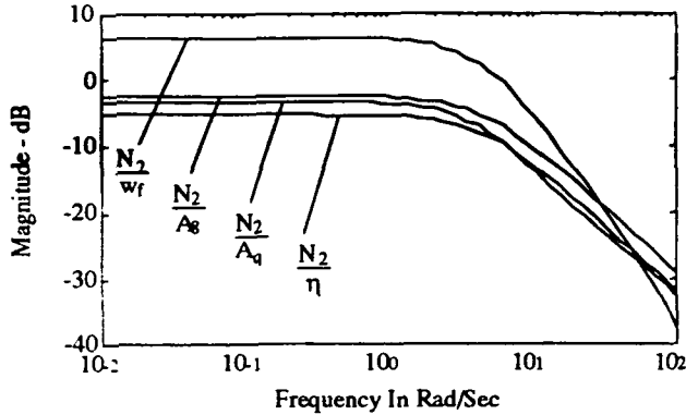
Figure 2 - Fan Speed Frequency Response Magnitudes
