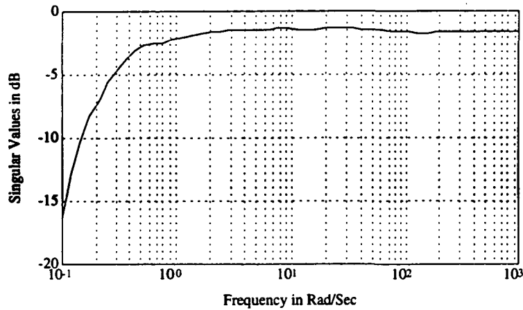
Figure 11.1 - Scaled Multivariable Singular Value Robustness Test q_0/r_0 = 1 \times 10^6
