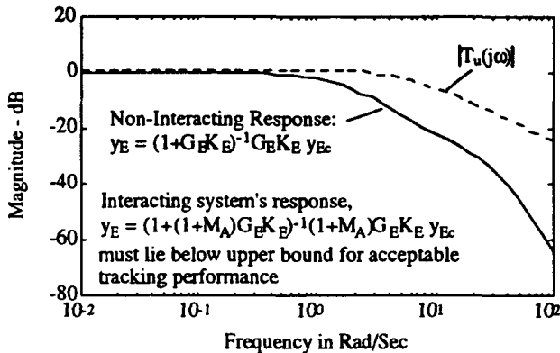
Figure 18 - Non-Interacting Fan Speed Response
