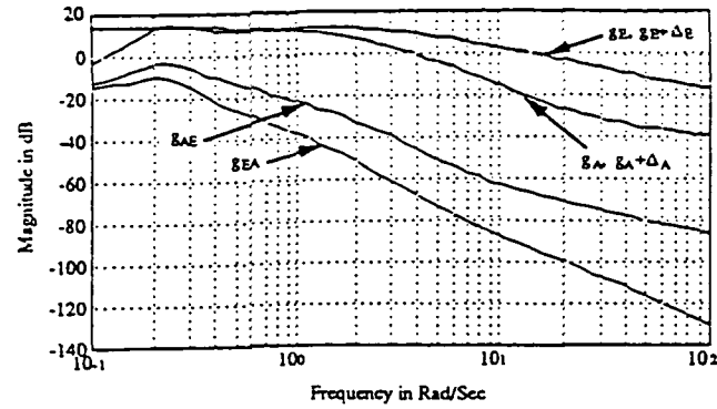
Figure 5.1 - Open Loop Describing Function Magnitudes
