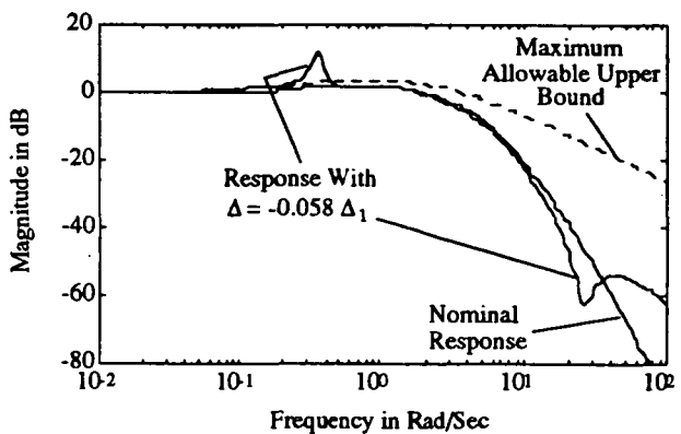
Figure 21 - Pitch Attitude From Pitch Attitude Command
