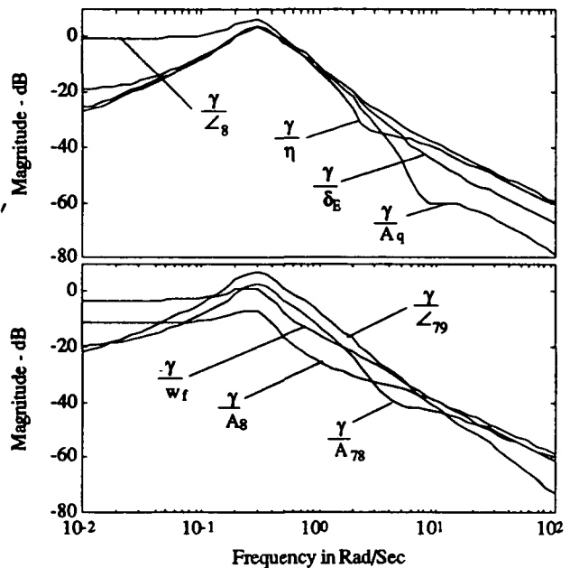
Figure 5 - Flight Path Angle Frequency Response Magnitudes
