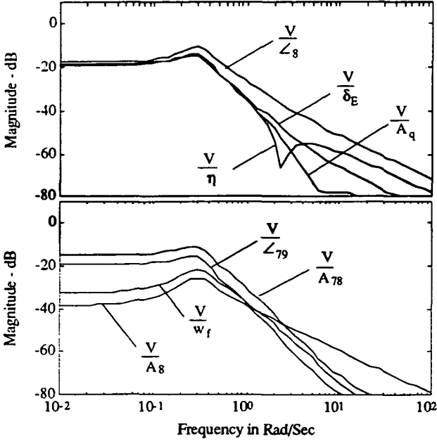
Figure 6 - Forward Velocity Frequency Response Magnitudes
