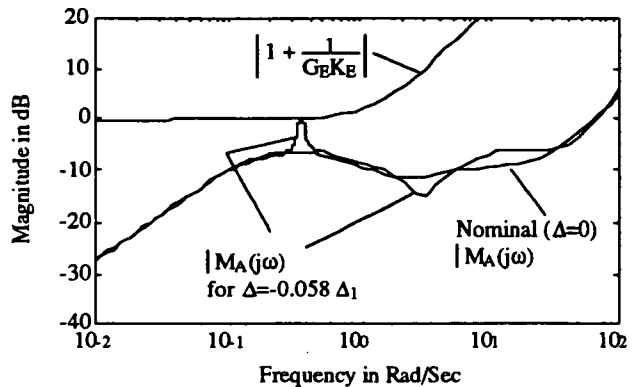
Figure 16 - IS Robustness Criterion With Uncertainty
