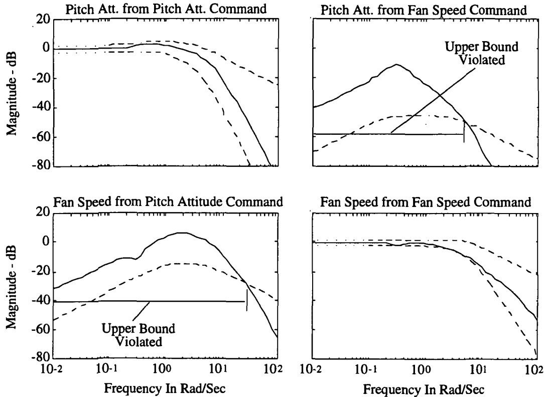
Figure 3 - Closed-Loop Frequency Response Magnitudes - All Elements of T_{AE}(j\omega) and T_{EA}(j\omega) Unacceptably Large For Decentralized Control
