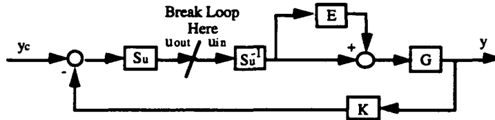
Figure B.1 - Addition of Control Input Scaling to the Loop
