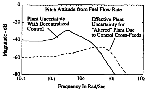
Figure 7 - Effective Plant Uncertainty in Pitch Attitude from Fuel Flow Rate Transfer Function
