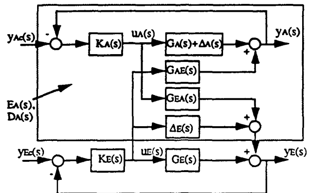
Figure 2.1 - Block Diagram of the Coupled Airframe/Engine System
