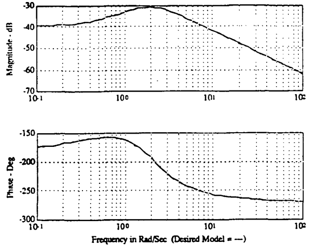
Figure 16 - Closed Loop Pitch Rate-to-Pilot Stick Input Frequency Response
