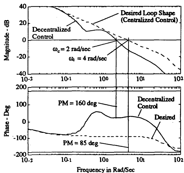
Figure 10 - Engine Loop Transfer Bode Plot With All Other Loops Closed - Centralized and Decentralized
