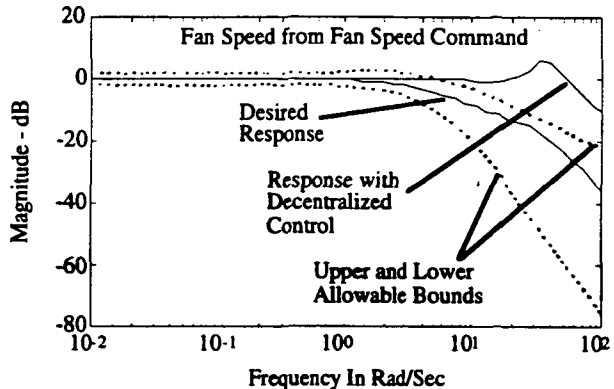
Figure 5 - Closed-Loop Frequency Response Magnitudes - Diagonal Elements of T(j\omega) Unacceptably Large At Higher Frequencies For Decentralized Control
