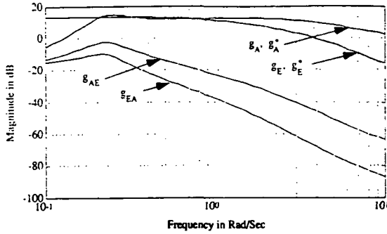
Fig. 8 Open-loop normalized transfer function magnitudes.
