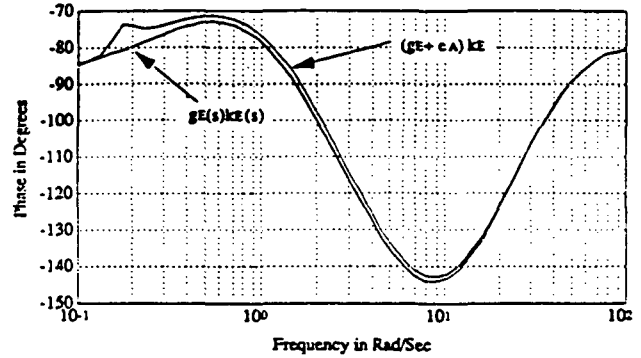
Figure 21 - Open Loop Bode Plot for the Engine Loop
