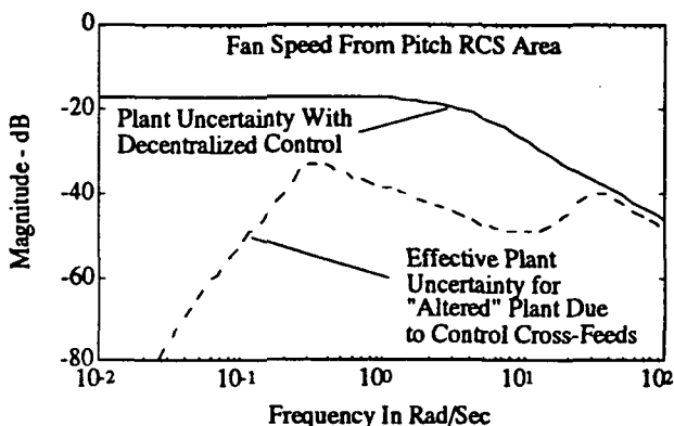
Figure 8 - Effective Plant Uncertainty in Fan Speed from Pitch RCS Area Transfer Function
