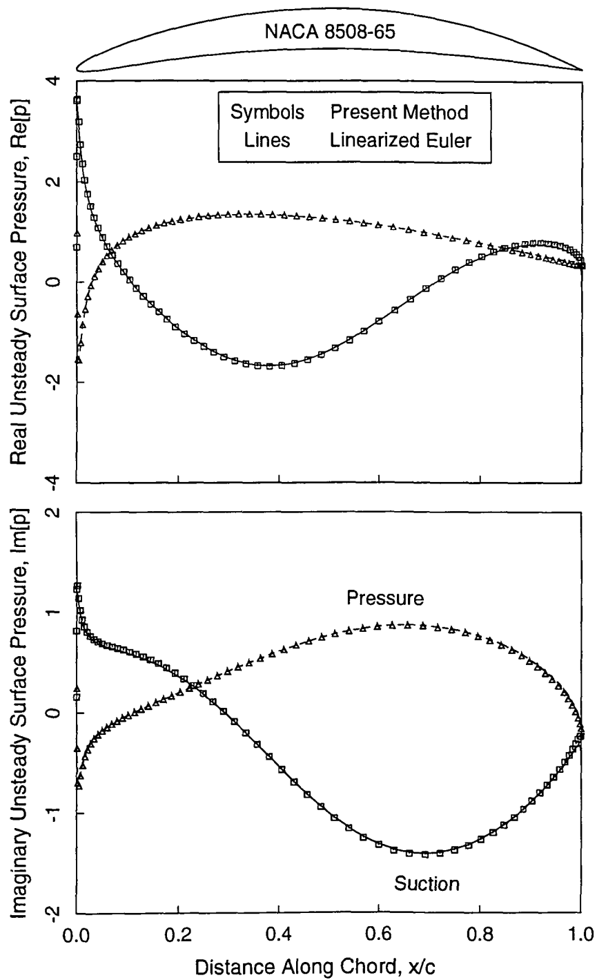
Figure 5.16: Unsteady surface pressure of cascade of NACA 8508-65 airfoils due to incoming vortical gust at 1 \times \text{BPF} . \omega = 3.7687 , \sigma = -144^\circ .
