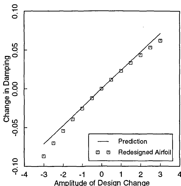
Figure 5.11: Accuracy of sensitivity analysis for various perturbation amplitudes.
