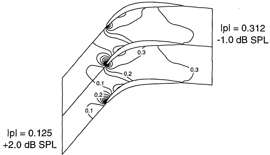
Figure 5.30: Contours of magnitude of unsteady pressure for radial station near the hub of a redesigned modern fan exit guide vane due to incoming vortical gust at 2 \times \text{BPF} . M_\infty = 0.32 , G = 0.46 , \omega = 12.5 , \sigma = -288^\circ .
