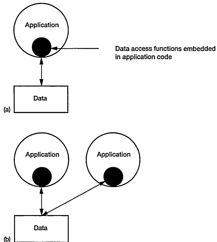
Figure 8.—Embedded data access functions in (a) single and (b) multiple applications allow free (uncoordinated) access to data.
