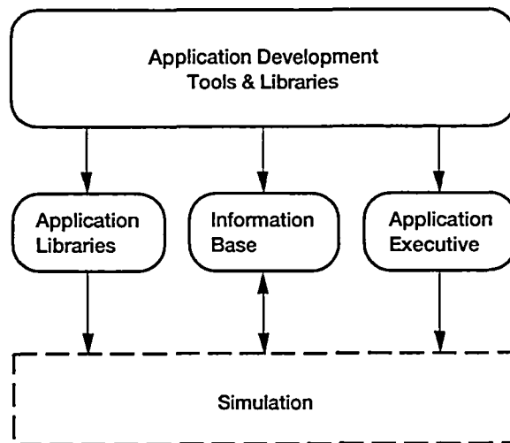
Figure 1.—The OSSM model.
