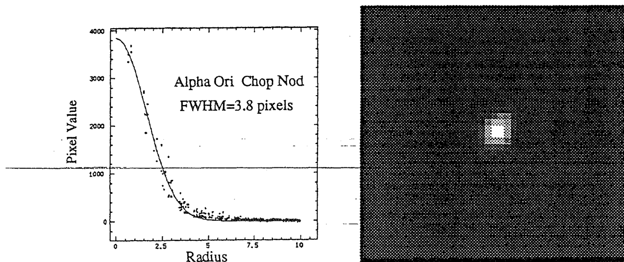
Figure 3. KAO stellar profiles of Alpha Ori. On the left is a profile taken on 4/1/94 at 6.2\mu\text{m} in a chop and nod sequence of four integrations, + - - + with the camera. On the right is a 64 \times 64 section of the chip from which the profile is taken. The 6.2\mu\text{m} profile has a FWHM of 6.1 arcsec. This image size is mostly a measure of the tracker chop-nod stability of our flight.
