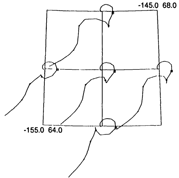
Figure 10. Wind hodographs from the model at 1400 and 1500 UT. The curves at four positions surrounding the observations are shown.
