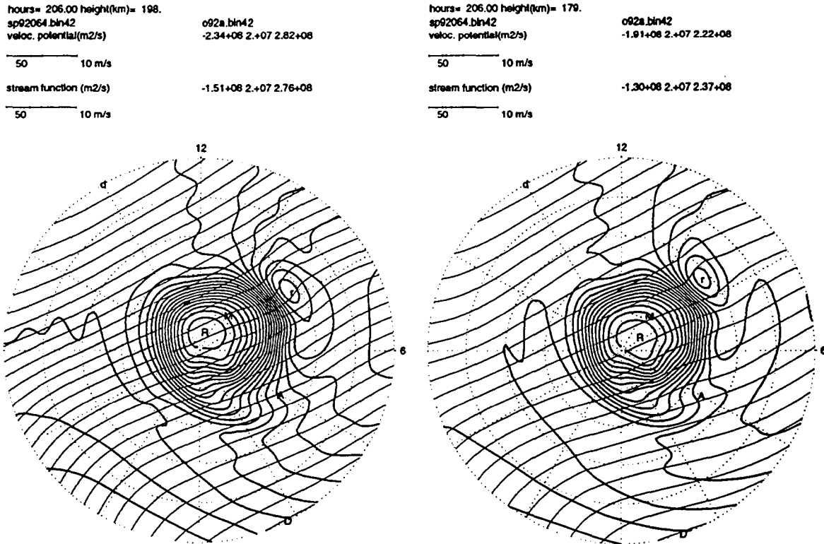
Figure 7. Stream function and velocity potentials from the spectral thermospheric general circulation model simulations for heights of 198 and 179 km at the time of the chemical release wind measurements. The flow velocities increase with decreasing separation between the contours. Velocity scales appear at the top.
