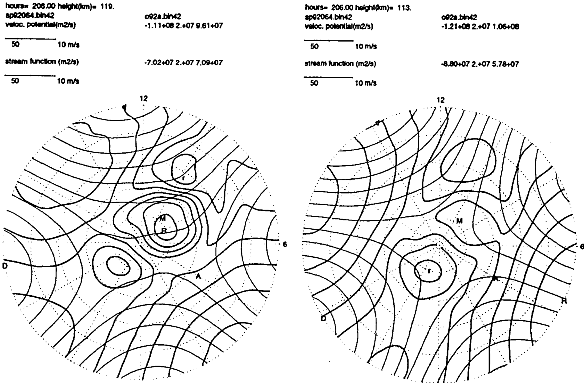
Figure 8. Similar to Figure 7 but for heights of 119 and 113 km.
