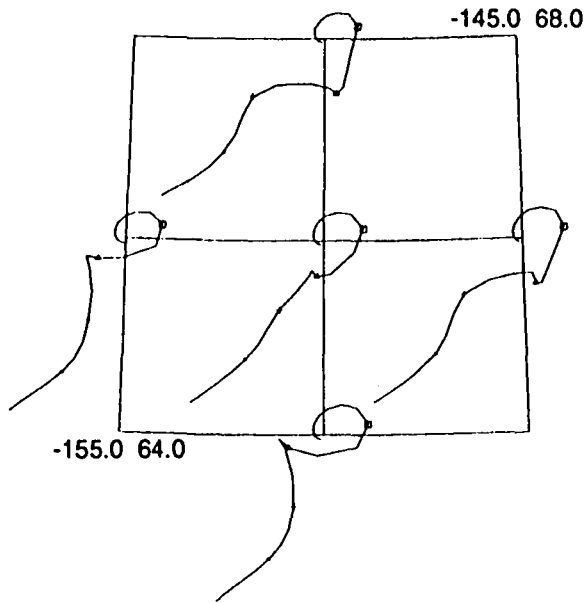
Figure 10. Wind hodographs from the model at 1400 and 1500 UT. The curves at four positions surrounding the observations are shown.
