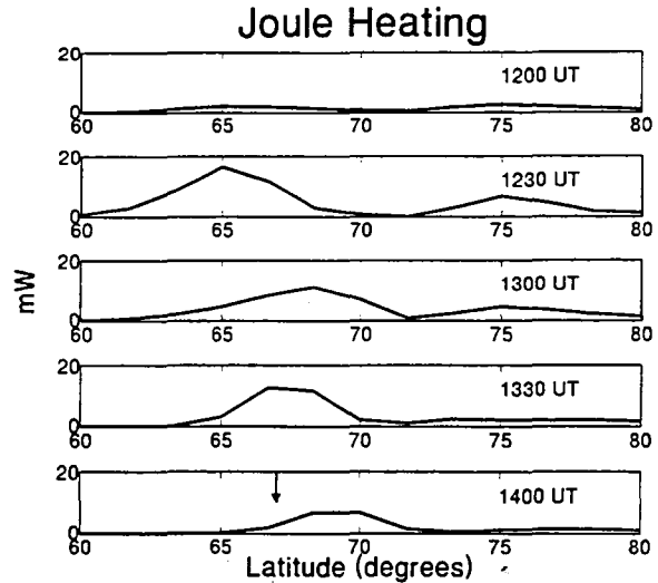
Figure 3. Joule heating in a format similar to that used in Figure 2. The values were obtained from the assimilated mapping of ionospheric electrodynamics (AMIE) analysis.
