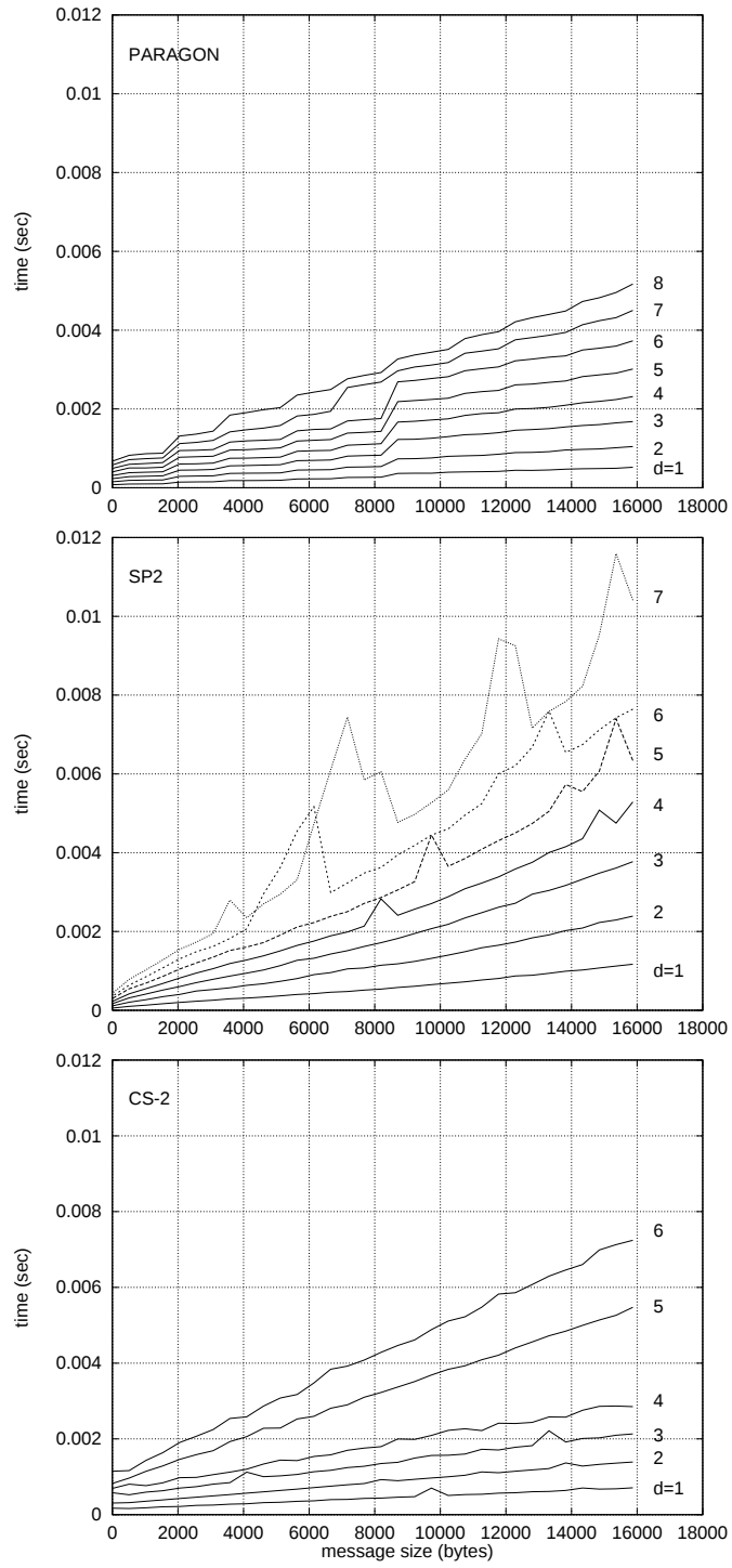
Figure 3: Hypercube emulation.
