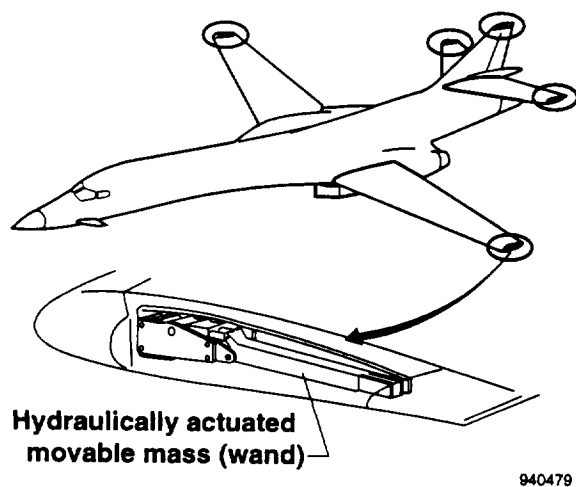
Figure 5. Inertial excitation system (ref. 23).
