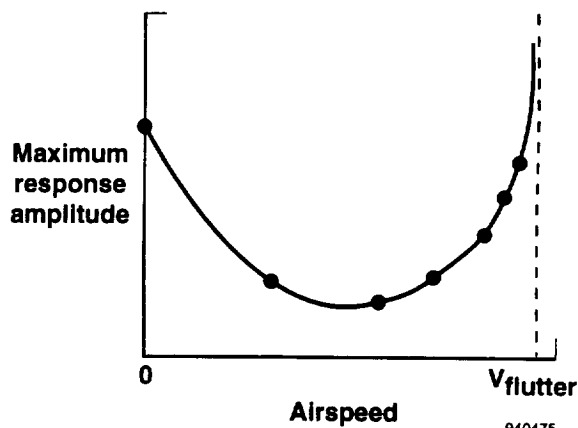
Figure 1. Von Schlippe's flight flutter test method.
